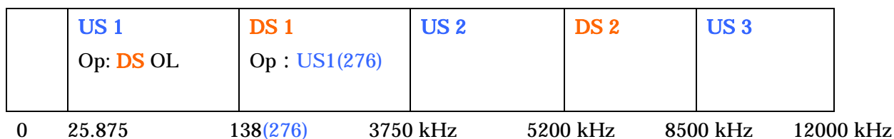
Fig.1 Band Plan for ADSL
