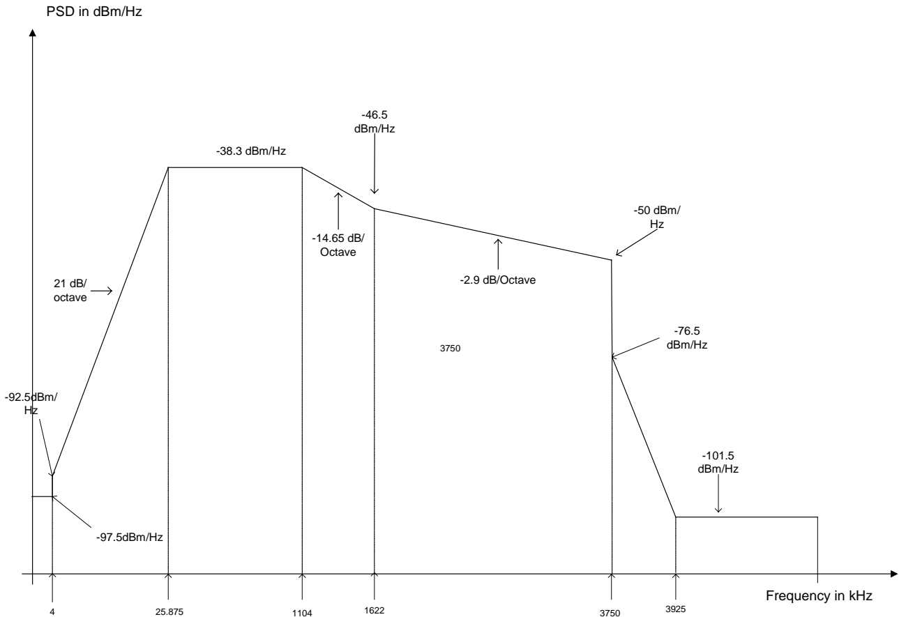
Figure 1. OL Quad Spectrum Mask Plot, Peak Values
