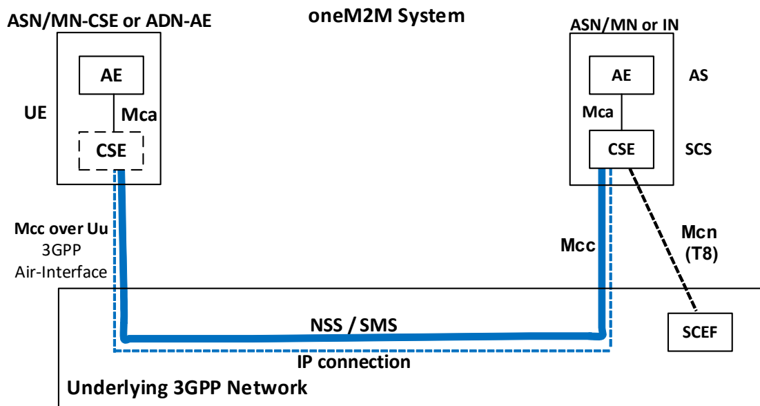
Figure 6.1-1: Connectivity Establishment between ASN/MN-CSE or ADN-AE and CSE (SCS)
