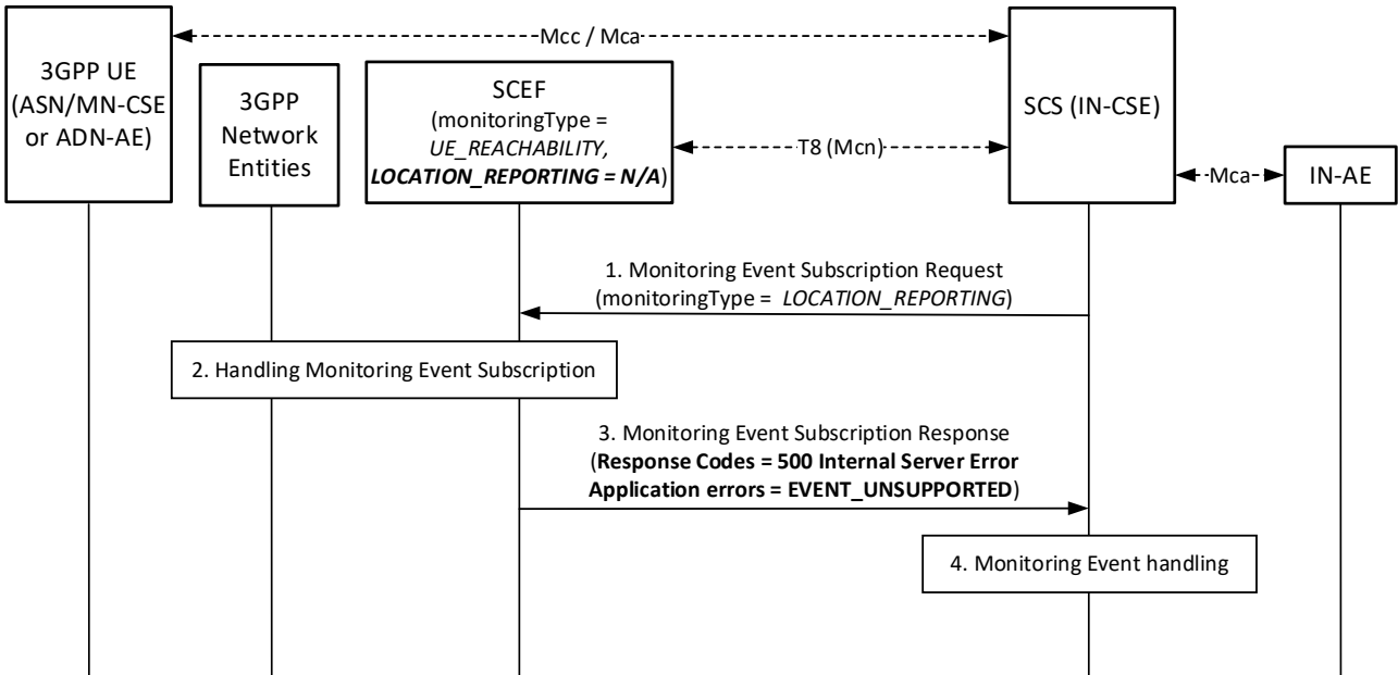
Figure 8.3.2.1-1: Error handling procedures for Location Reporting of Monitoring events
