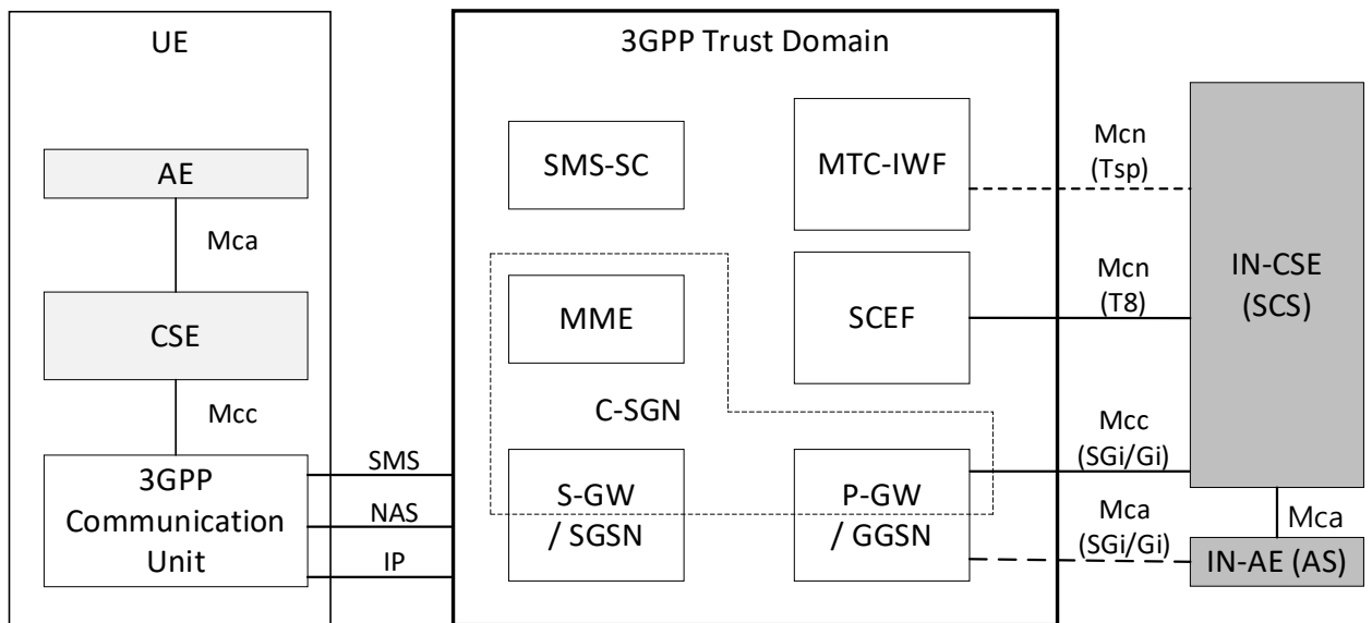
Optionally present oneM2M entity oneM2M entity - - - - - Direct connection option not currently supported - - - - - Tsp is not focus at this TS
