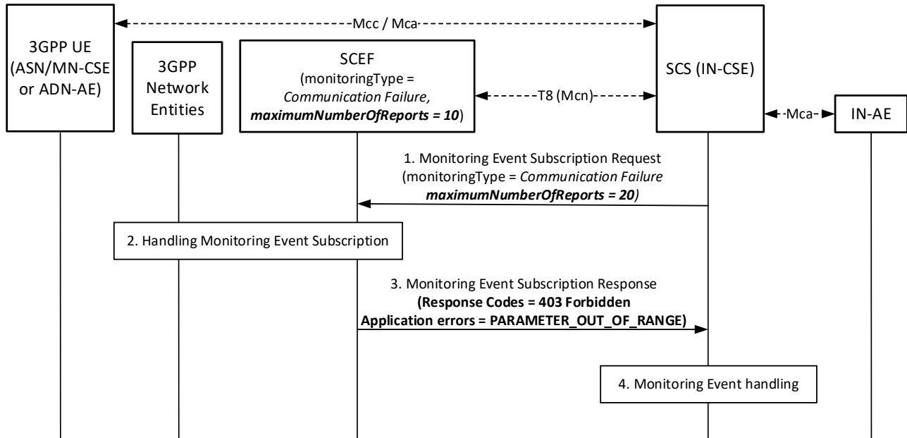
Figure 8.3.2.2-1: Error handling procedures for Communication Failure of Monitoring events
