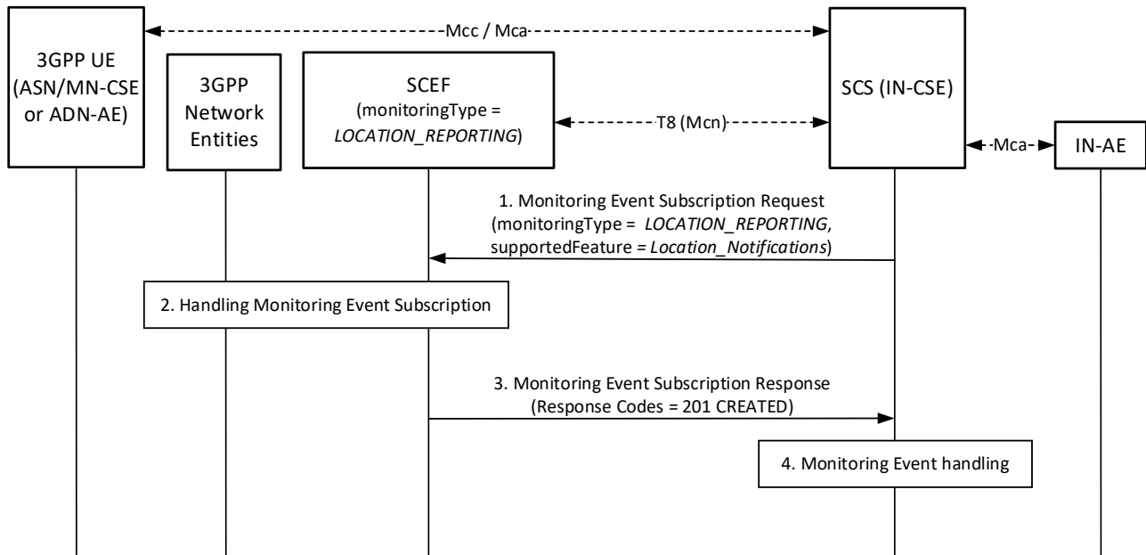
Figure 7.14.2-1: Normal procedures for a supportedFeatures
