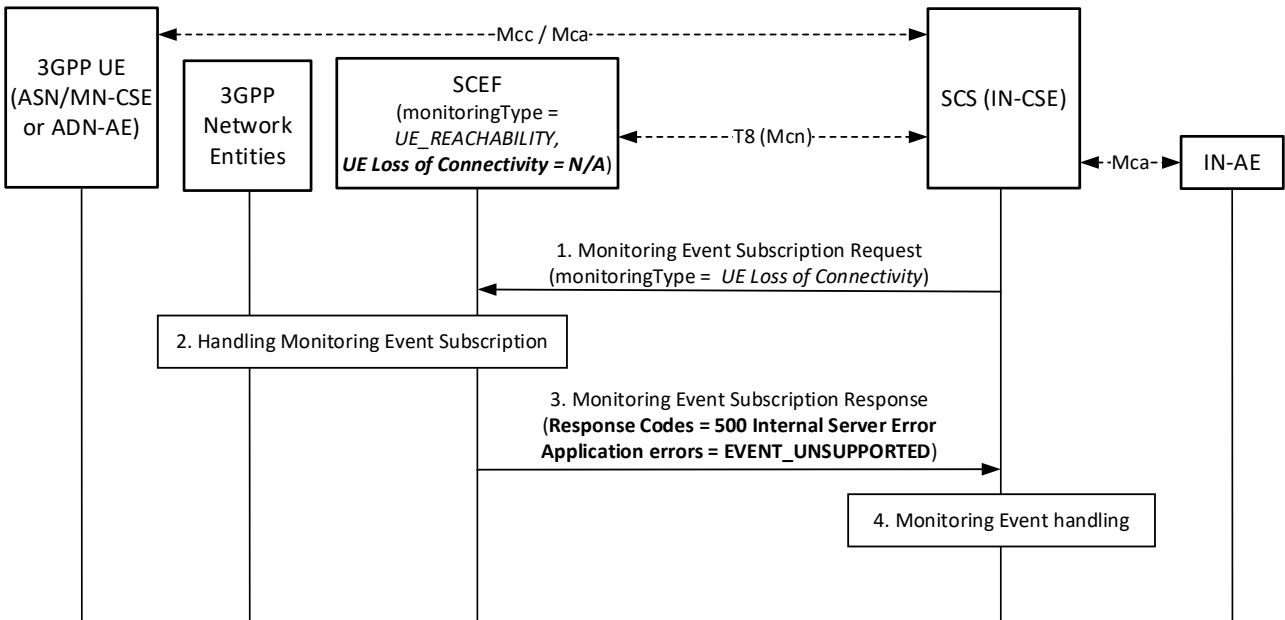
Figure 8.3.2.1-2: Error handling procedures for UE Loss of Connectivity of Monitoring events
