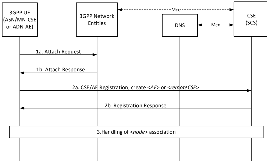
Figure 6.3-1 UE Attach Procedure with oneM2M Registration
