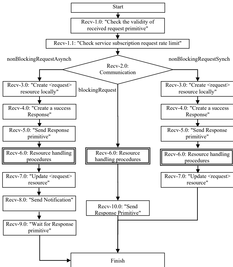
Figure 7.2.2.2-1: Generic procedure of Receiver
