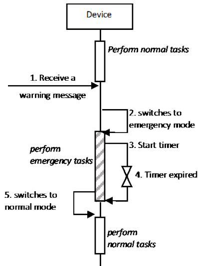
Figure 6.4.7-1: Alternative flow on triggering by a timer
