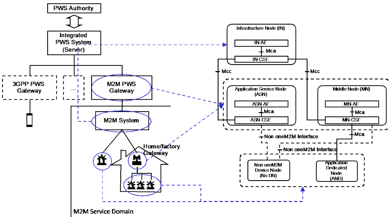
Figure 7.2-1: High Level Architecture for IoT PWS Service
