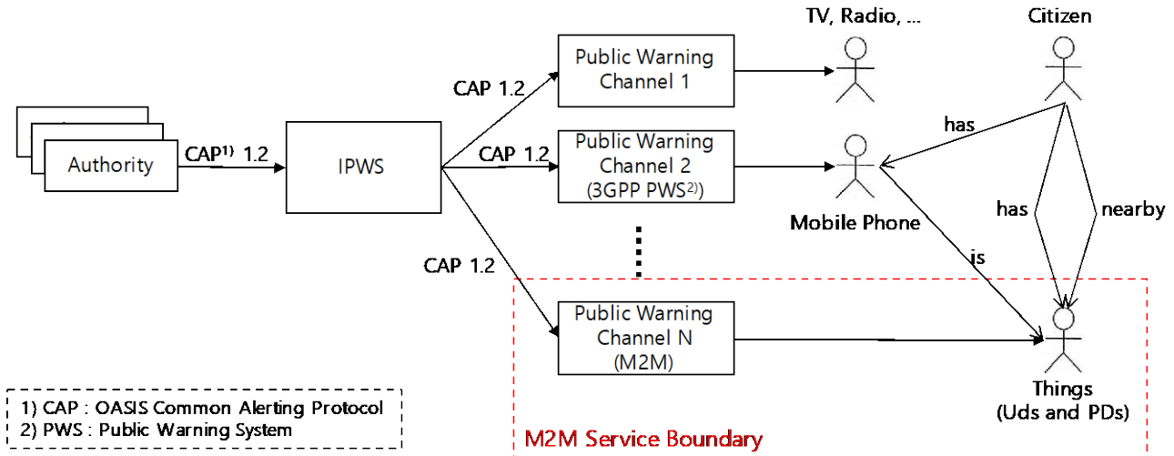
Figure 6.1.9-1: High level system view
