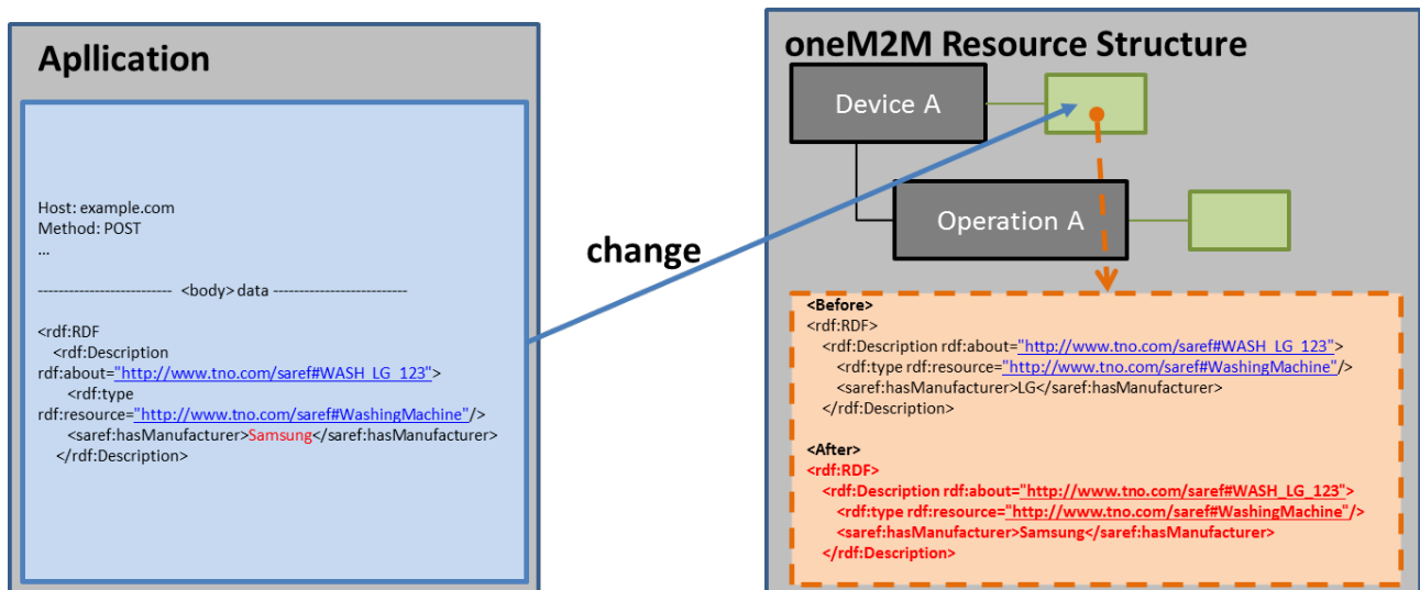
Figure 8.2.2.2-1: Concrete example of managing semantic instance in the oneM2M system
