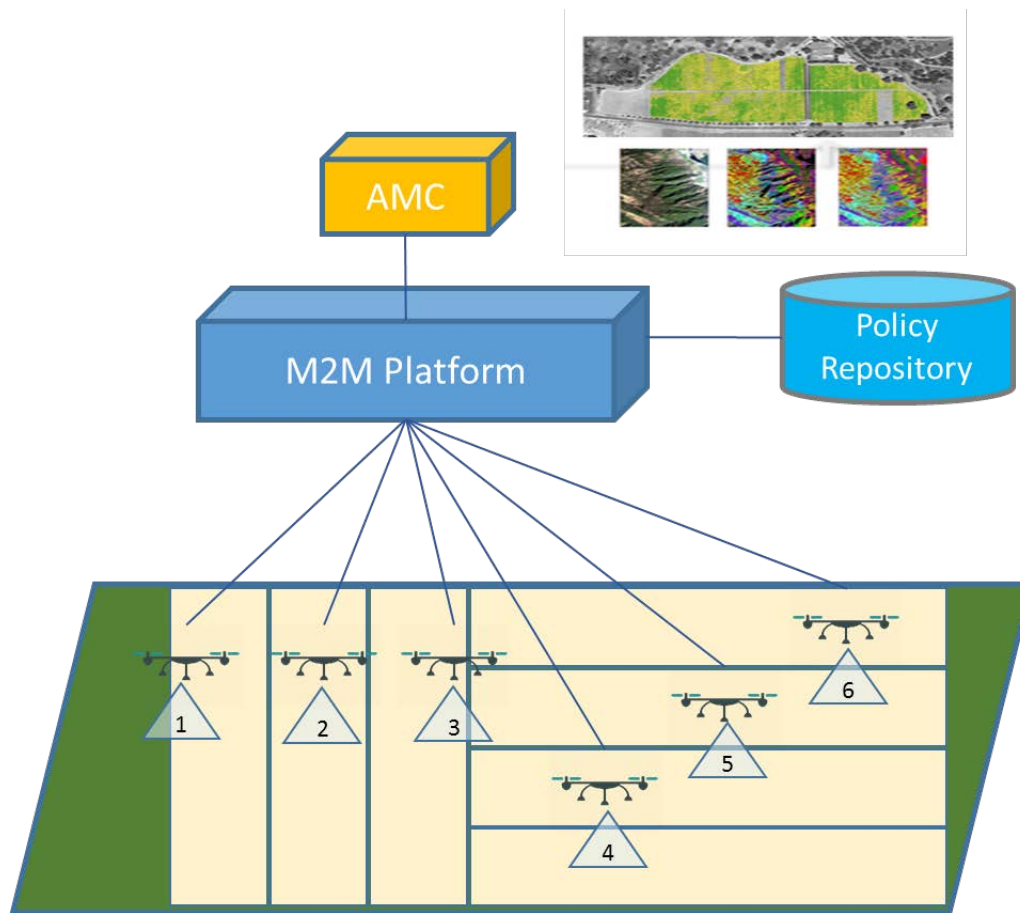
Figure 12-29 Agriculture monitoring drone system
