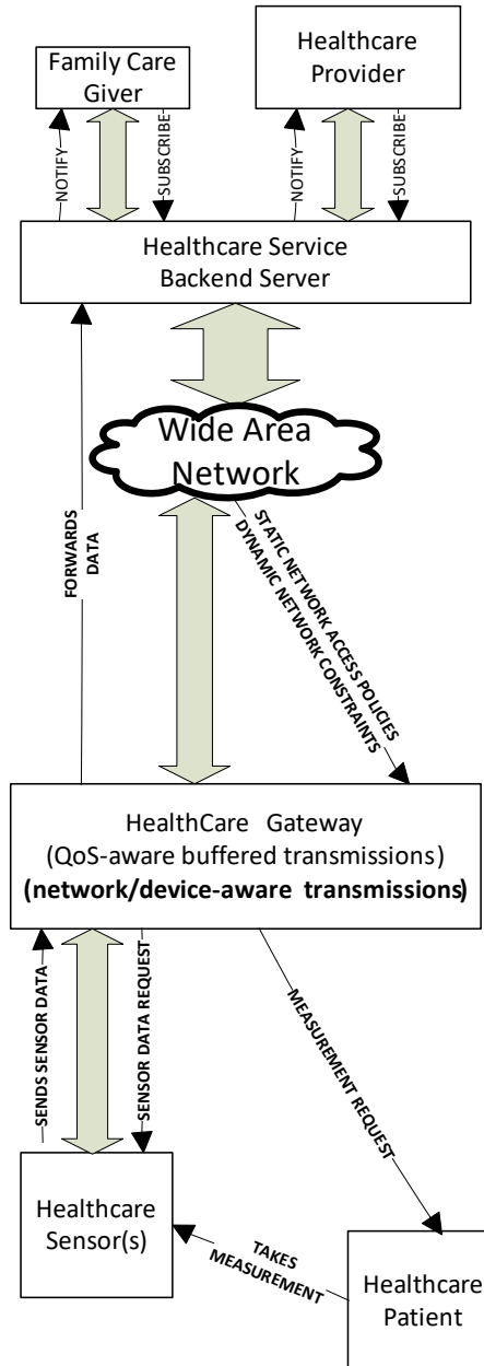
Figure 7-2 Network/Device-aware Flow
