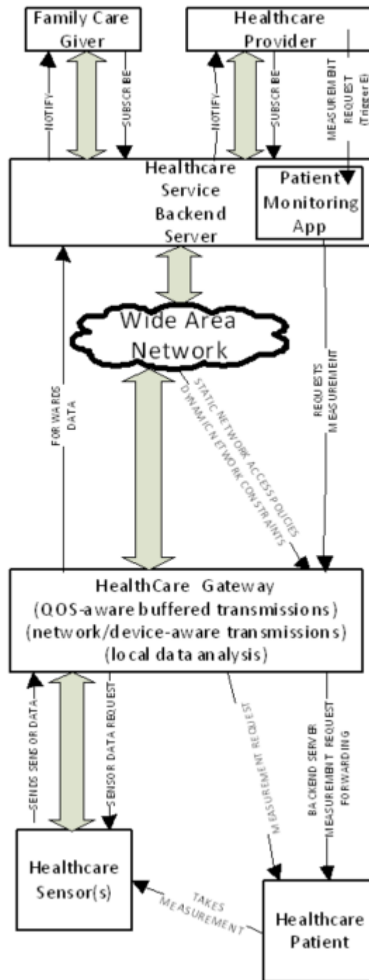
Figure 7-1 Healthcare Measurement Data Processing Flow
