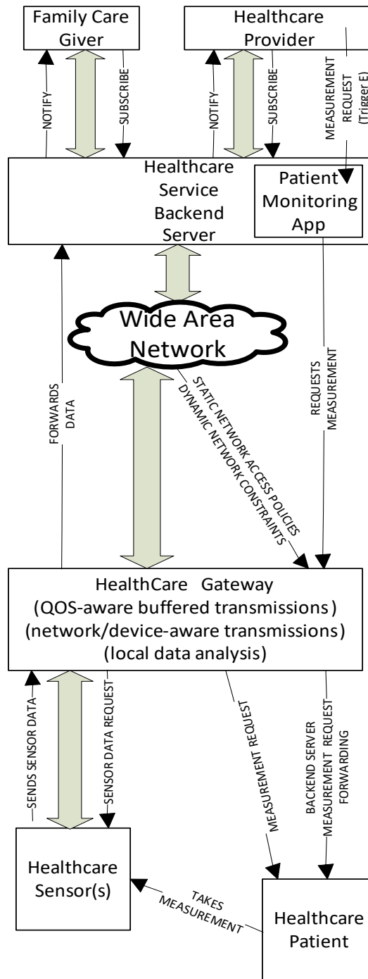
993 994 Figure 7-6 Healthcare Gateway High Level Illustration
