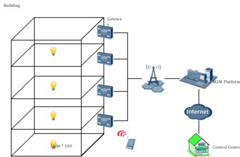
737 738 Figure 6-1 Smart Building Scenario
