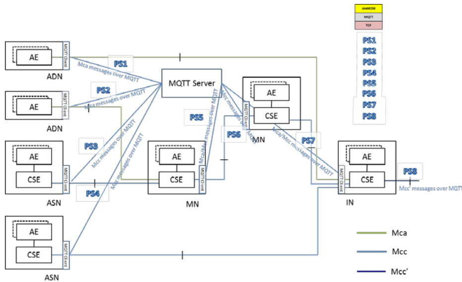
Figure 5.2.2.2-1: MQTT server independently located scenario
