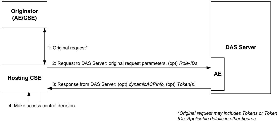
Figure 7.3.2.1-2: Direct Dynamic Authorization
