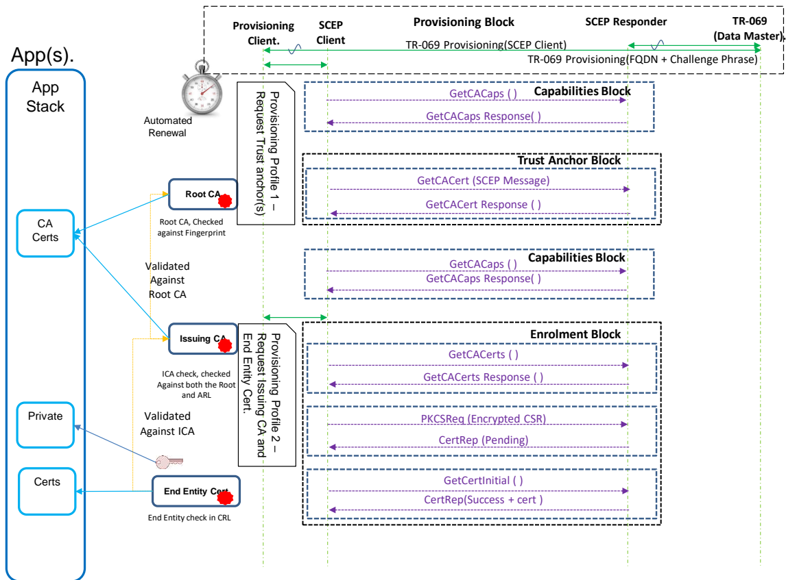
Figure L. 1: SCEP certificate provisioning procedure
