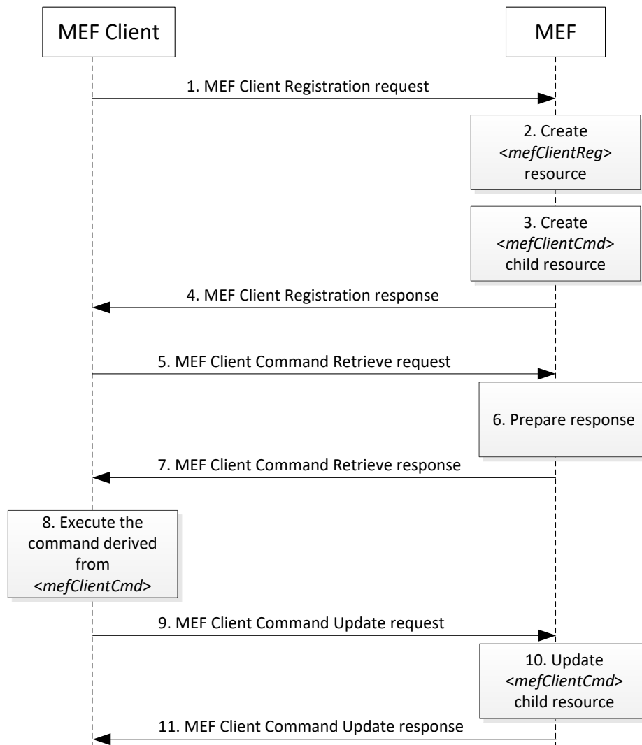
Figure 8.3.4.6-1: Example MEF Client Command procedure
