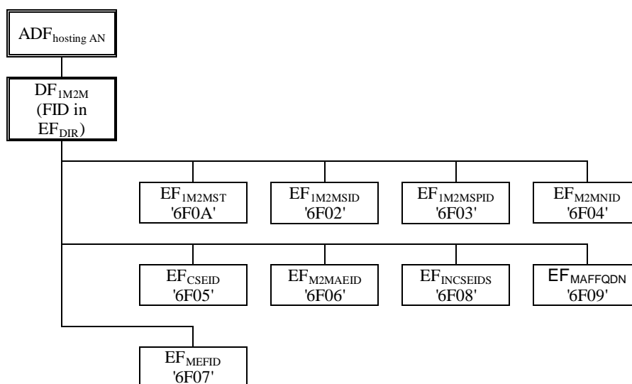
Figure D.1: File identifiers and directory structures of DF_{1M2M} in an hosting Access Network application ADF
