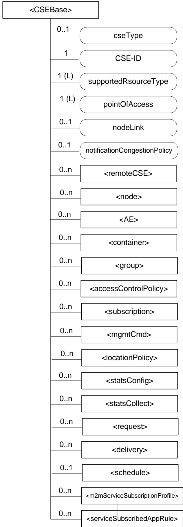
Figure 9.6.3-1: Structure of <CSEBase> resource
