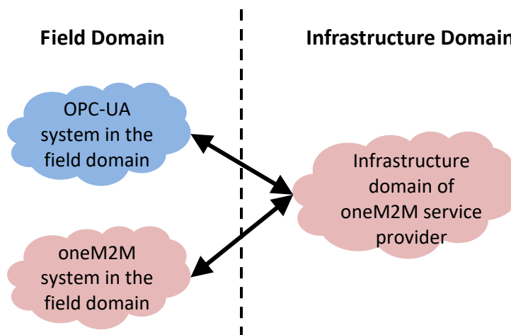
Figure 10.2.4-1: OPC-UA and oneM2M system in the field domain interact with each other via oneM2M infrastructure domain
