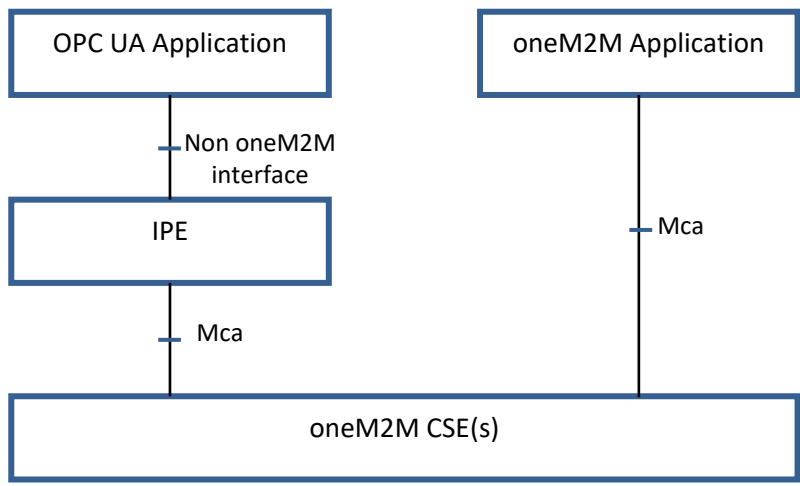
Figure 10.3.2-1: Functional Architecture with IPE
