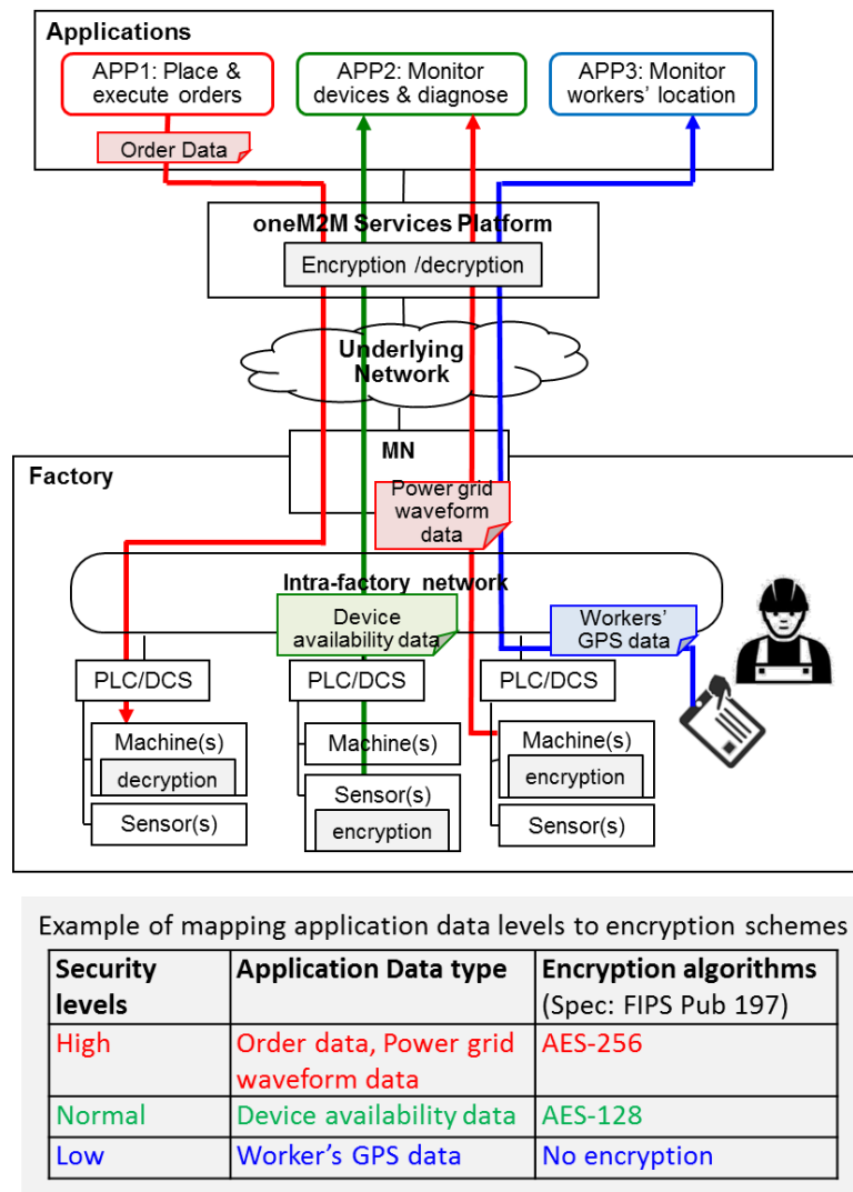
Figure 6.6.7-1: High-level Illustration of Real Time Data Collection
