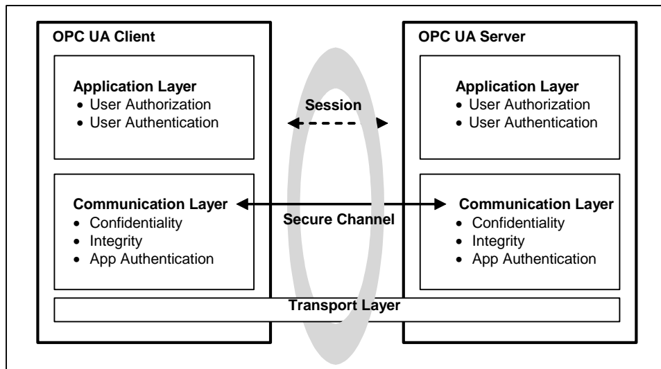
Figure 10.1.5-2: OPC-UA security architecture
