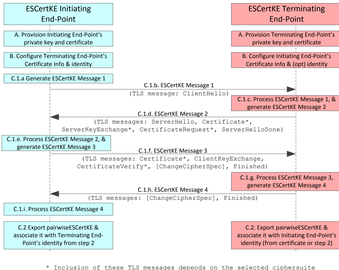
Figure 8.4.2-1: ESCertKE Procedure message flow
