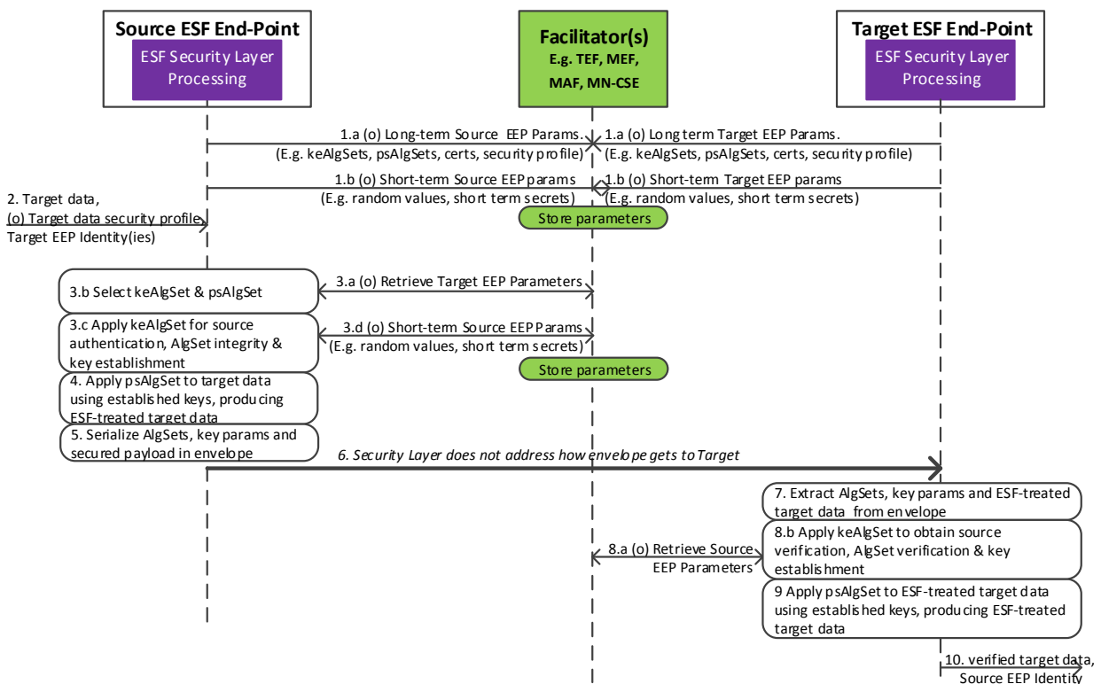
Figure 6.2.2.3-1 Processing flow for single envelope session type (S1).
