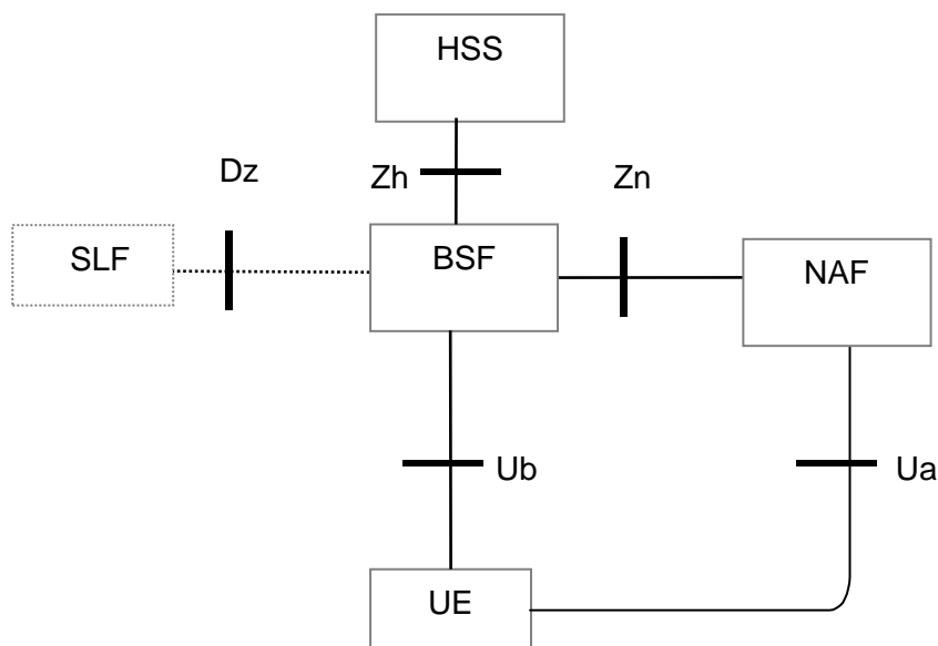
Figure 11.1-1: Simple Network Architecture for GBA in ETSI TS 133 220 [i.10]
