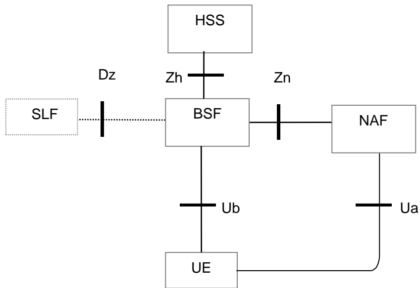
Figure 5-a: Simple Network Architecture for GBA in ETSI TS 133 220 [i.10]
