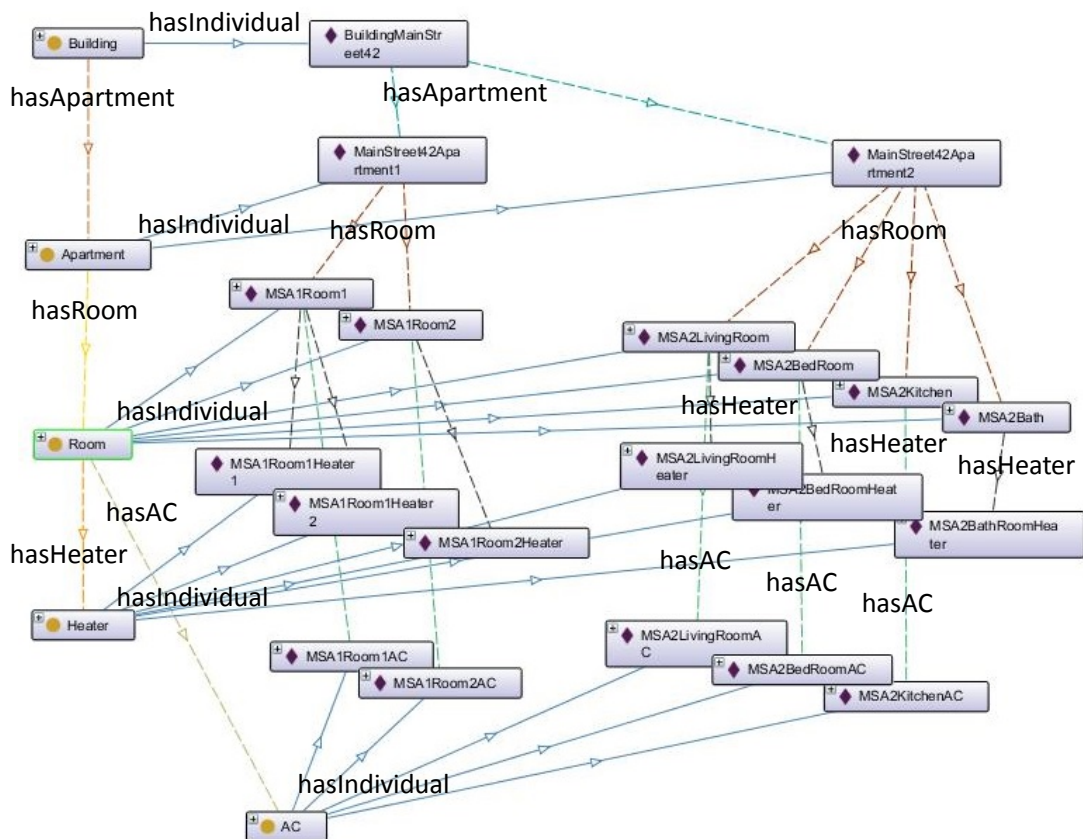
Figure A.6: Ontology model with instances
