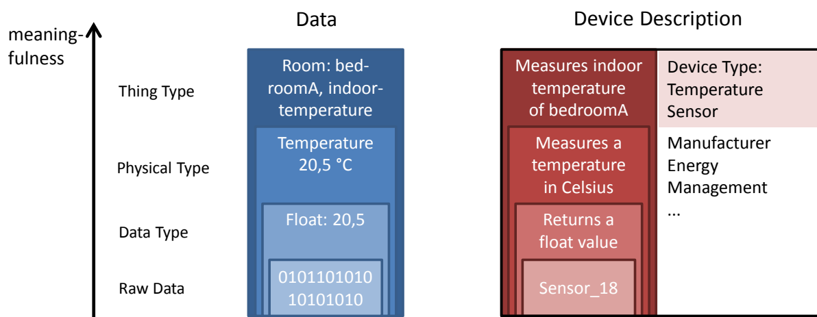
Figure 2: Levels of meaningfulness
