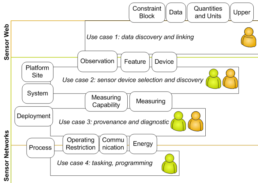
Figure 24: Use cases and ontology modules
