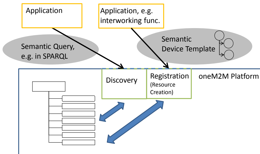
Figure 37: Use of Semantic Technologies for Platform Functionalities
