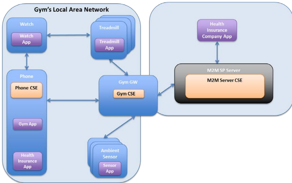
Figure A.8: Gym Use Case Architecture
