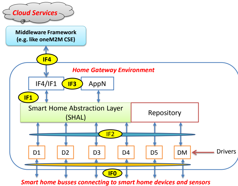
Figure 9: A high-level conceptual HGI architecture
