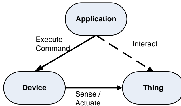
Figure 25: Domain Model
