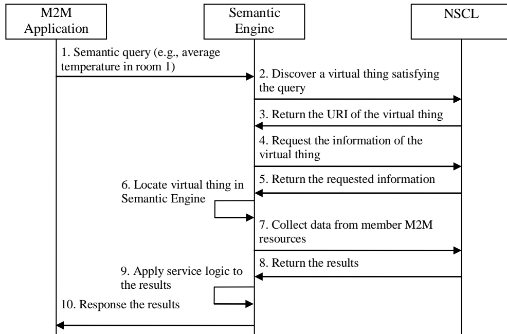
Figure 14: Semantic virtual mashup procedure
