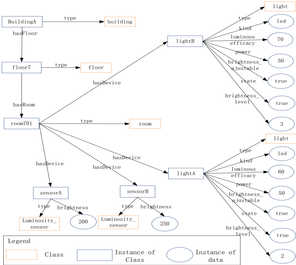
Figure A.25: Example of instances
