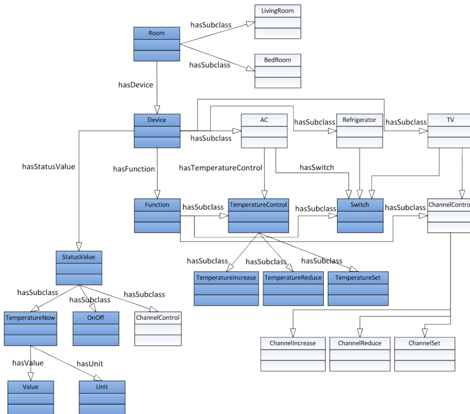
Figure A.19: Home Automation Ontology Model
