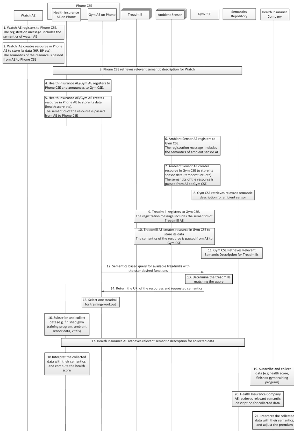
Figure A.12: Normal Flow
