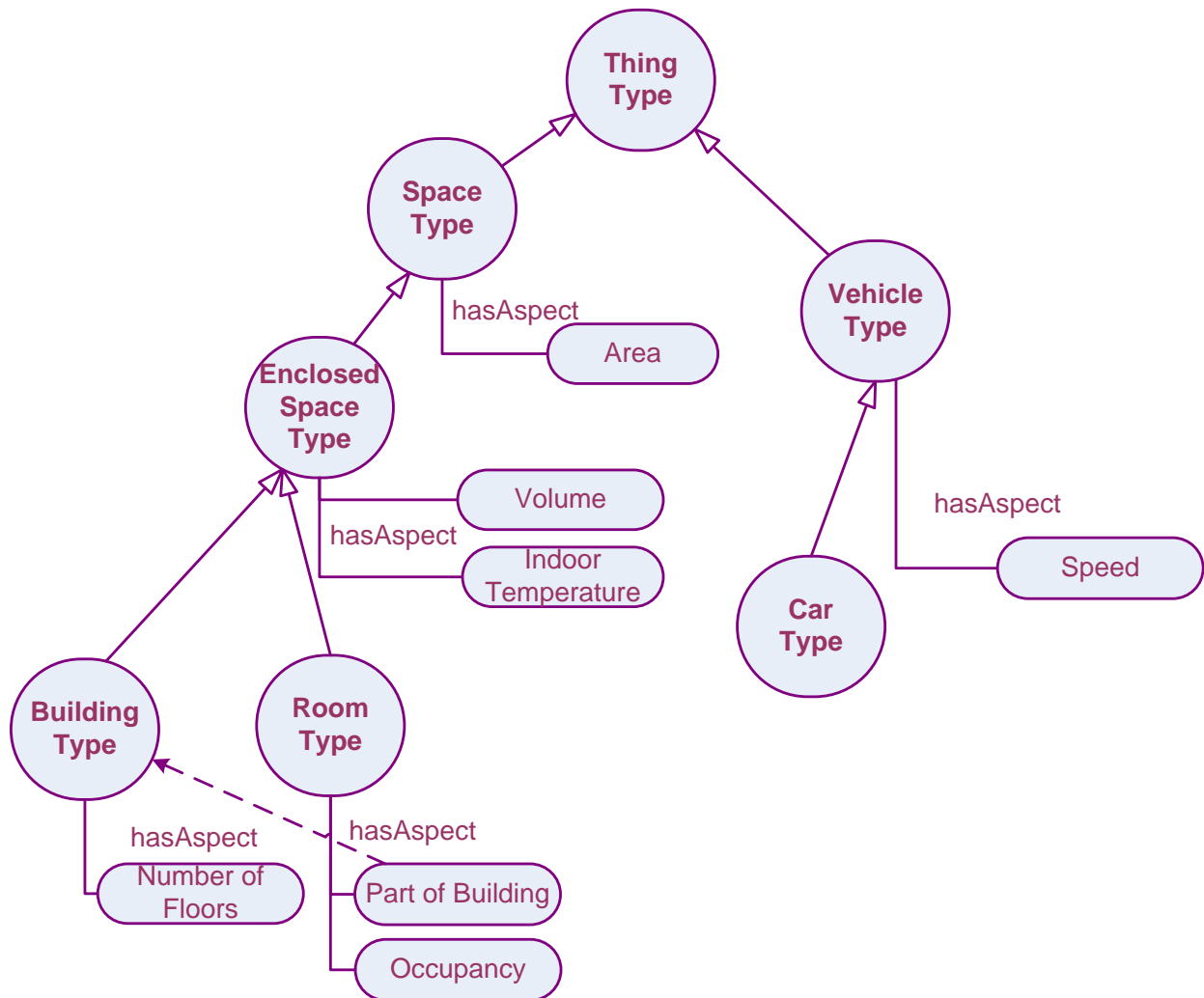
Figure 30: Example of Thing Type Hierarchy
