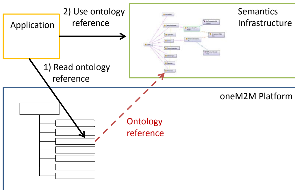
Figure 36: Semantic Annotations
