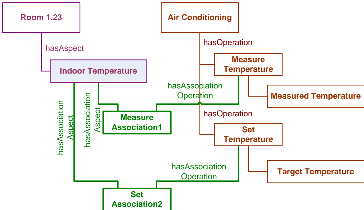
Figure 34: Association Example
