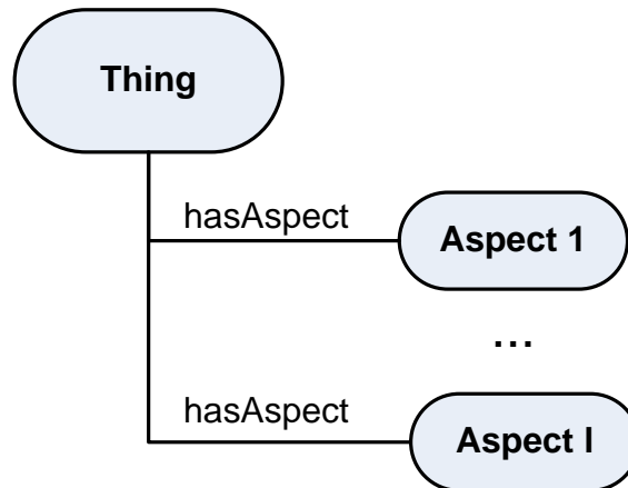
Figure 27: Thing Structure
