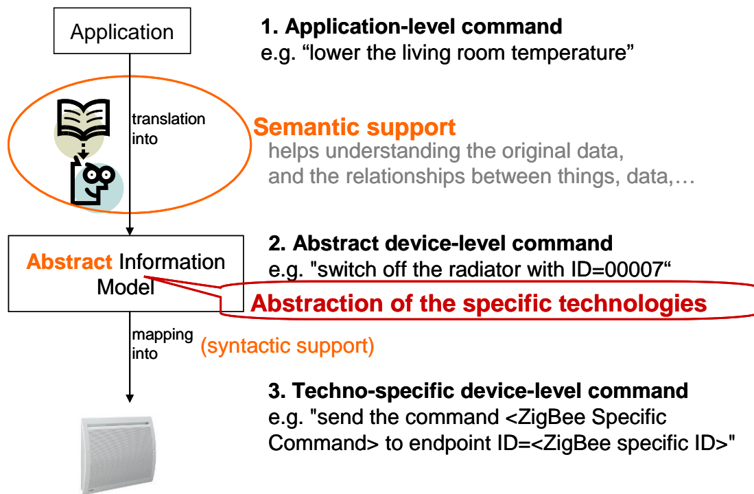
Figure 1: Abstraction versus Semantic for oneM2M
