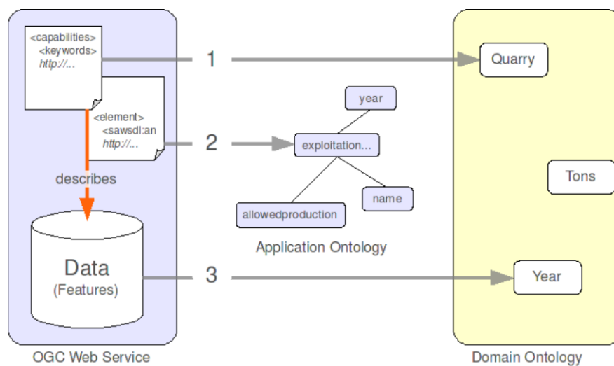
Figure 16: Semantic annotations at three different levels
