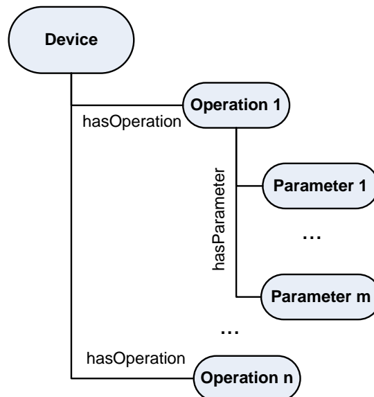
Figure 26: Device Structure
