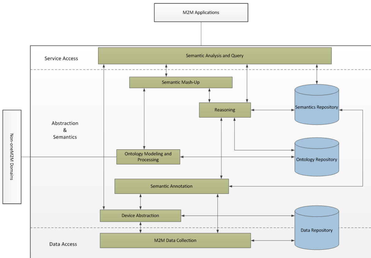
Figure 11: Generic functional model for supporting semantics
