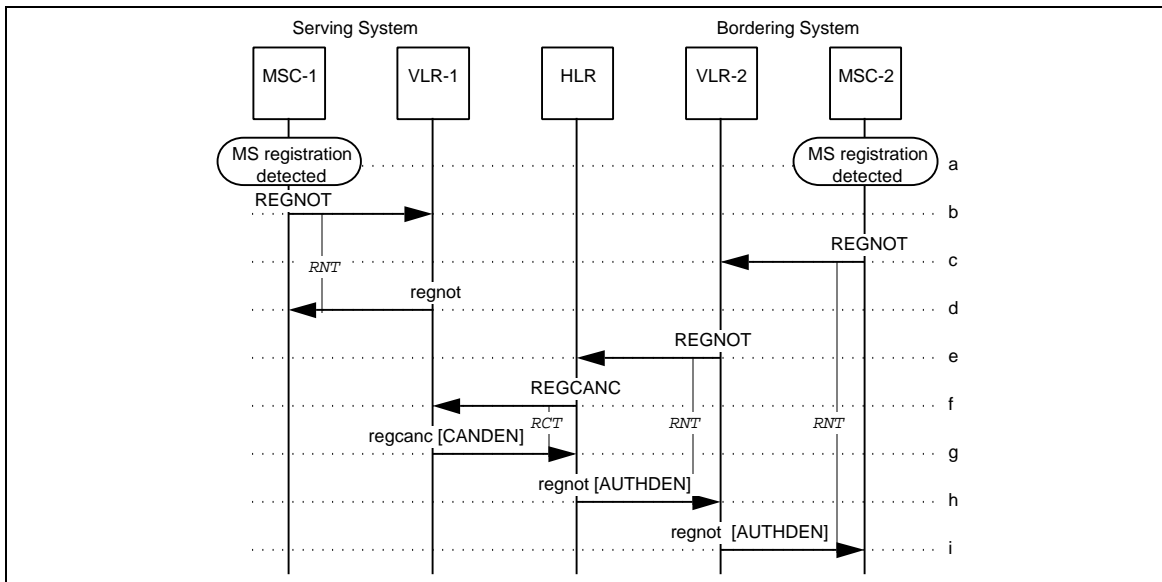
Figure 88 Multiple Registrations with Cancellation Denied at the VLR
