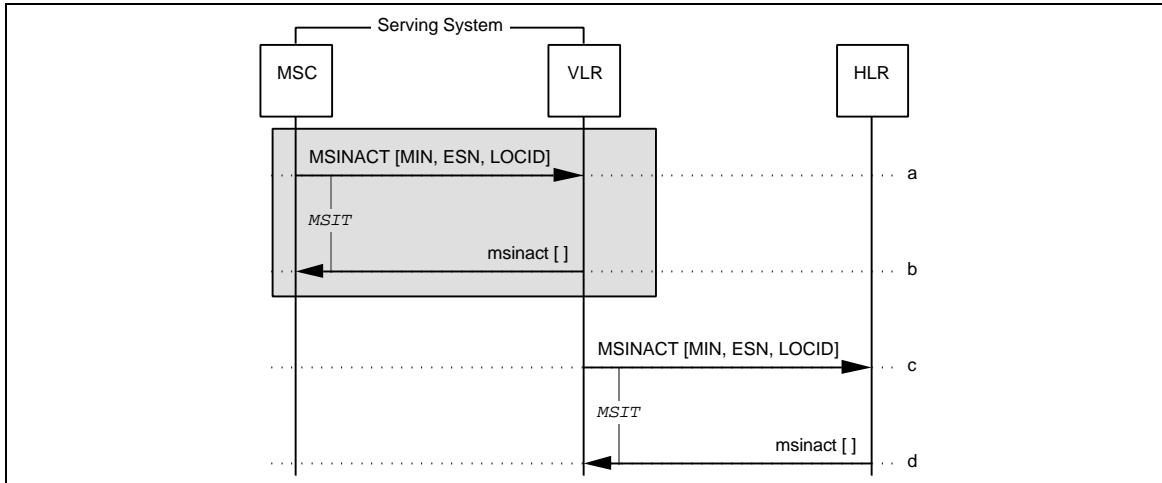
Figure 43 Successful MSInactive: MS Declared Inactive
