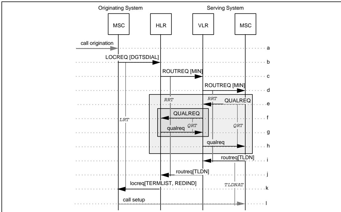
Figure 114 CD Invocation to an Idle MS on Another MSC
