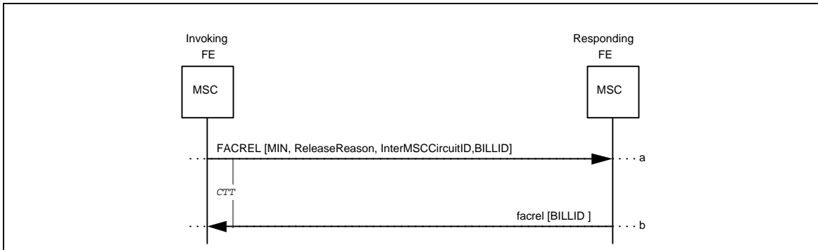
Figure 5 Successful FacilitiesRelease
