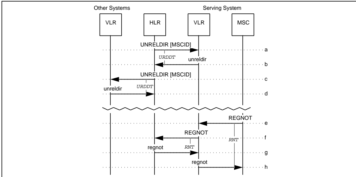
Figure 113 Recovery from data failure at the HLR
