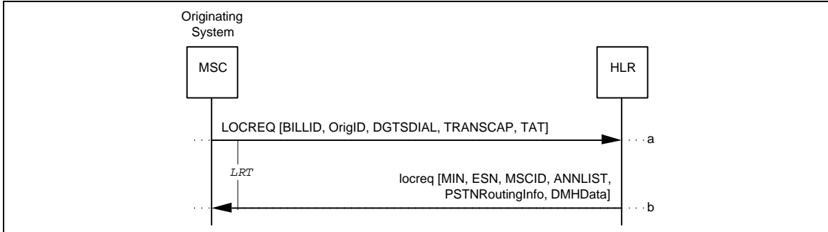
Figure 37 Successful LocationRequest: Route to a PSTN DN
