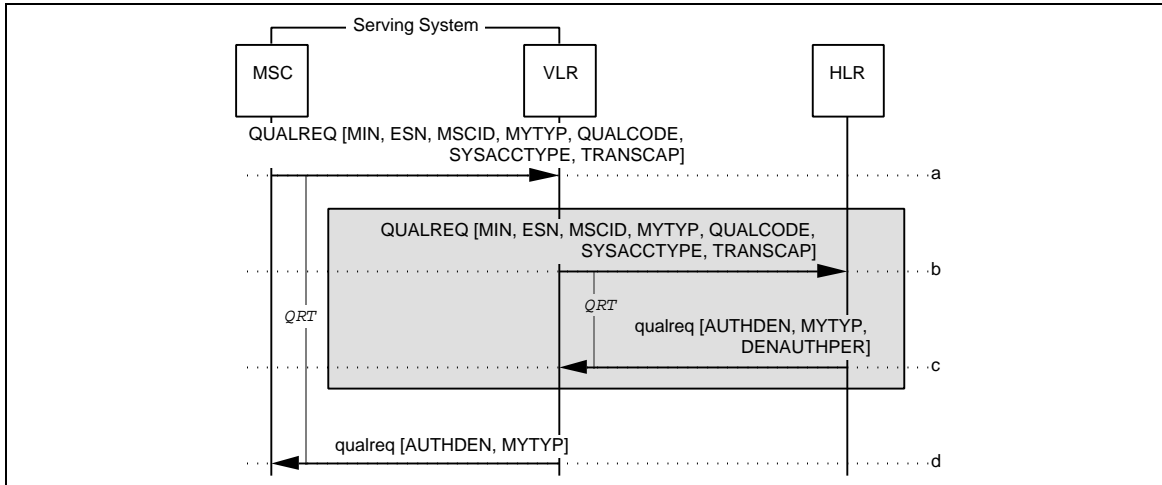
Figure 54 Unsuccessful QualificationRequest: Authorization Denied
