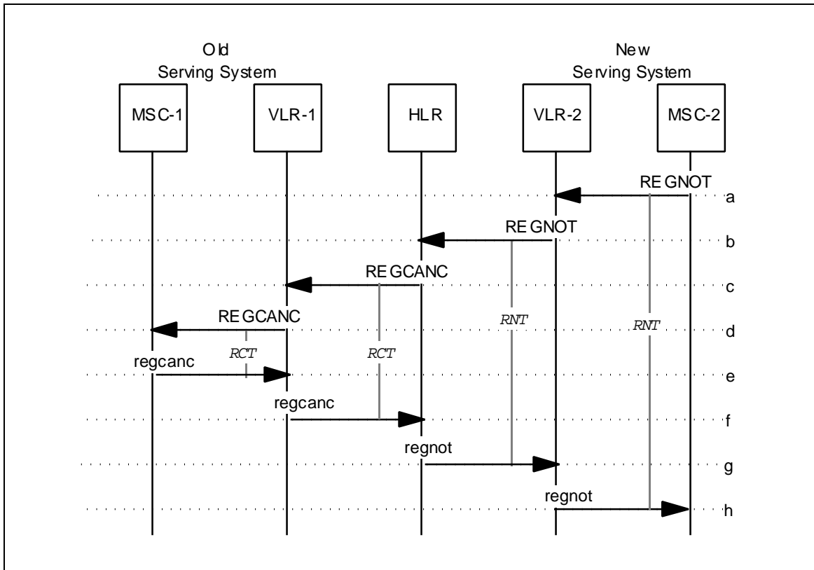
Figure J.1 Initial MS Registration in a New Serving System with Interconnection charge billing system
