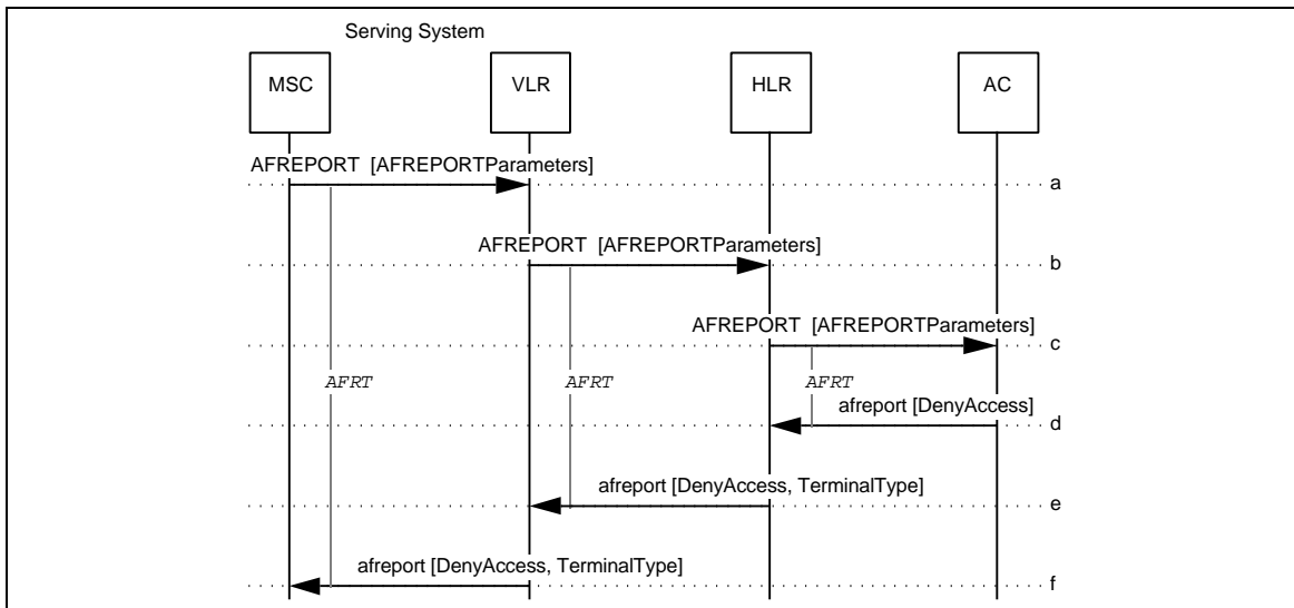
Figure 8 Access Denied on Initial Registration
