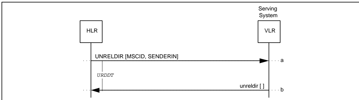
Figure 84 Successful UnreliableRoamerDataDirective
