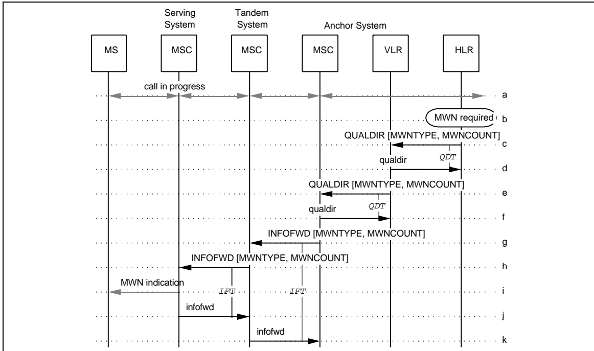
Figure 161 MWN After Handoff
