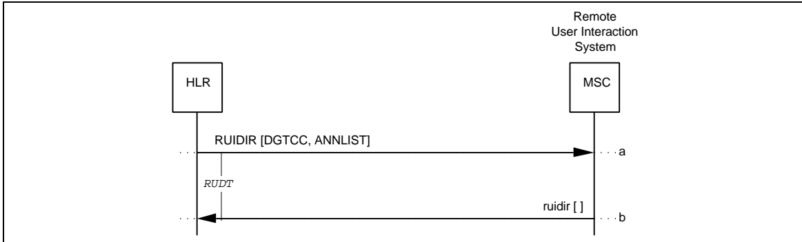
Figure 68 Unsuccessful RemoteUserInteractionDirective
