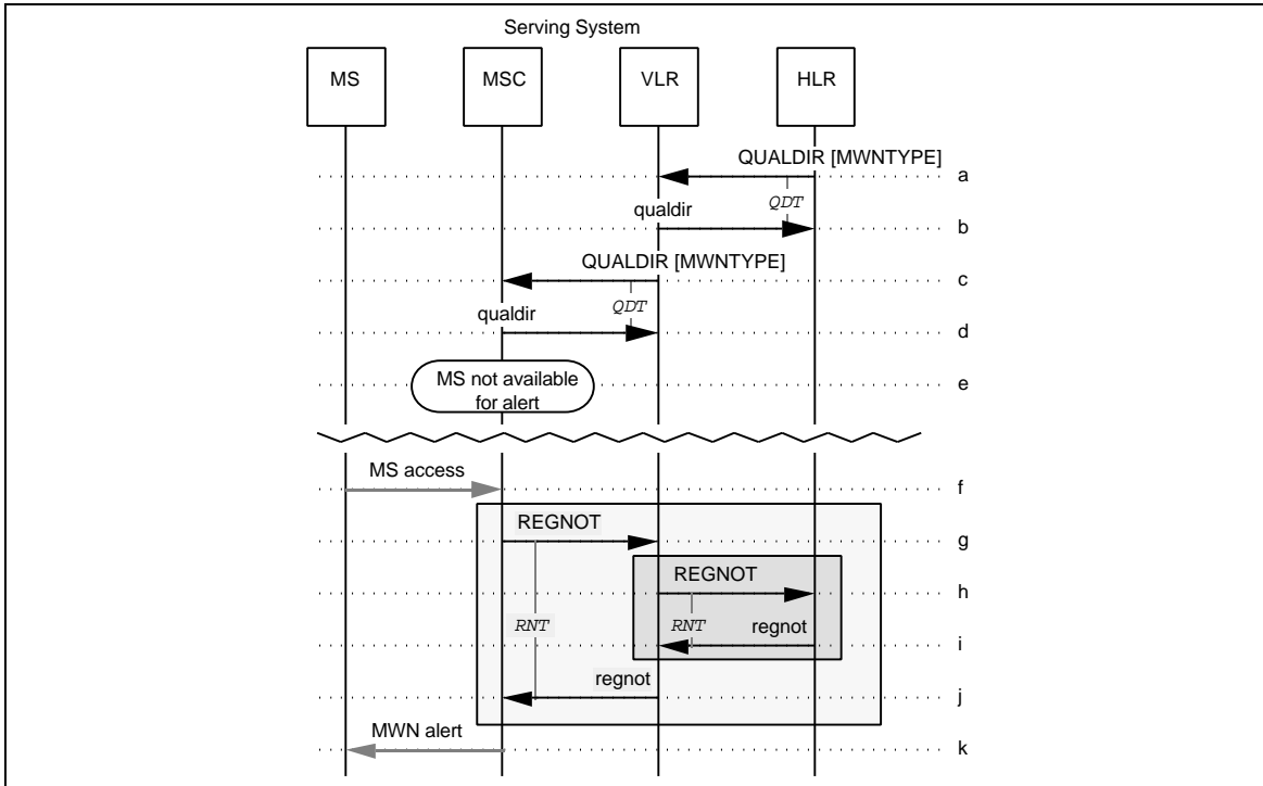
Figure 159 MWN via Alert Pip Tone
