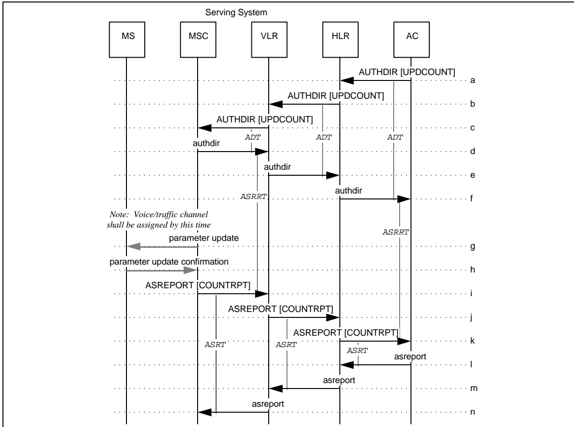
Figure 99 AC Initiated CallHistoryCount Update with SSD Not Shared
