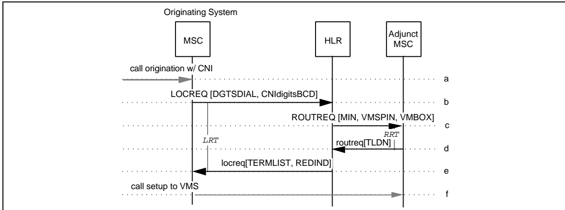
Figure 182 SCA Invocation with Call Refused to Voice Mail
