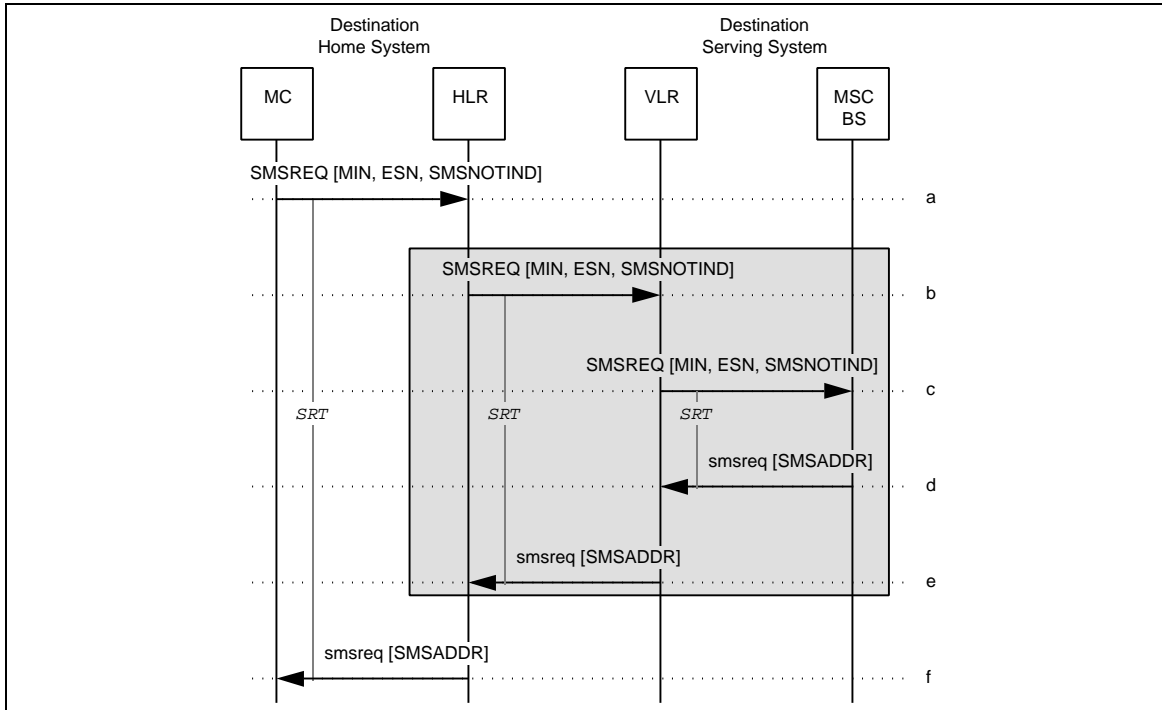
Figure 80 Successful SMSRequest: MS-Based SME Address Request
