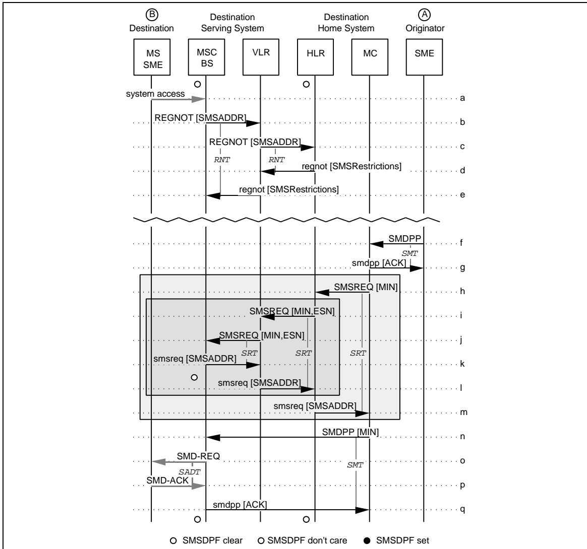
Figure 197 Successful Short Message from a Fixed SME to a Known MS-Based SME
