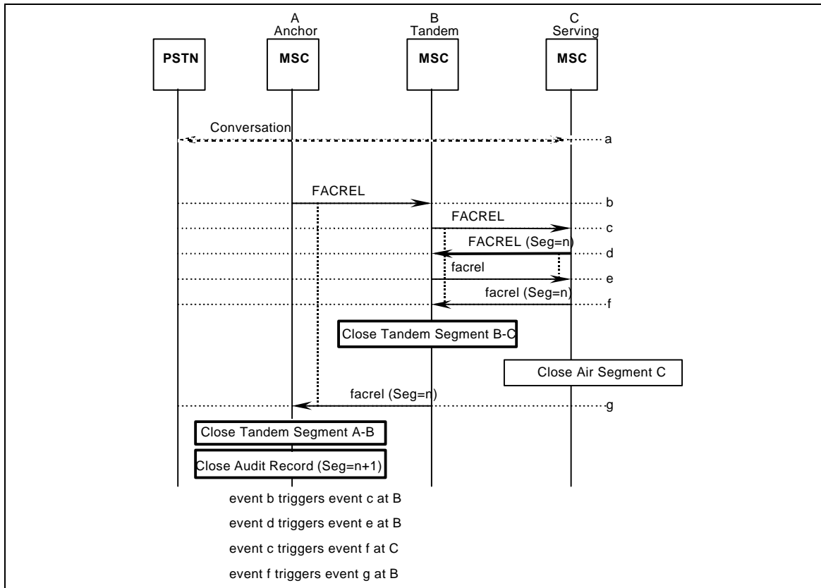
33 34 35 36 37 38 Figure A.8 Release Glare
