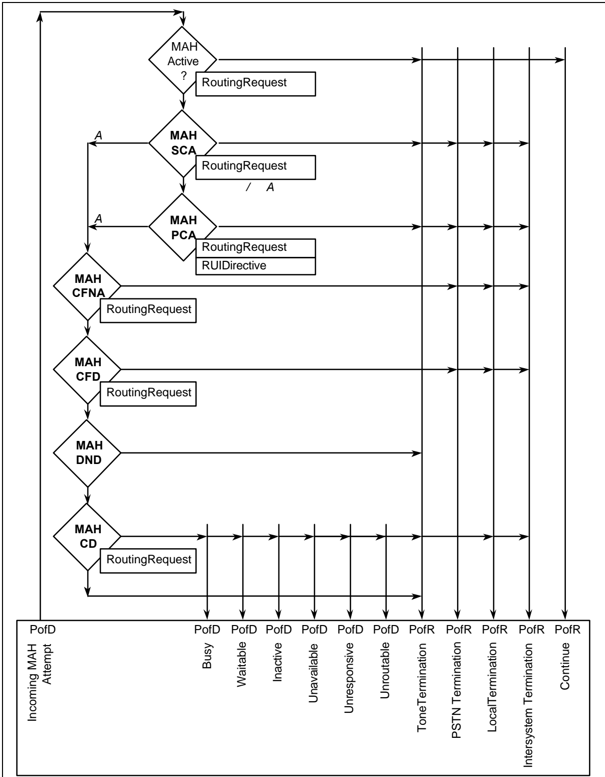
Figure 15 Incoming MAH Call Attempt GSL (HLR)
