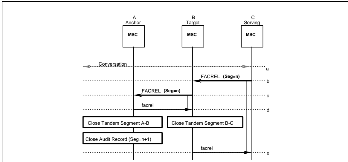
Figure A.6 Release by the MS (C-B-A)
