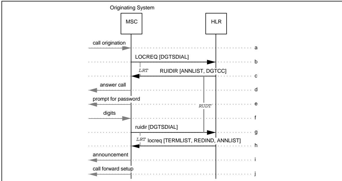
Figure 174 PCA Invocation with Call Refused to Forward-To Number
