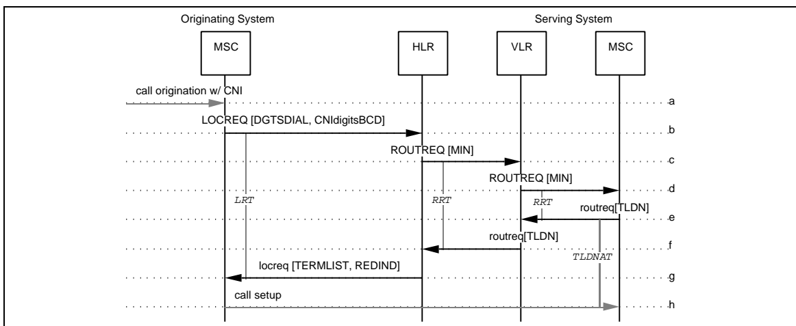
Figure 180 SCA Invocation with Call Accepted
