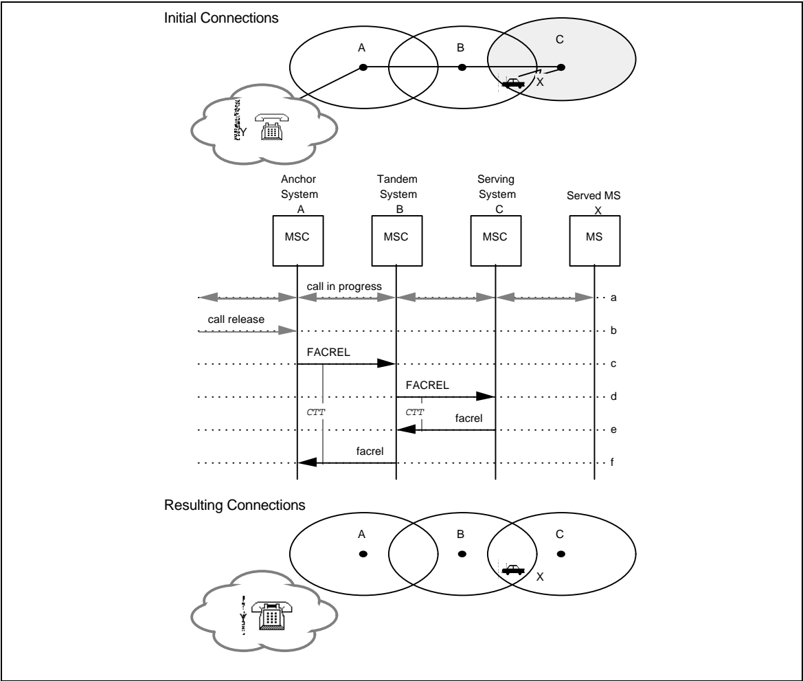
Figure 25 Successful Call Release by Other Party
