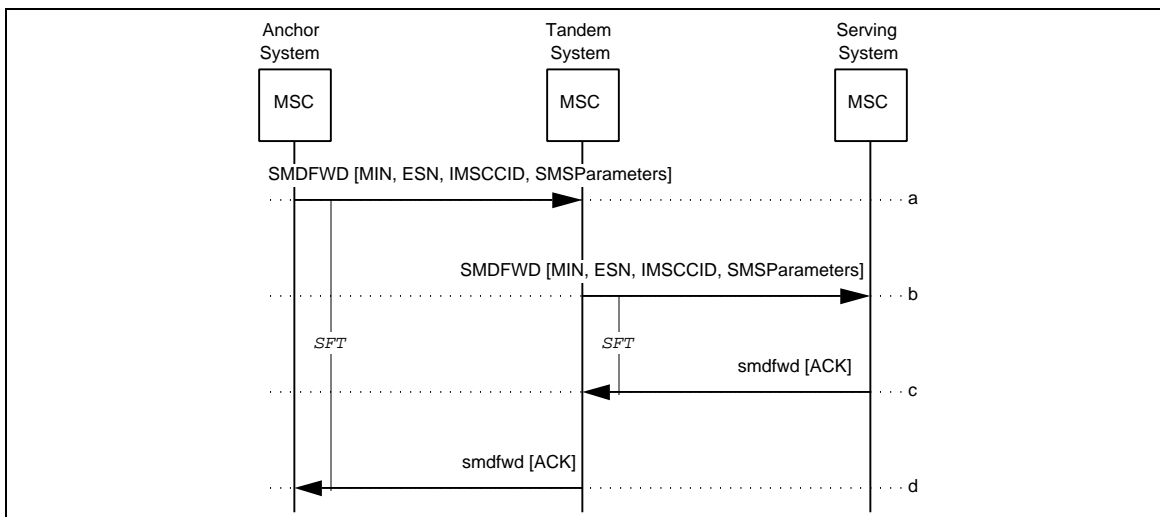
Figure 74 Successful SMSDeliveryForward
