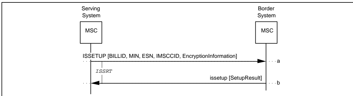
Figure 35 Successful InterSystemSetup
