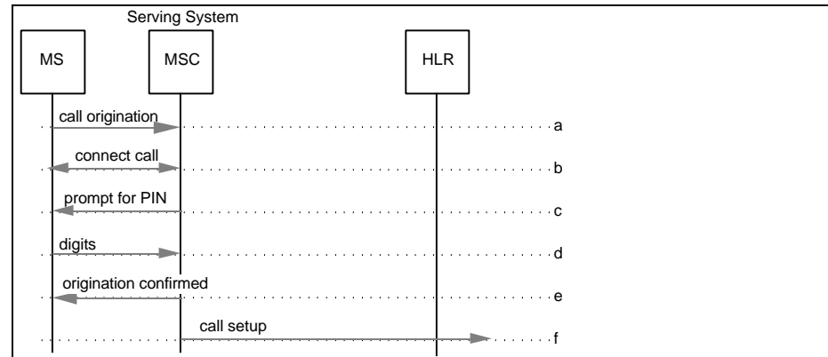
Figure 192 Successful Call Origination with Local SPINI Operation
