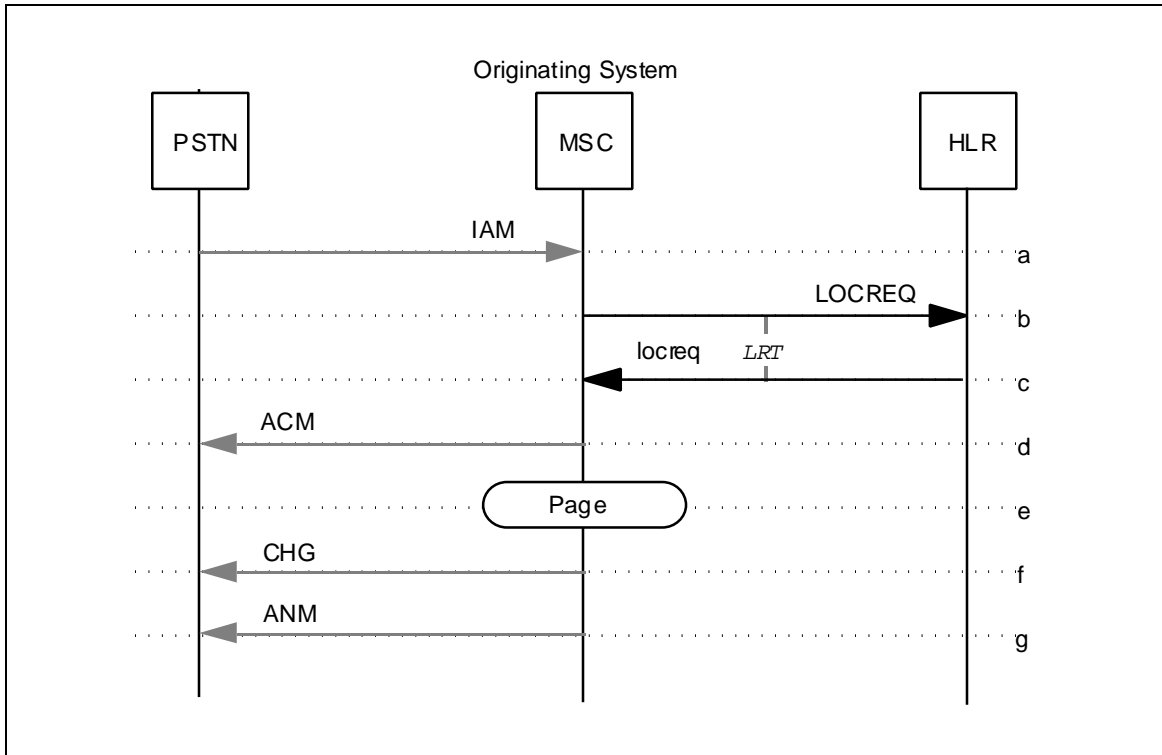
Figure J.2 CD Invocation to an Idle, Local MS with Interconnection charge billing system
