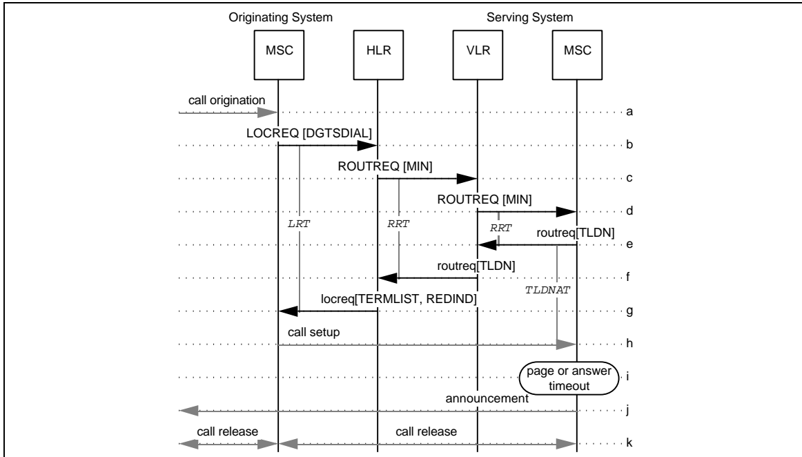
Figure 117 CD Invocation with No Page Response or No Answer
