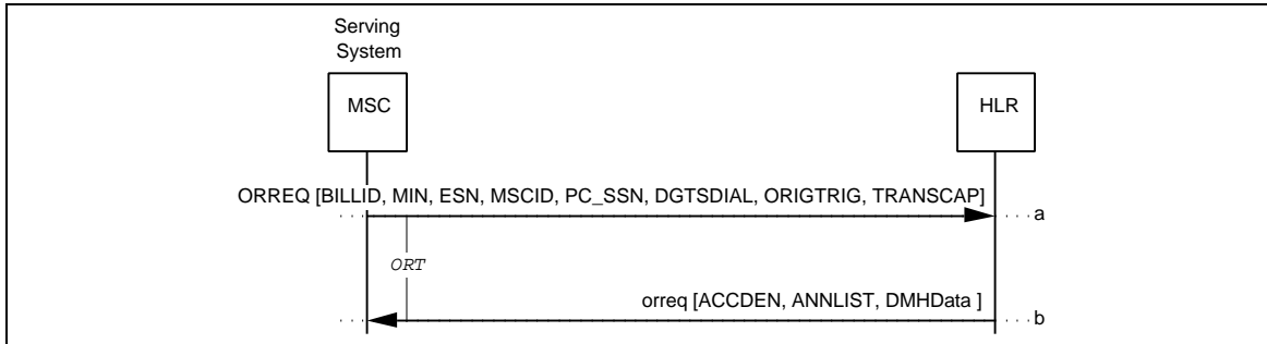
Figure 46 Unsuccessful OriginationRequest
