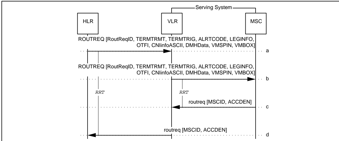
Figure 71 Unsuccessful RoutingRequest: Access Denied Returned
