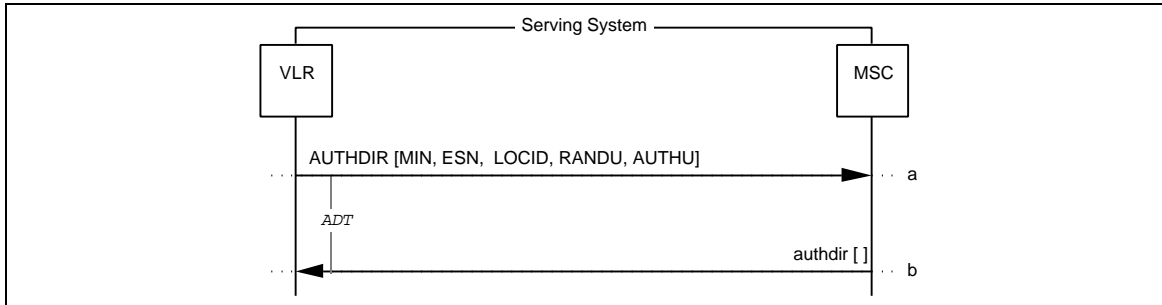
19 20 Figure 4 VLR-Initiated Unique Challenge
