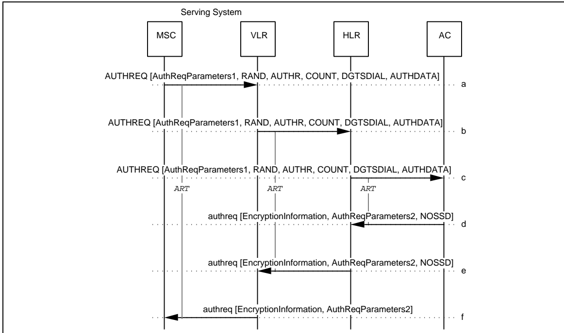
Figure 11 Successful Authentication on Call Origination (SSD not shared)
