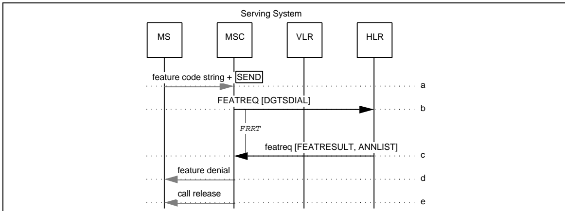
Figure 107 Feature Request Denial with Call Release
