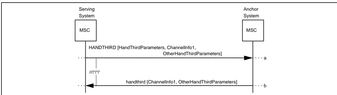
Figure 12 Successful HandoffToThird
