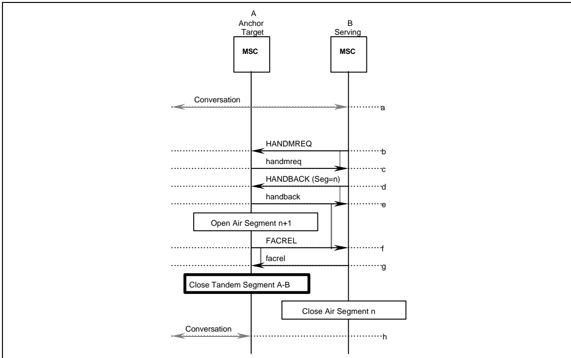
Figure A.2 Handoff-Back (B to A)
