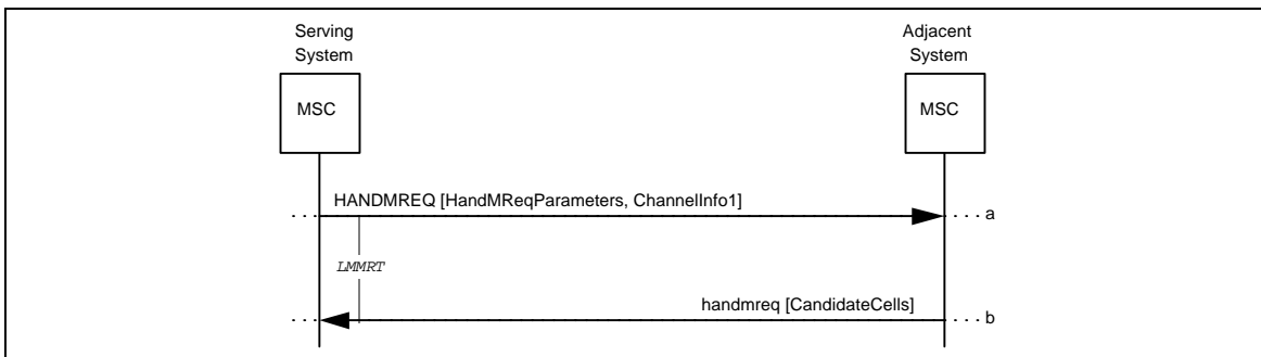
Figure 10 Successful HandoffMeasurementRequest
