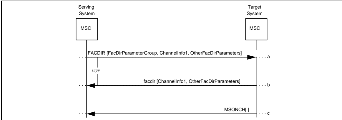
Figure 1 Successful FacilitiesDirective
