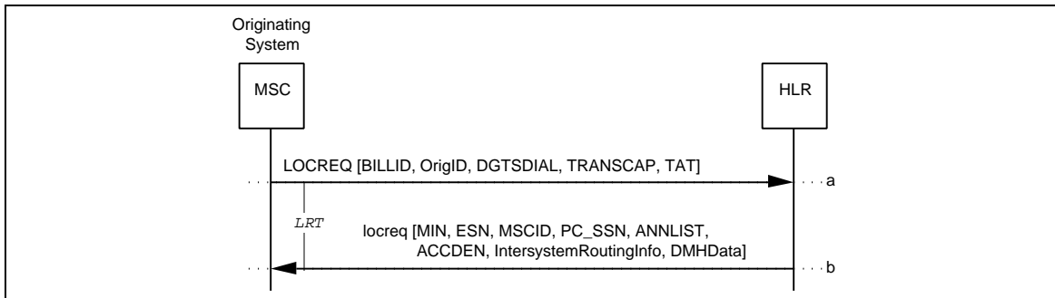
Figure 40 Successful LocationRequest: Routing Information and Access Denied Indication Returned
