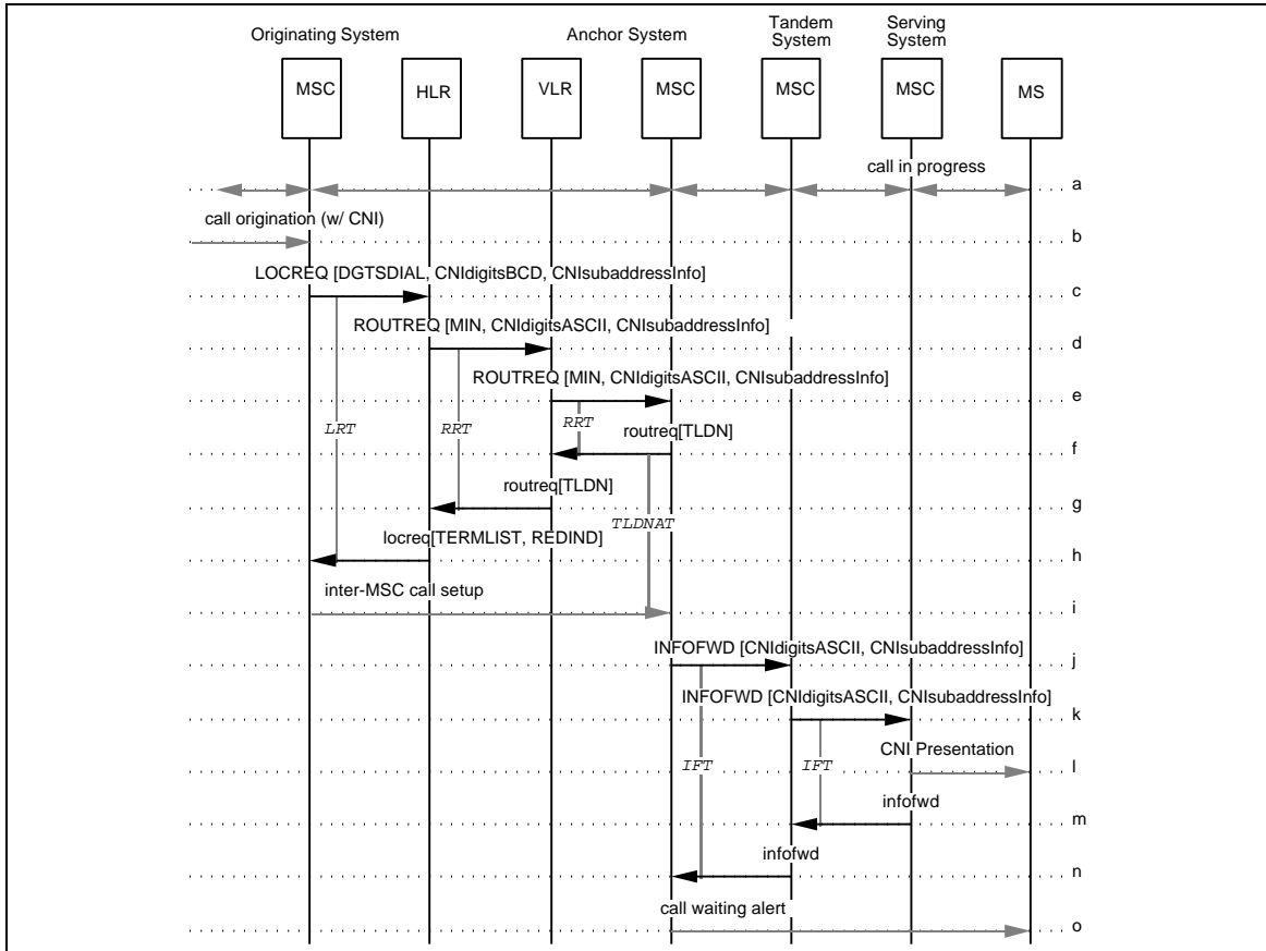
Figure 137 CNIP Interaction with Call Waiting After Handoff
