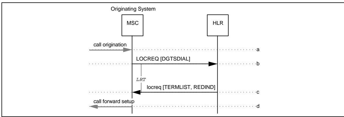
Figure 128 CFD Invocation (Immediate)
