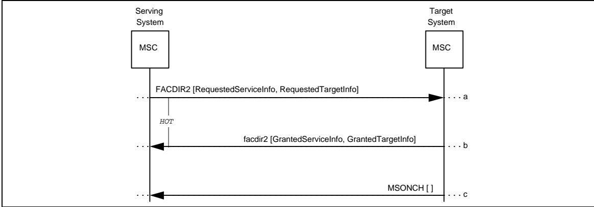
Figure 3 Successful FacilitiesDirective2
