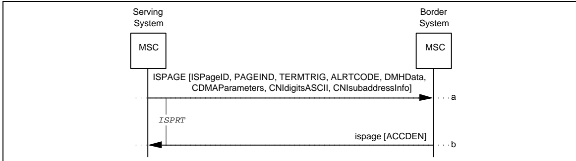
Figure 30 Unsuccessful InterSystemPage: Border MSC Access Denied
