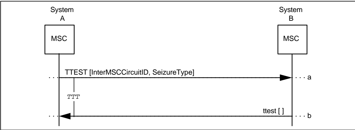
Figure 4 Normal Operation (TrunkTest)
