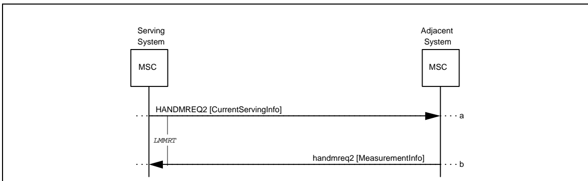
Figure 11 Successful HandoffMeasurementRequest2
