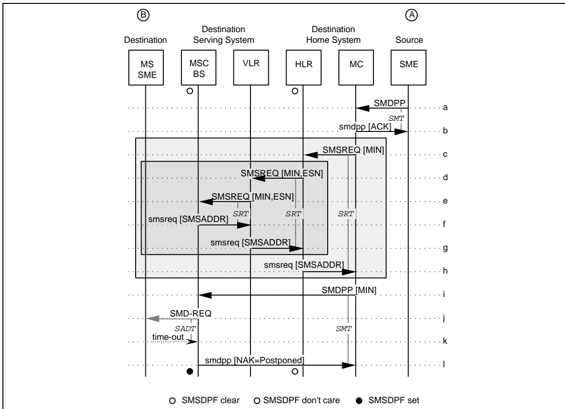
Figure 200 Short Message Time-Out to an MS-Based SME with Notification
