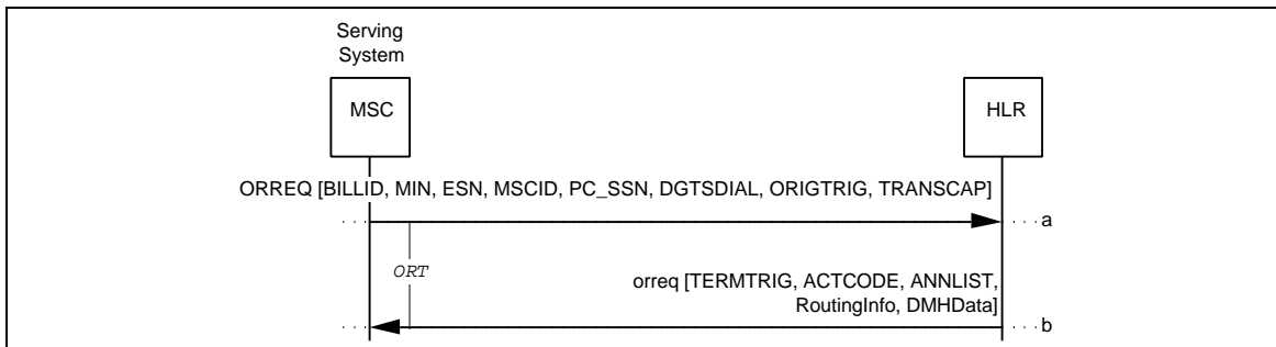
Figure 45 Successful OriginationRequest
