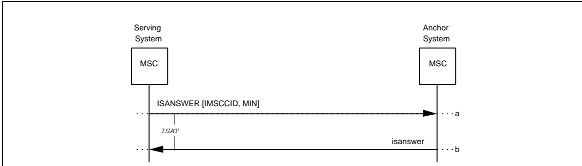
Figure 17 Successful InterSystemAnswer Following the Handoff of a Terminating MS in the Alerting State
