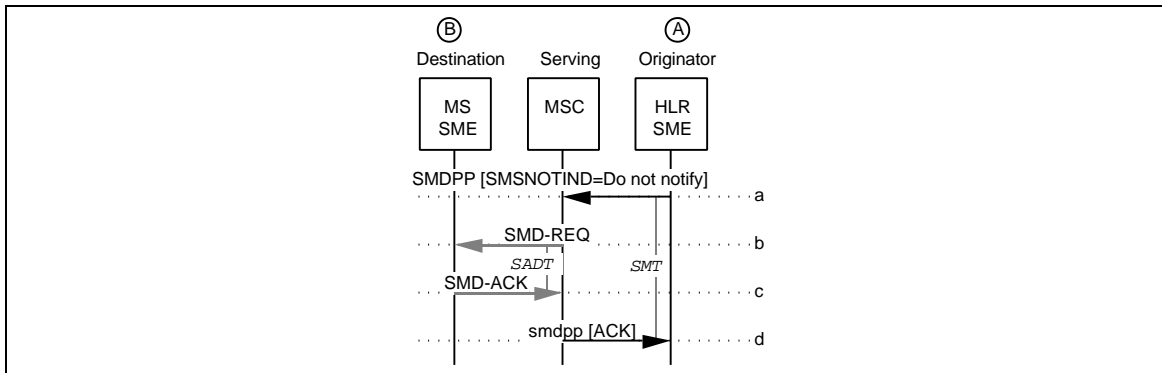
Figure 218 Short Message Between HLR Based SME and MS-Based SME
