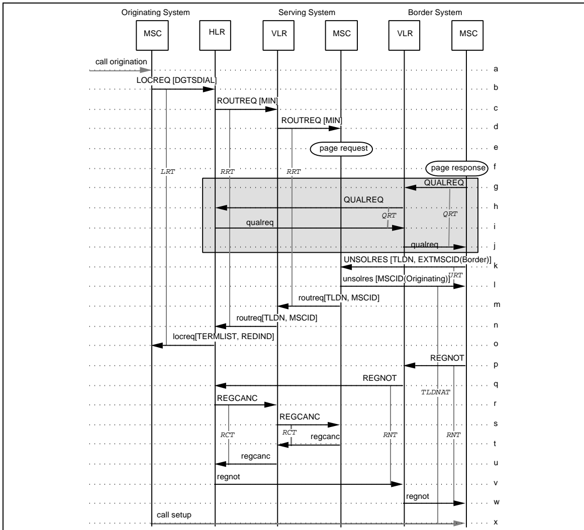
Figure 120 CD Invocation with Unsolicited Page Response
