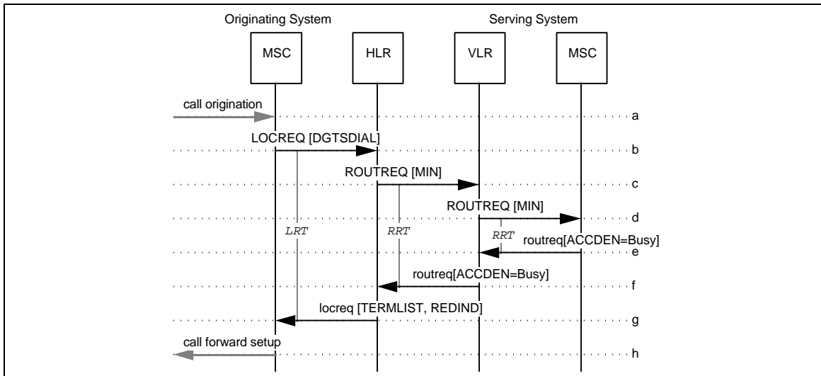
Figure 126 CFB Invocation
