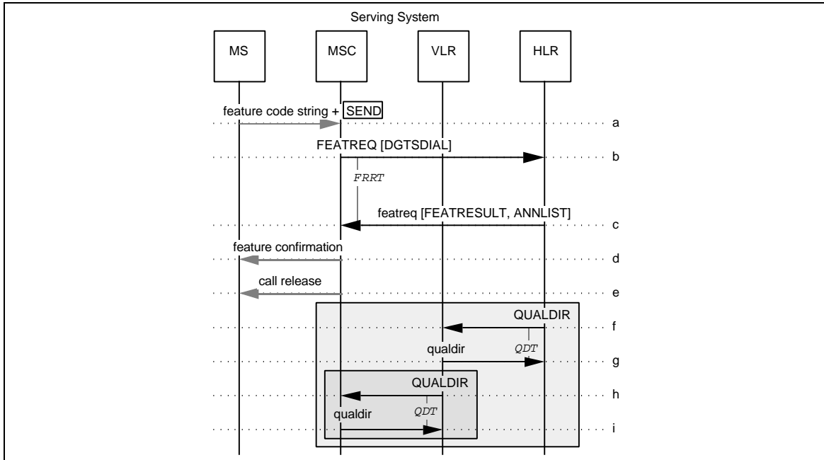
Figure 105 Feature Request Confirmation with Release
