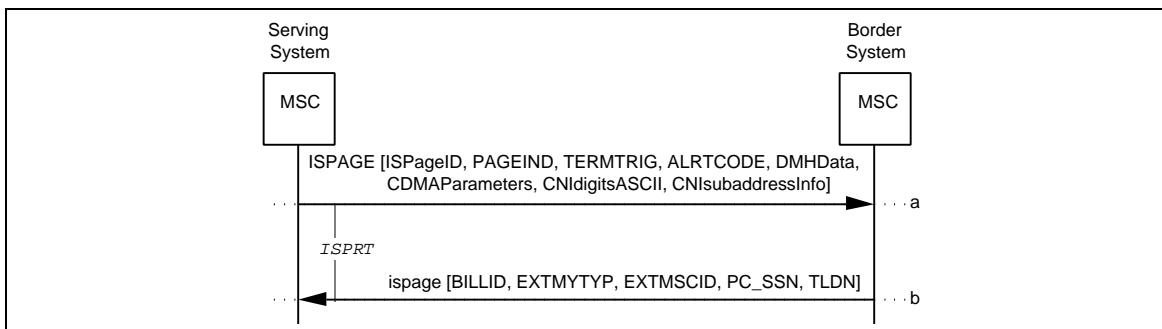
Figure 29 Successful InterSystemPage: Border MSC Routing Information Returned
