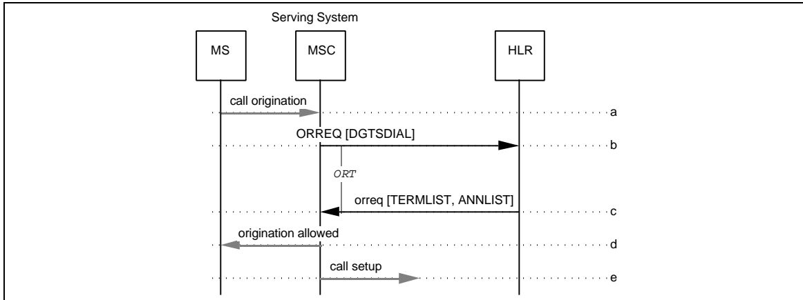
Figure 190 Call Origination with SPINI Active and PIN Not Required
