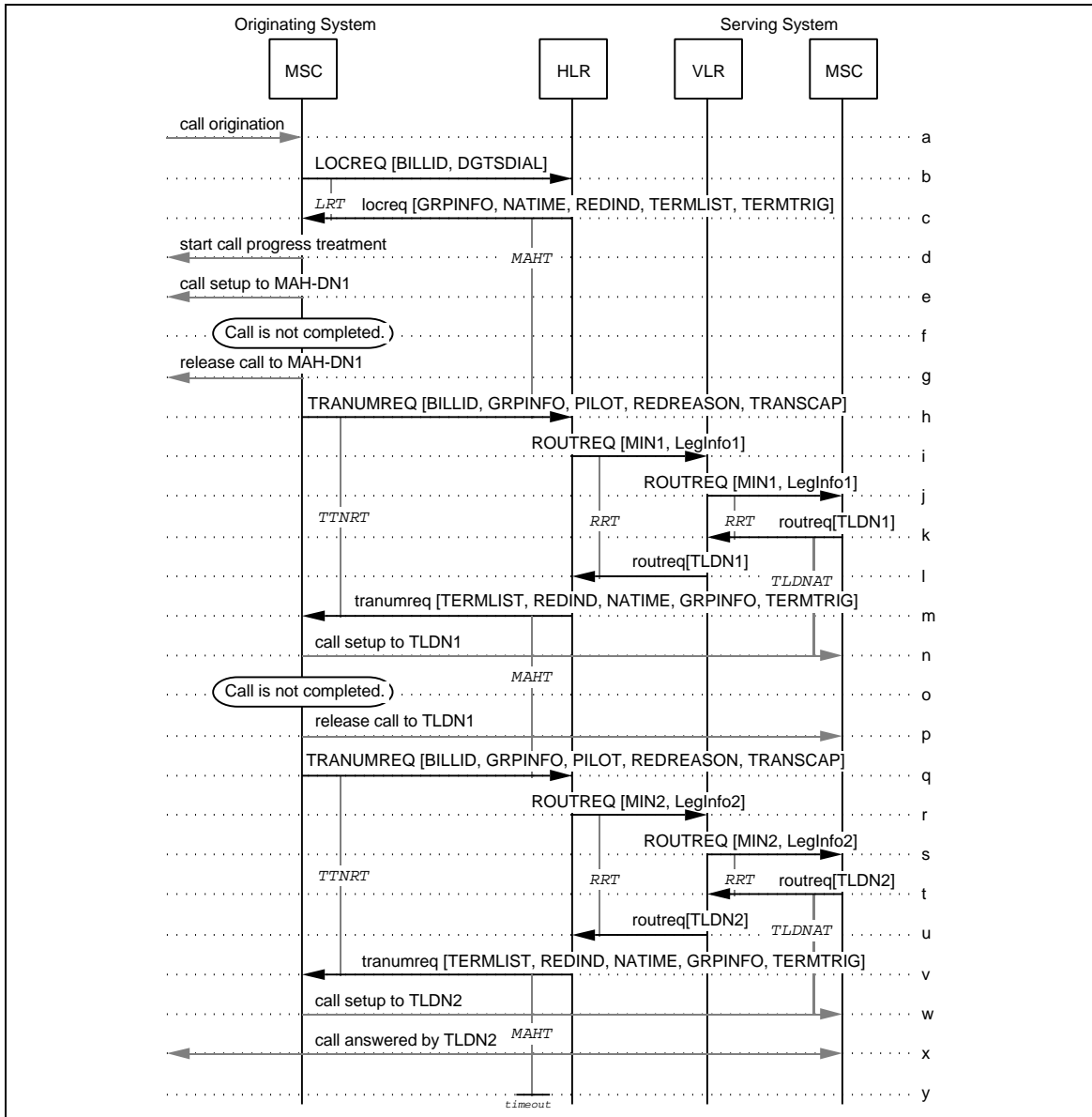
Figure 164 MAH Invocation
