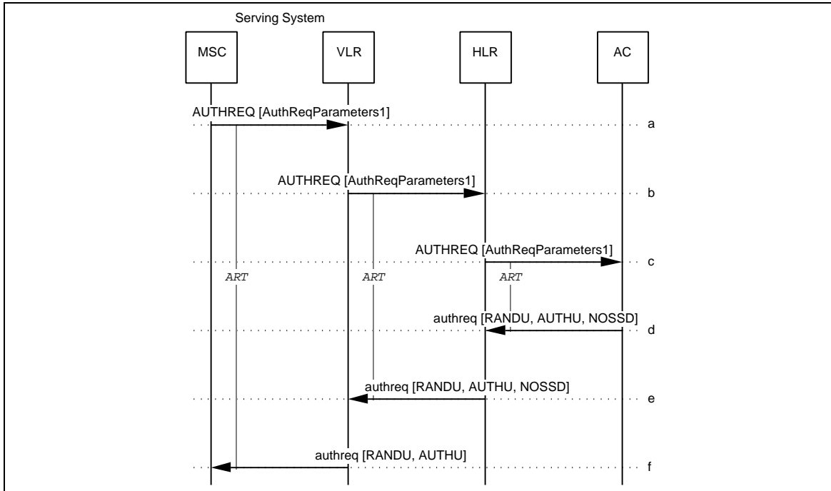
Figure 13 Initiate Authentication on Voice Channel (SSD not shared)
