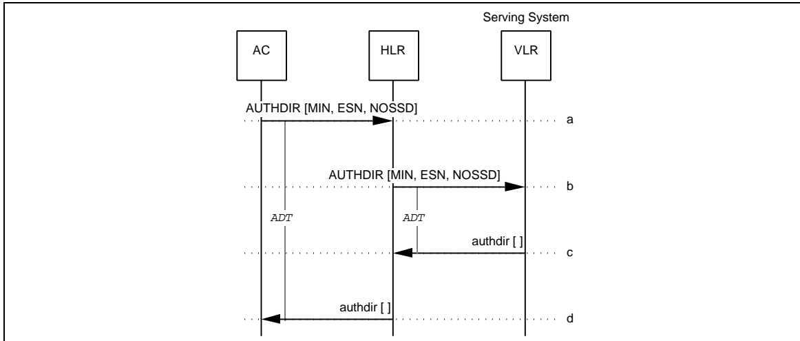
Figure 6 Revocation of SSD Sharing
