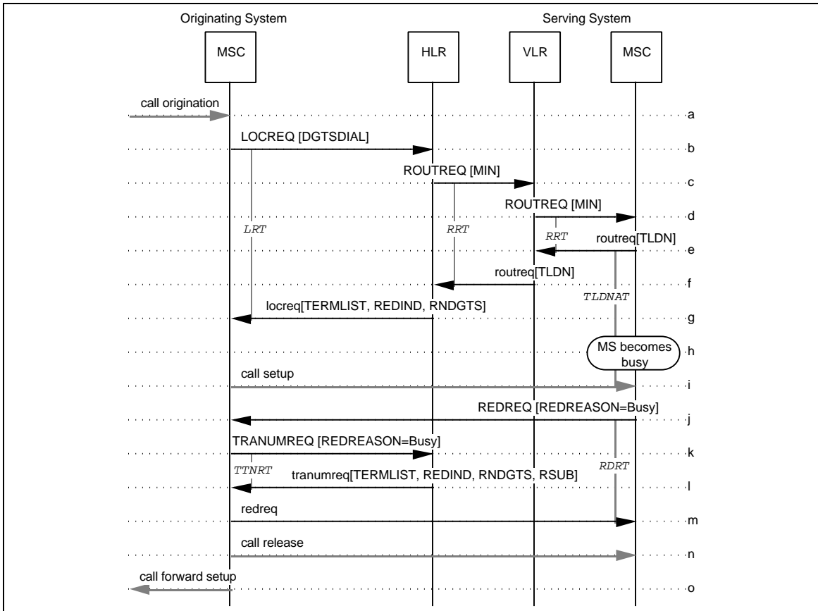
Figure 144 CNIR Interaction with CFB or CFD on Call Collision
