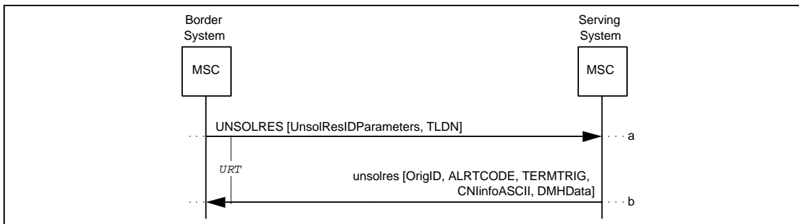
Figure 85 Successful UnsolicitedResponse
