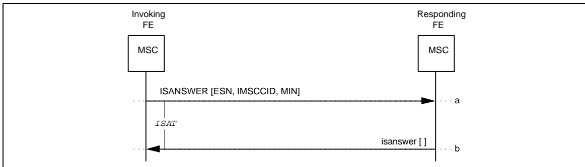
Figure 28 Successful InterSystemAnswer
