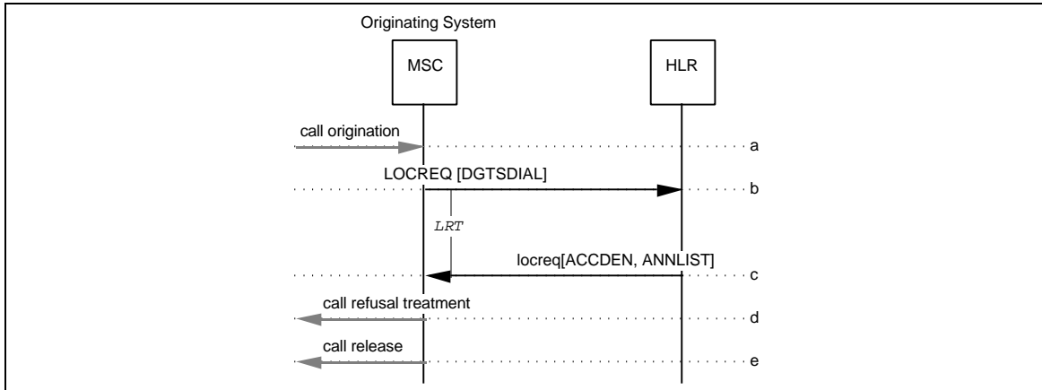
Figure 118 CD Invocation to an Inaccessible MS
