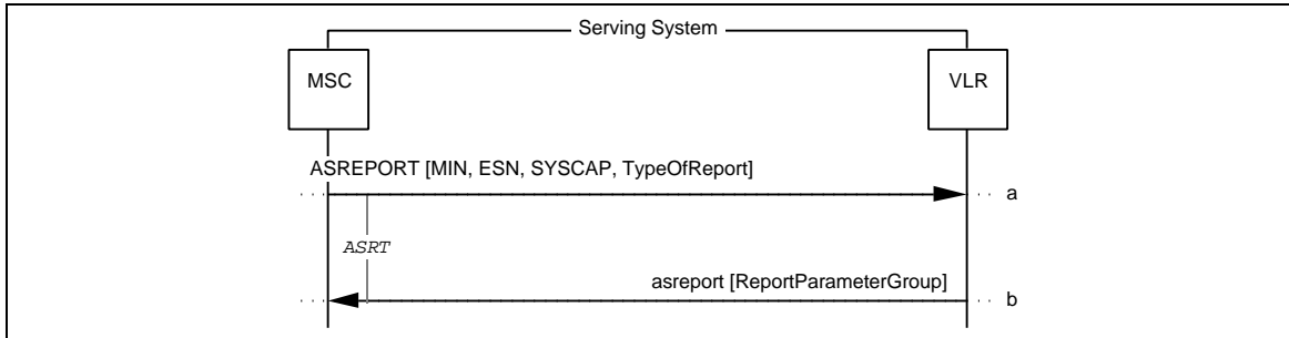
Figure 18 Report of VLR-initiated action
