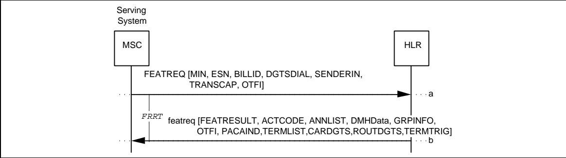
Figure 24 Direct FeatureRequest with Call Routing
