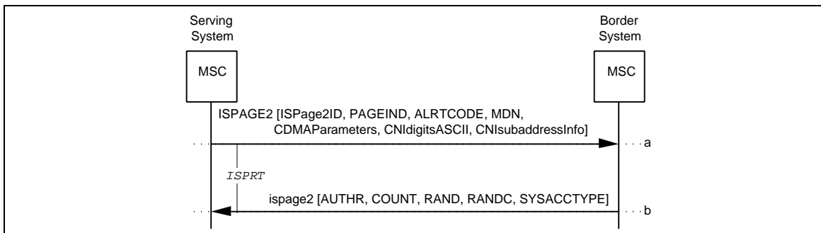
Figure 32 Successful InterSystemPage2: MS Presence Confirmed in Border MSC
