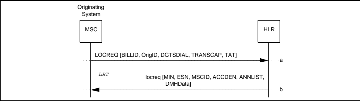
Figure 42 Unsuccessful LocationRequest: Access Denied without Routing Information Returned
