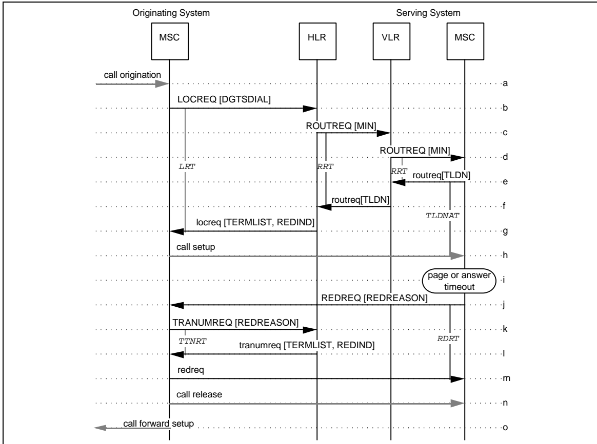
Figure 129 CFD Invocation with No Answer or No Response to Page
