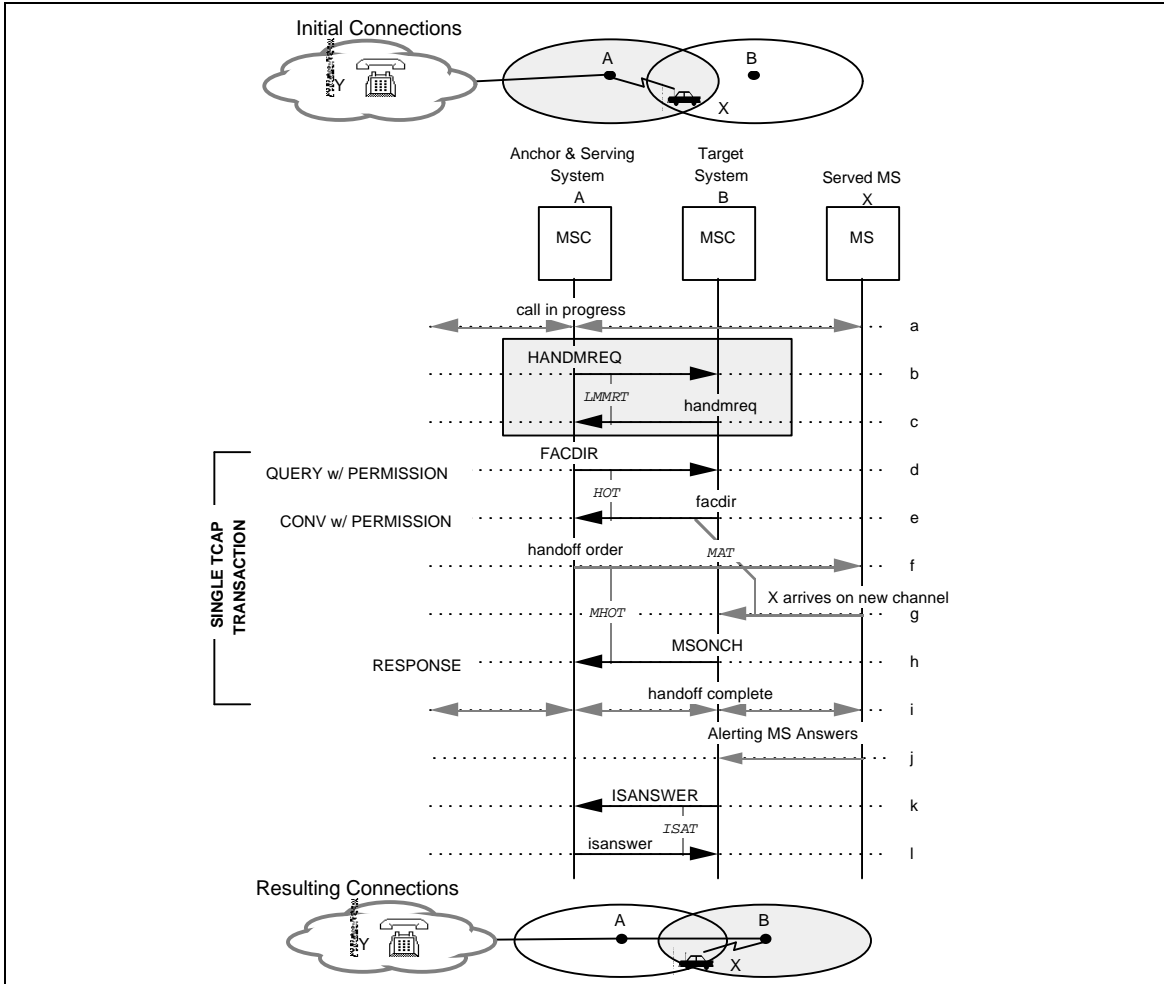
Figure 27 Successful Handoff-Forward of a Terminating MS While Alerting
