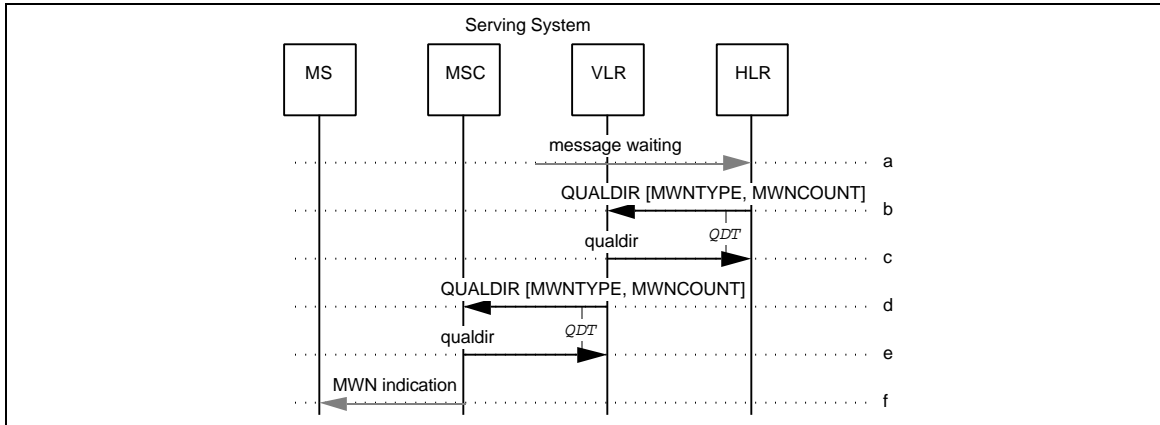
Figure 160 MWN via an MS Indication and/or MS Count
