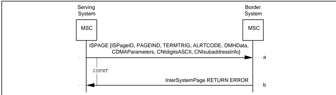
Figure 31 Unsuccessful InterSystemPage: Border MSC Resource Shortage
