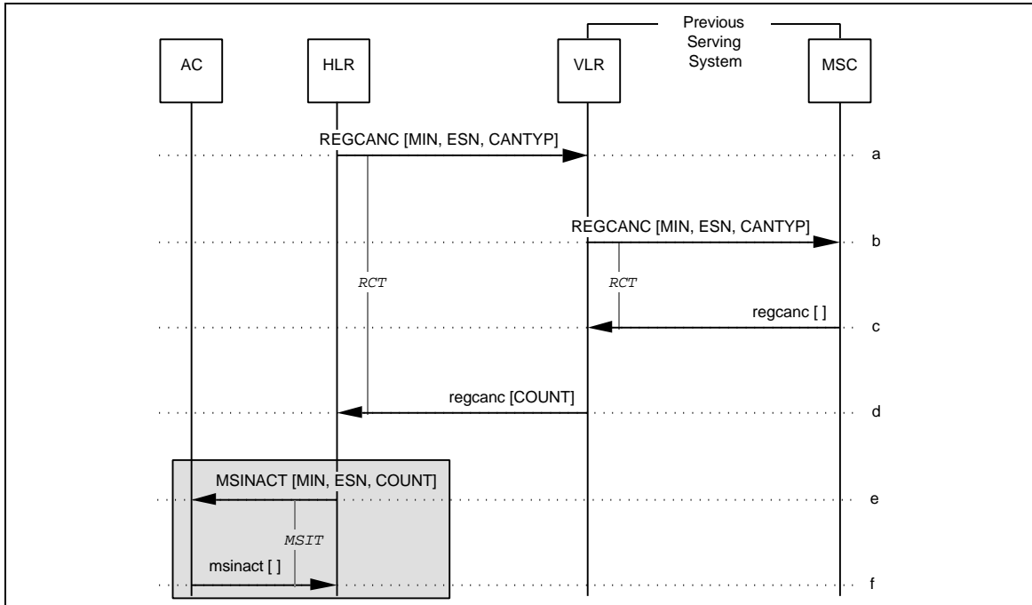
Figure 104 RegistrationCancellation with CallHistoryCount Report
