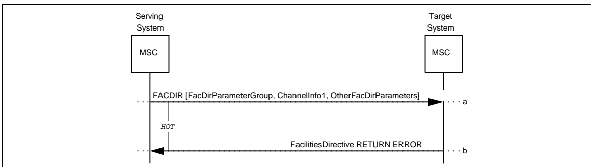
Figure 2 Unsuccessful FacilitiesDirective
