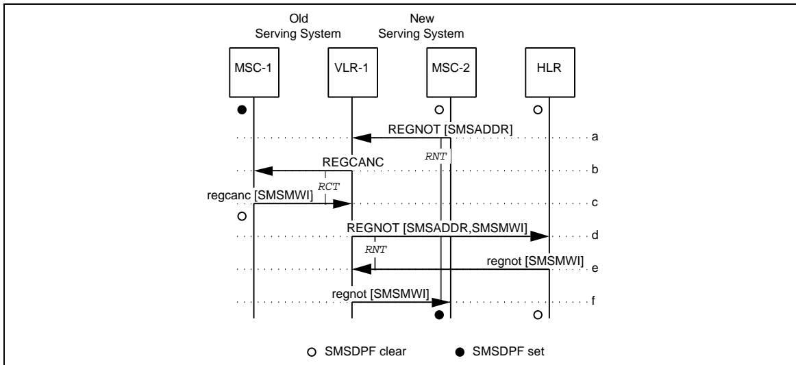
Figure 211 Local Roaming Between SMS-Capable Systems with Pending Postponed Delivery
