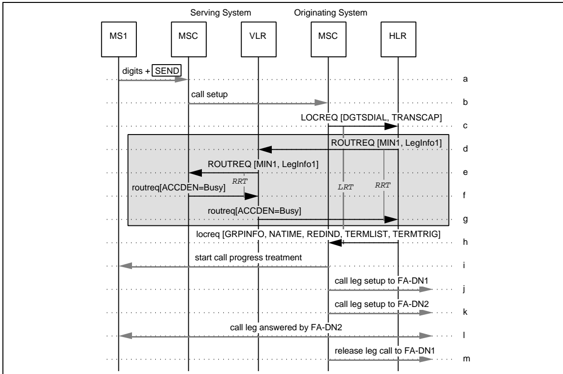
Figure 157 FA Invocation on Call from FA Group Member
