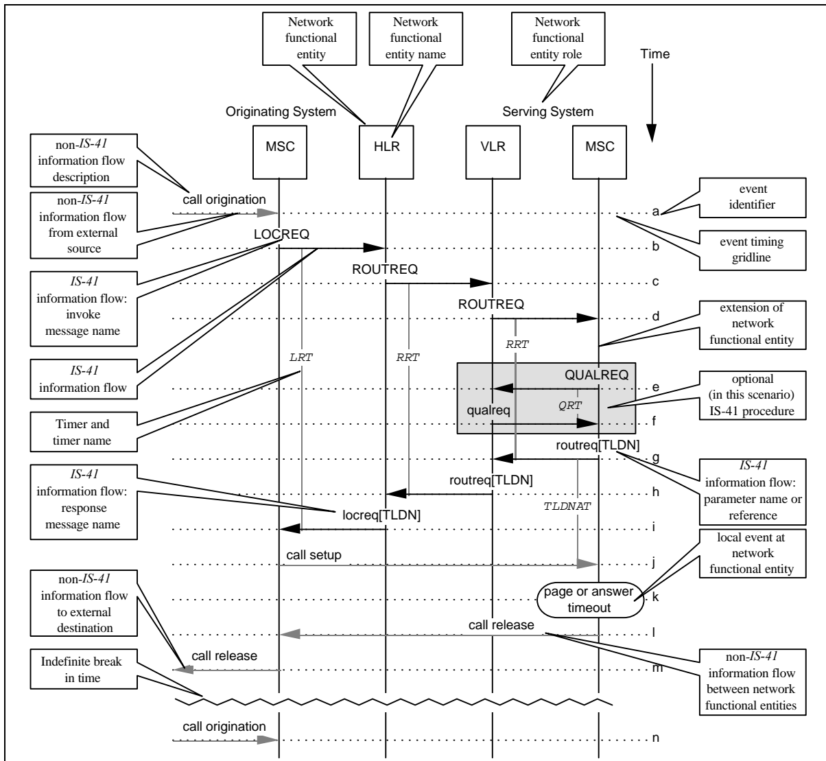
Figure 1 Diagrammatic Conventions
