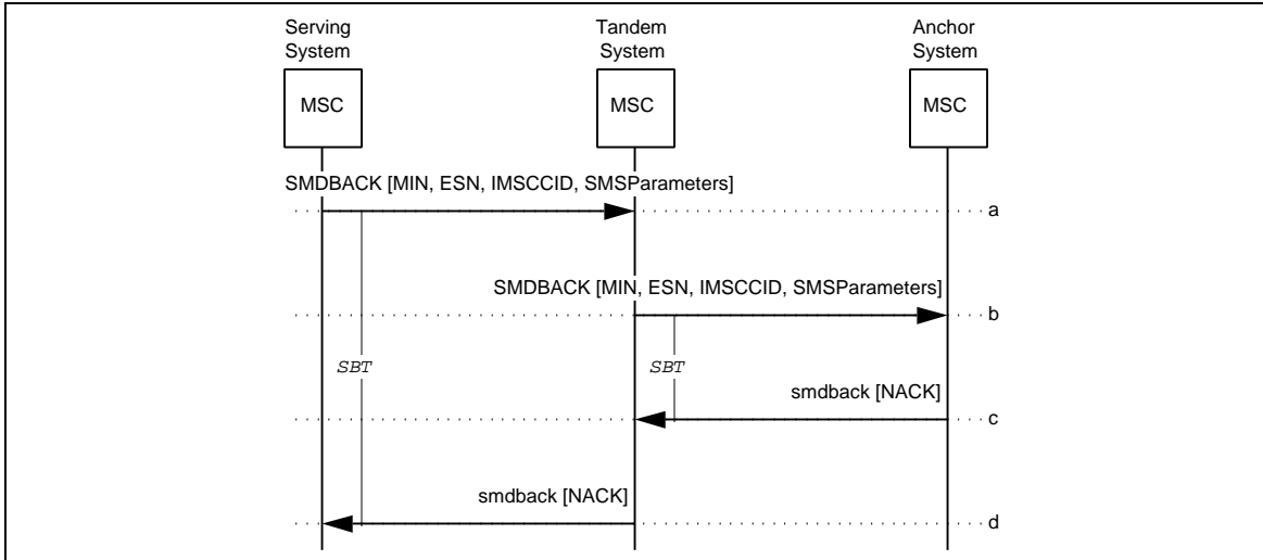
Figure 73 Unsuccessful SMSDeliveryBackward
