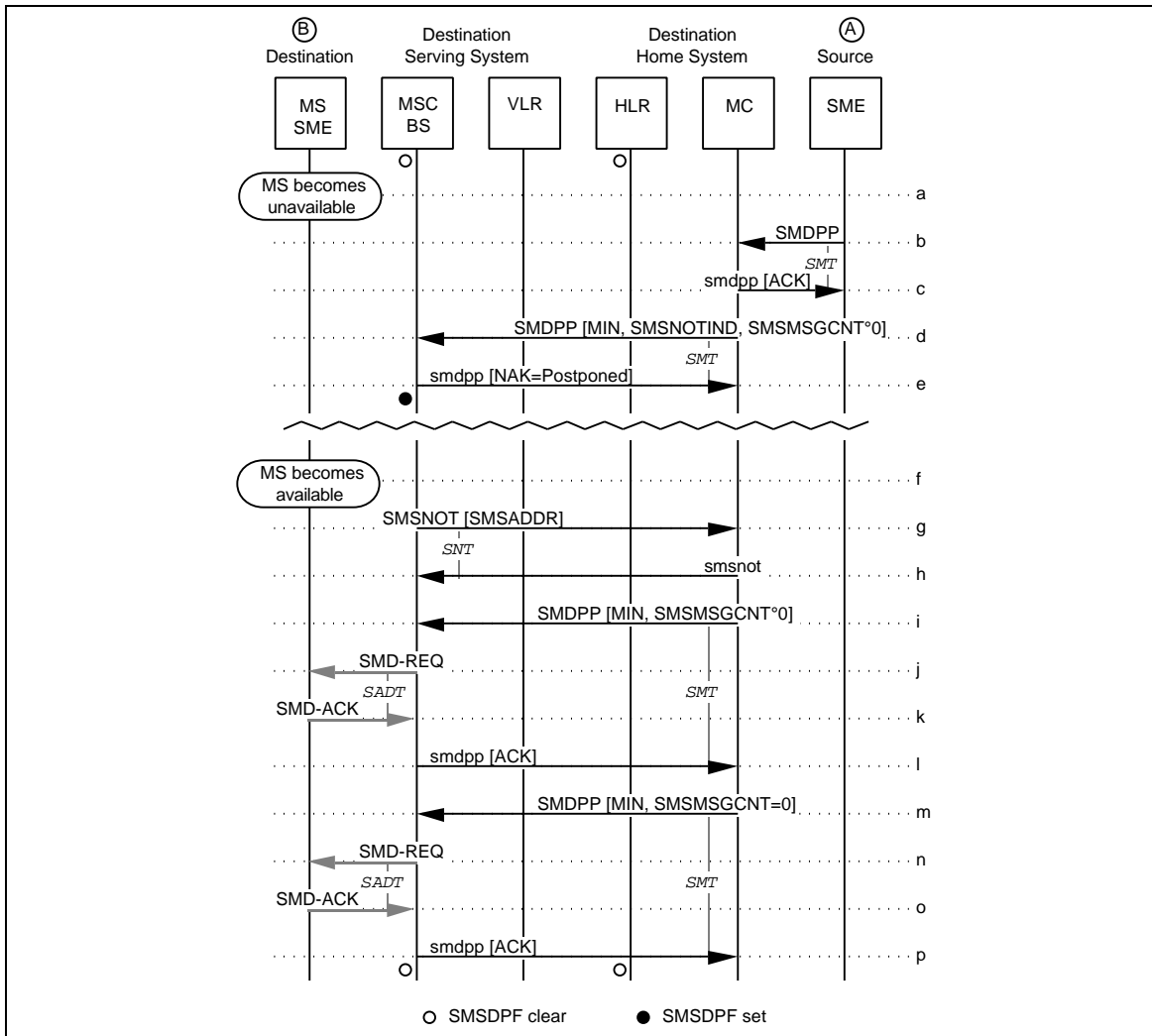
Figure 216 Postponed MSC SMSNotification with Multiple SMDPPs
