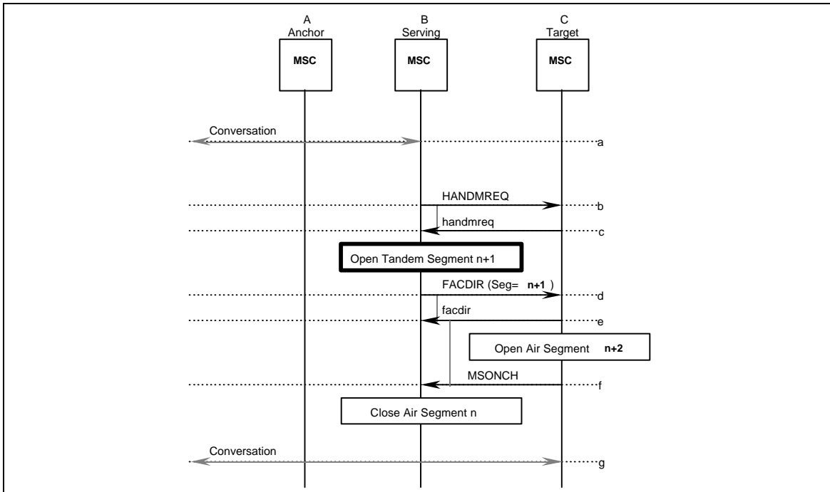
Figure A.3 Handoff-Forward (B to C)
