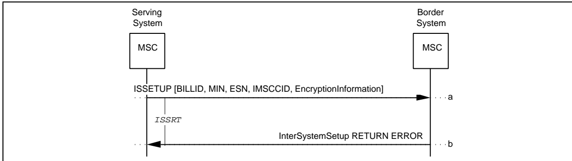
Figure 36 Unsuccessful InterSystemSetup
