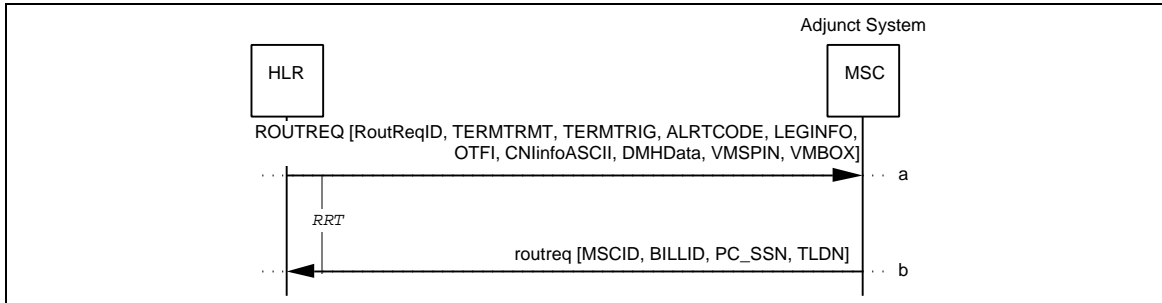
Figure 70 Successful Direct RoutingRequest: TLDN Returned
