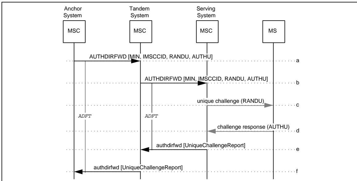
Figure 7 Successful AuthenticationDirectiveForward
