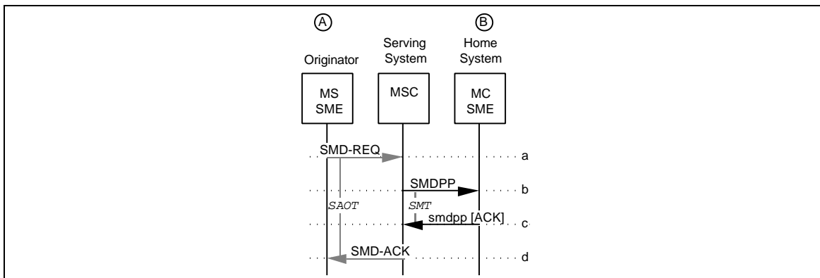
Figure 219 Short Message Between MS-Based SME and MC for MC-Based Feature Control
