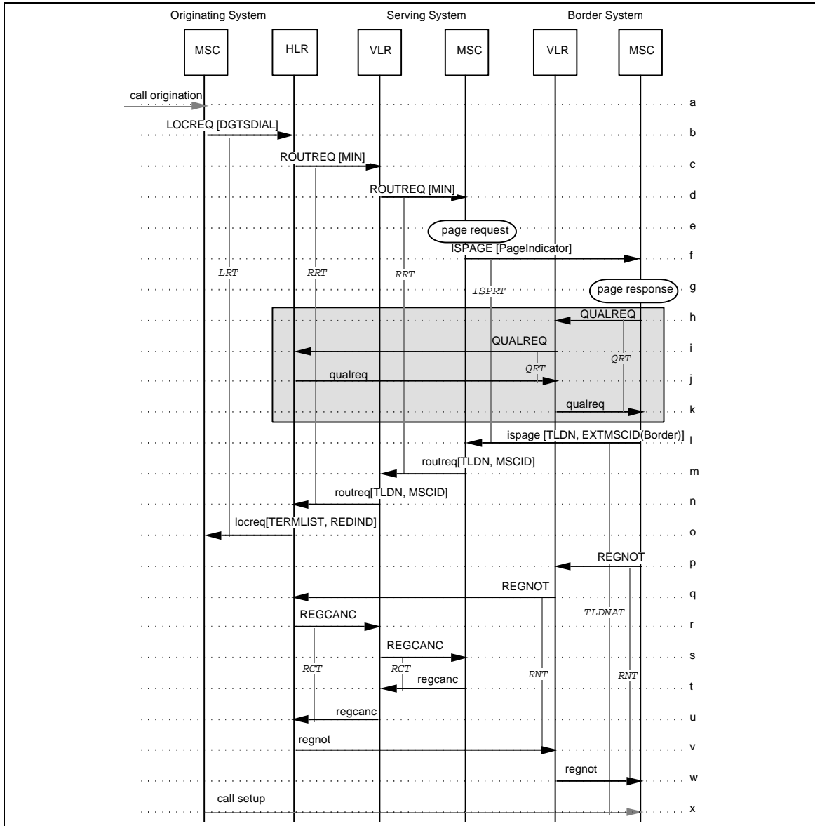
Figure 119 CD Invocation with Intersystem Paging
