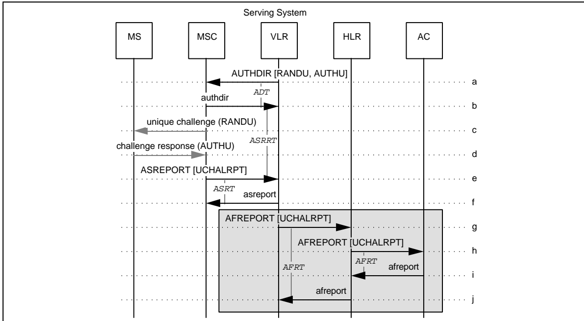
Figure 103 VLR Initiated Unique Challenge When SSD is Shared. The Serving VLR chooses a Unique Random Variable (RANDU) and executes CAVE using the SSD-A currently stored, ESN, MIN1 and MIN2 associated with the MS to produce an Authentication Response for Unique Challenge (AUTHU).
