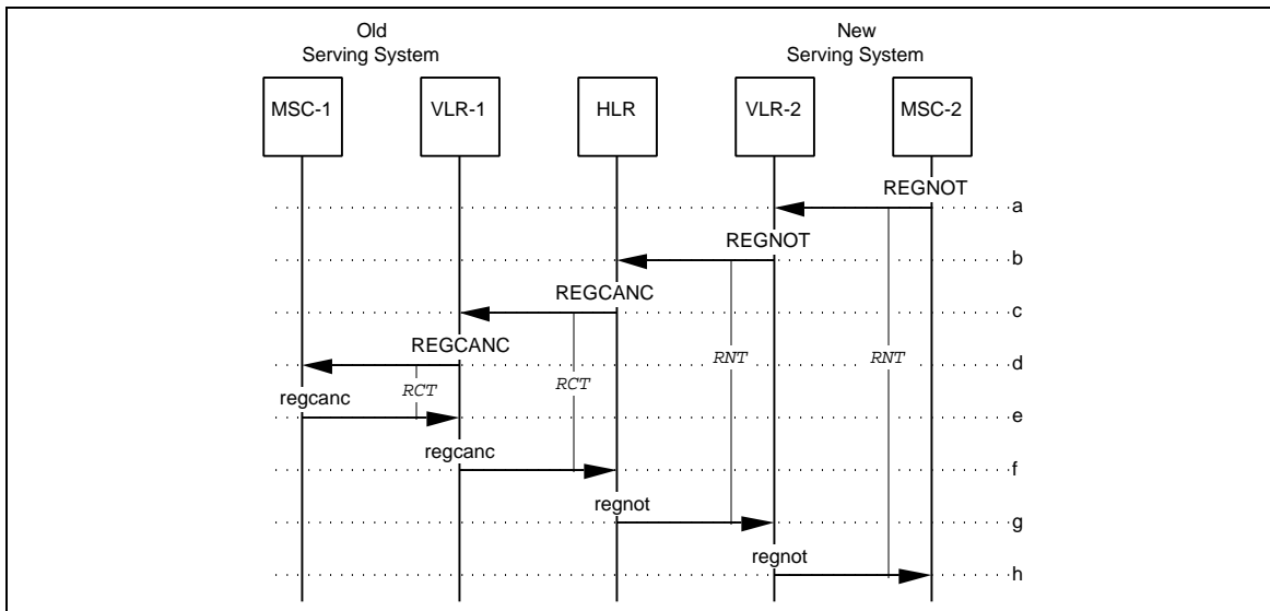
Figure 87 Initial MS Registration in a New Serving System
