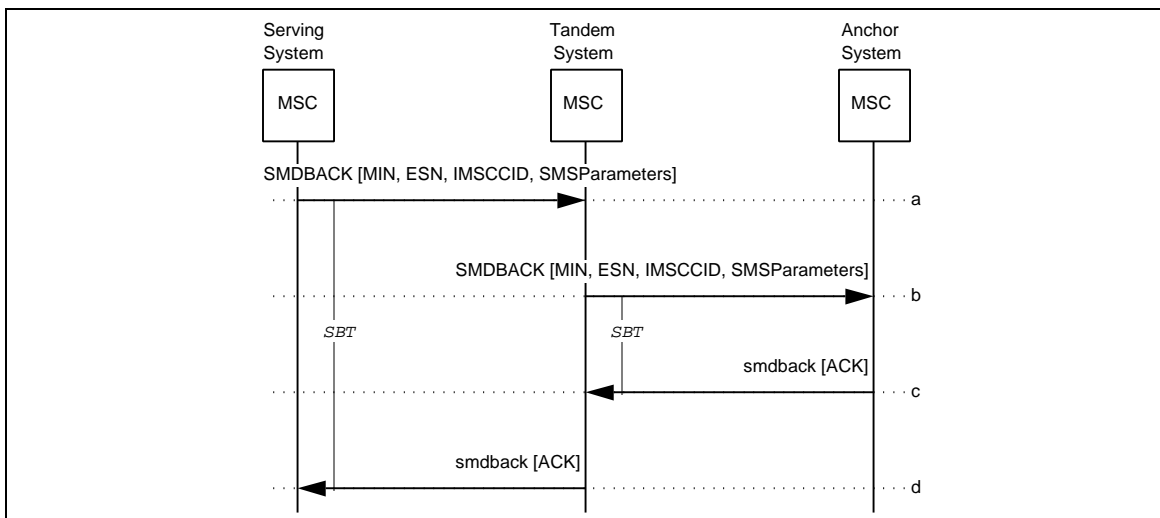
Figure 72 Successful SMSDeliveryBackward
