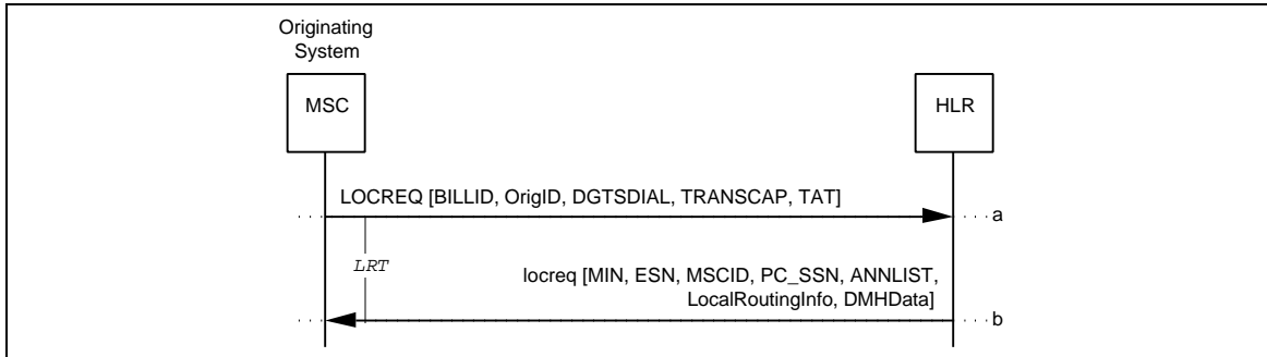
Figure 38 Successful LocationRequest: Route to a Local MS
