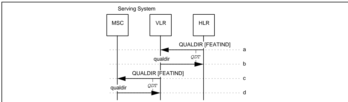
Figure 196 VP Profile Change
