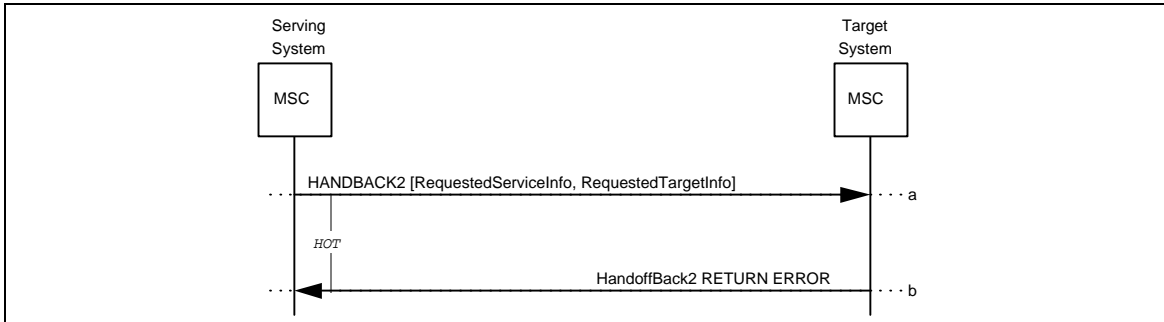
Figure 9 Unsuccessful HandoffBack2
