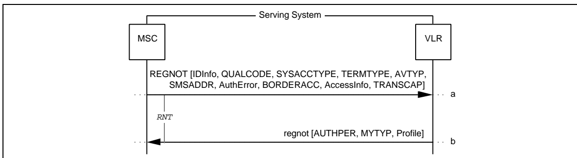
Figure 64 Successful RegistrationNotification: Confirmed at the VLR
