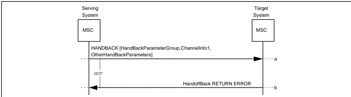
Figure 7 Unsuccessful HandoffBack
