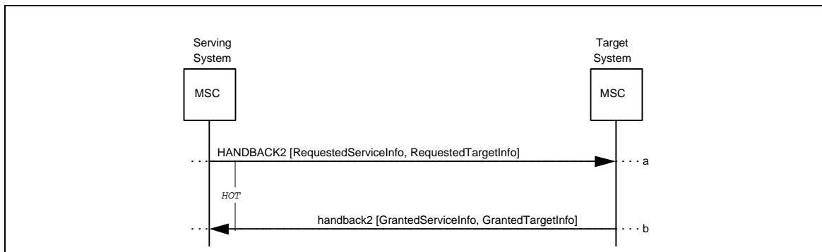
Figure 8 Successful HandoffBack2
