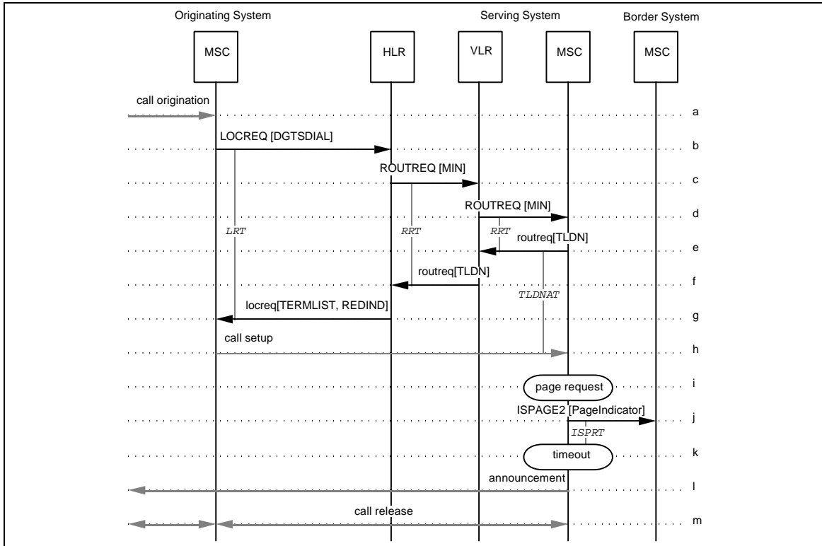
Figure 122 TLDN Call Arrival with No Page Response to Intersystem Paging
