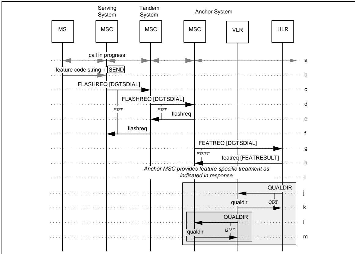
Figure 108 Feature Request After Handoff
