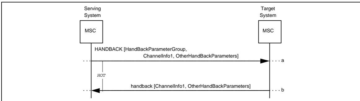
Figure 6 Successful HandoffBack
