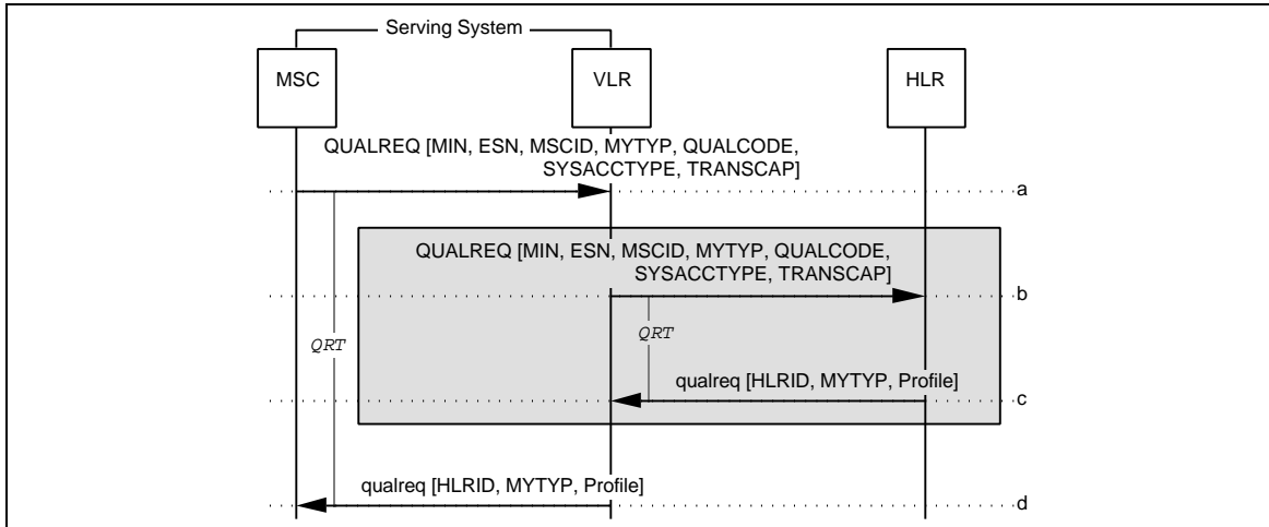
Figure 53 Successful QualificationRequest: Profile Returned Only
