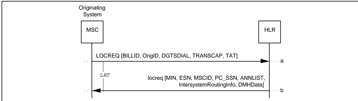
Figure 39 Successful LocationRequest: Route to an MS on Another MSC
