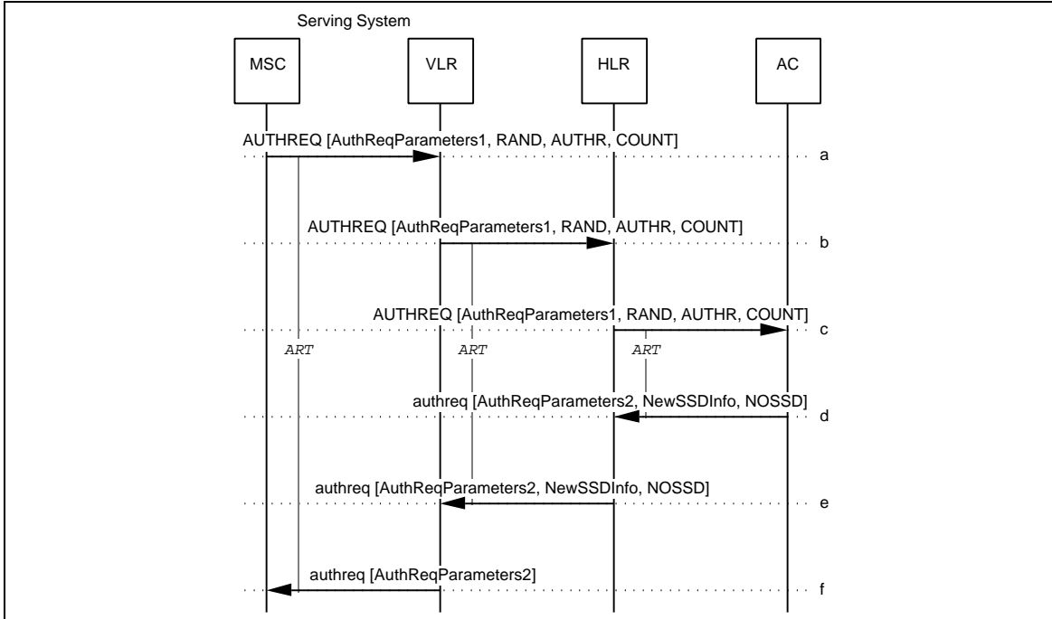
Figure 9 Successful Authentication on Initial Access
