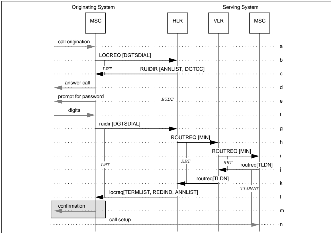
Figure 170 PCA Invocation with Call Accepted
