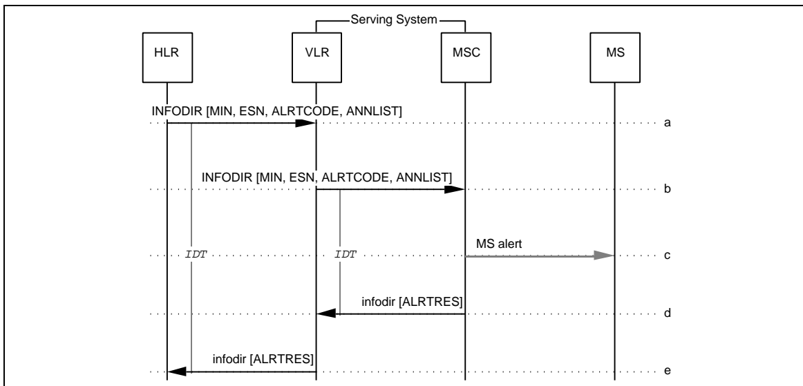
Figure 26 Successful InformationDirective
