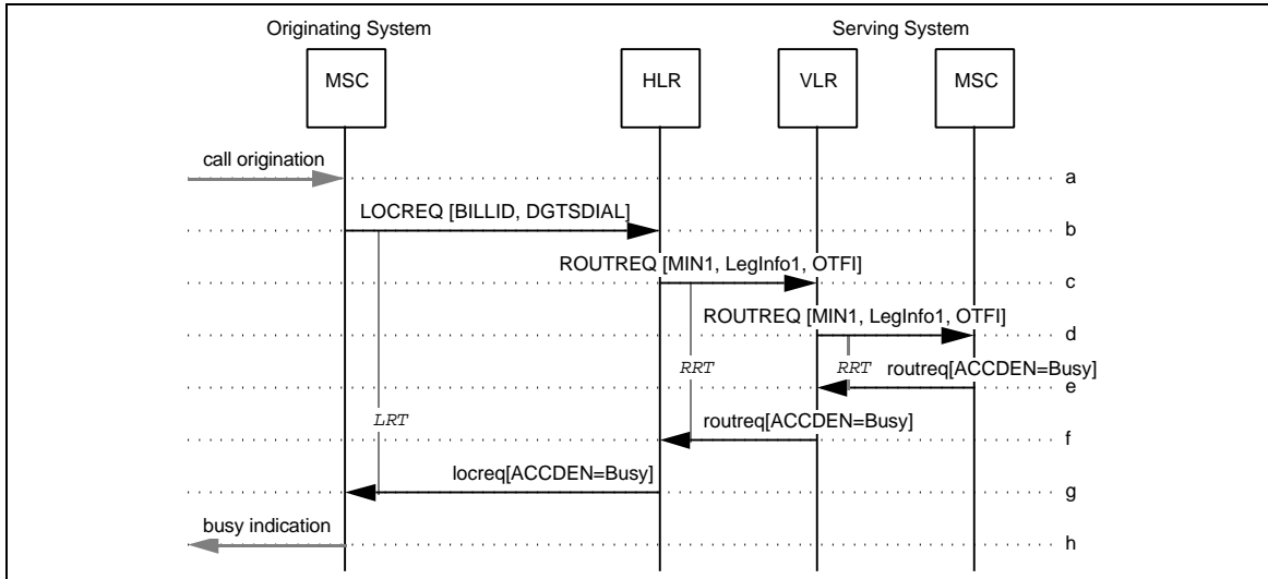
11 12 13 14 15 16 17 18 19 20 21 22 23 24 25 26 27 28 29 Figure 165 MAH Invocation with a Busy MAH Group Member 30 (Single-User Type) 31
