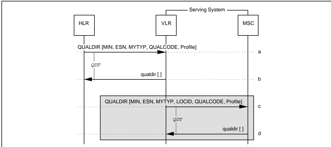
Figure 49 Successful QualificationDirective: Update Profile Only
