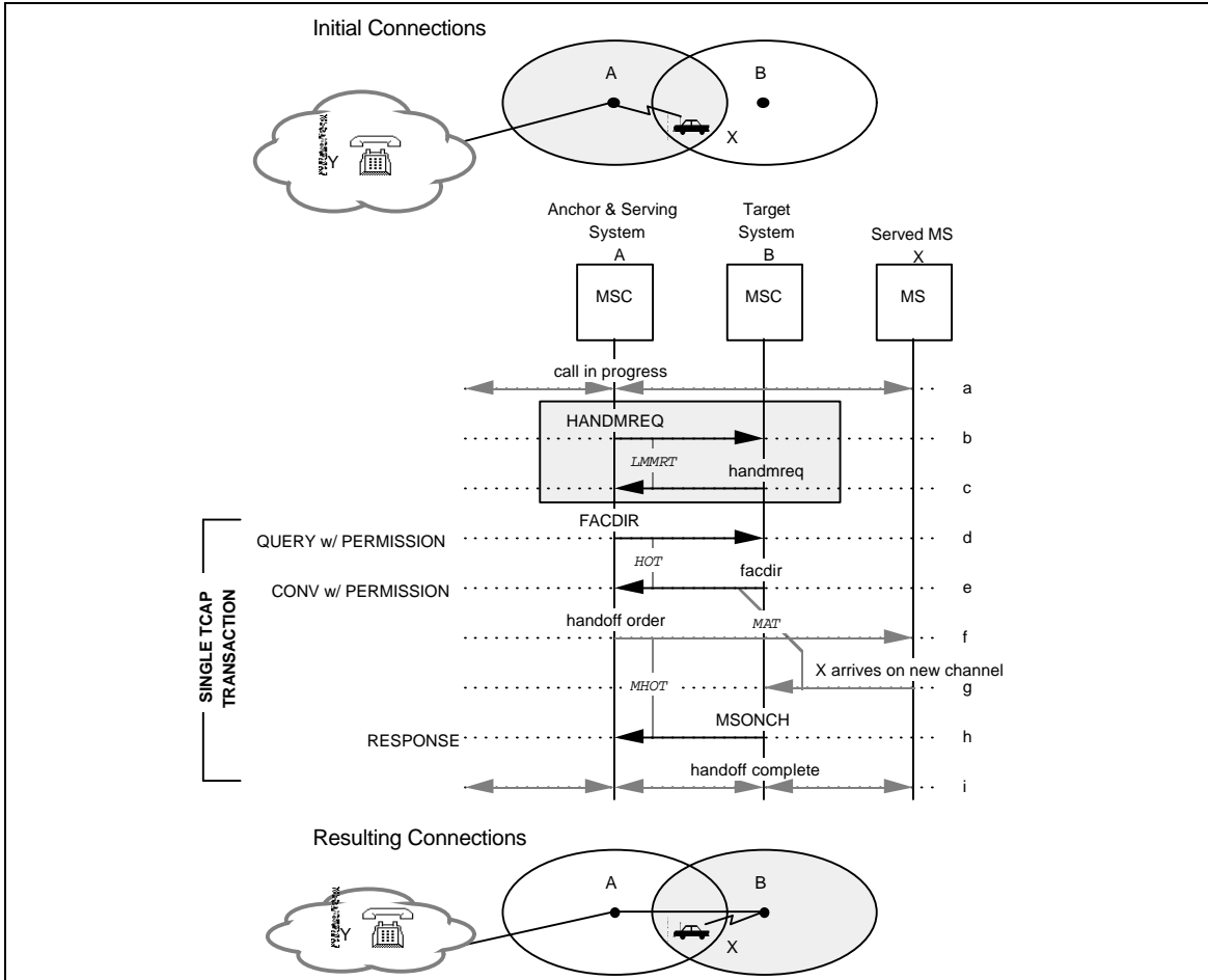
Figure 18 Successful Handoff-Forward
