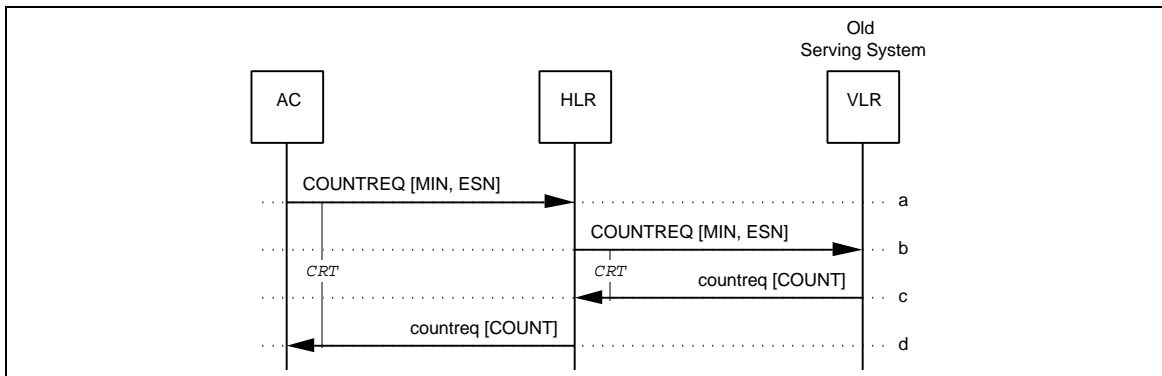
Figure 22 Successful CountRequest
