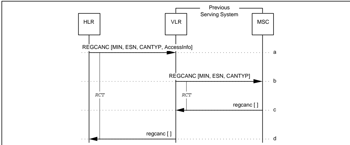
Figure 62 Successful RegistrationCancellation: Multiple Access
