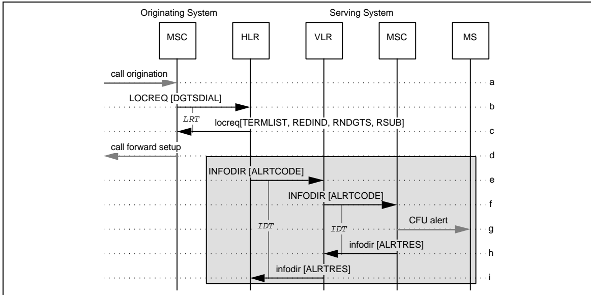
Figure 141 CNIR Interaction with CFU
