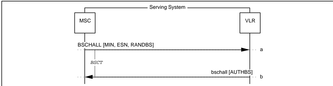
Figure 20 Base Station Challenge with SSD shared
