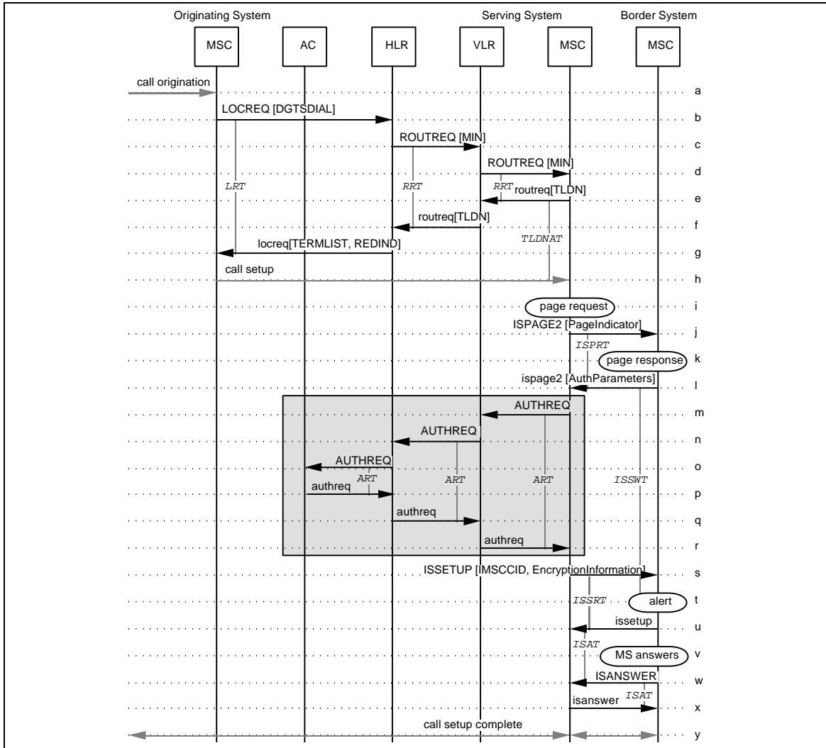
Figure 121 TLDN Call Arrival with Intersystem Paging
