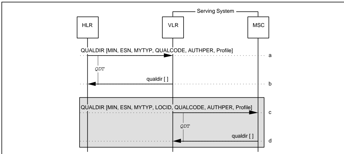
Figure 48 Successful QualificationDirective: Re-authorization and Update Profile
