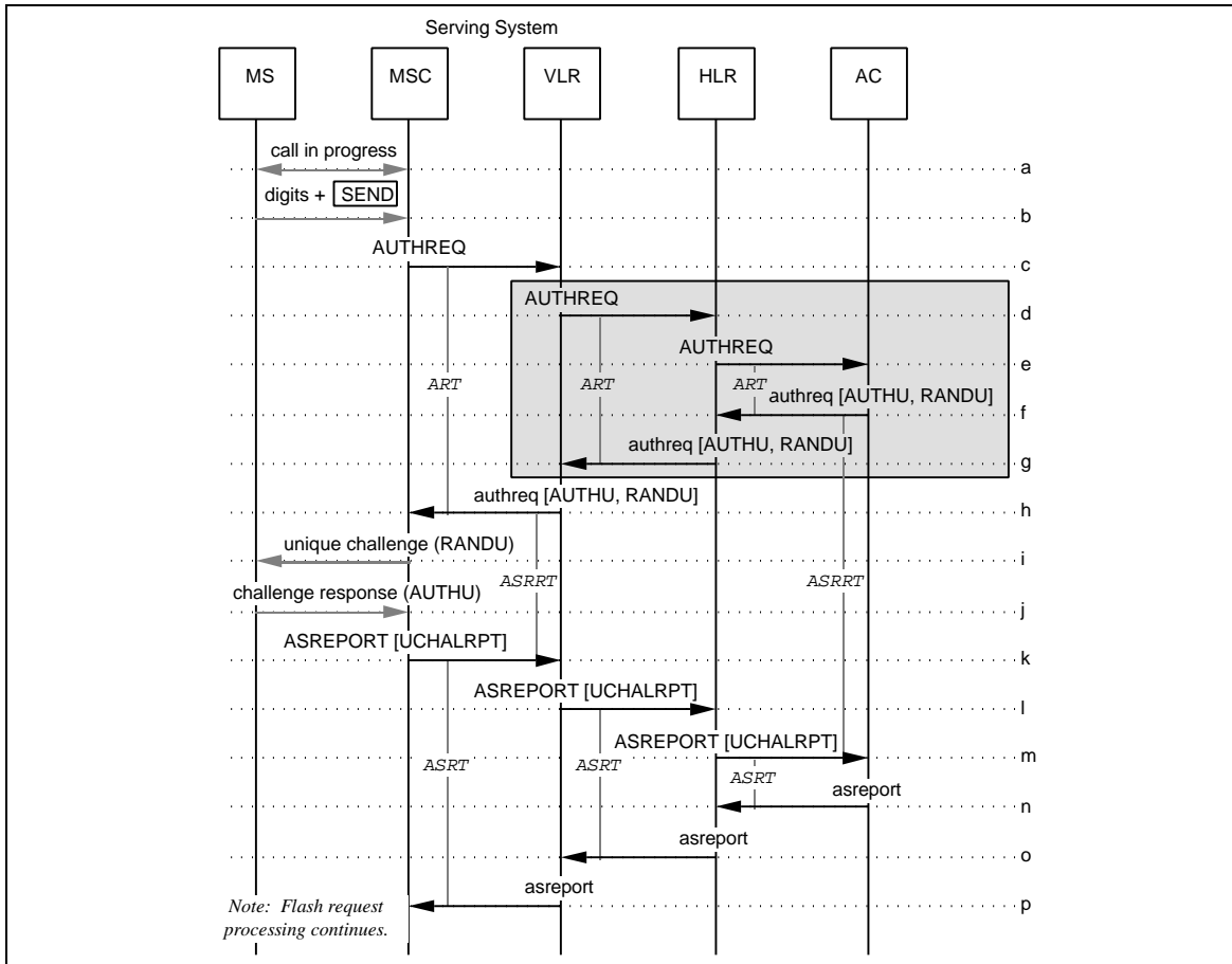
Figure 97 Authentication on Flash Request
