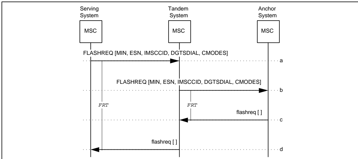
Figure 25 Successful FlashRequest
