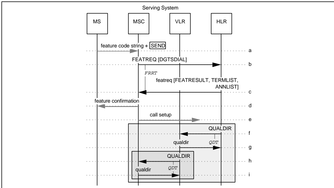
Figure 106 Feature Request Confirmation with Call Routing
