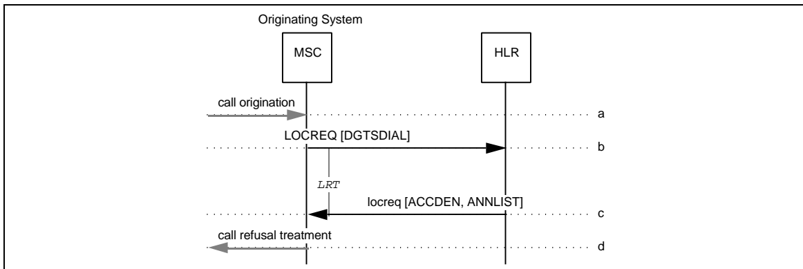
Figure 149 DND Invocation
