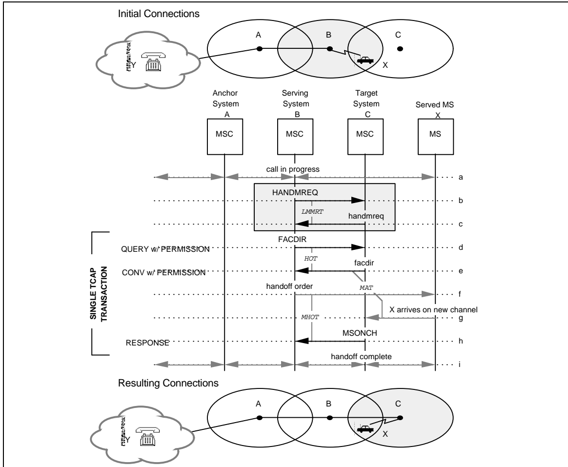
Figure 20 Successful Handoff-Forward with Tandem
