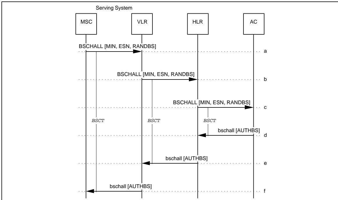
Figure 19 Base Station Challenge with SSD not shared
