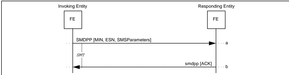
Figure 76 Successful SMSDeliveryPointToPoint
