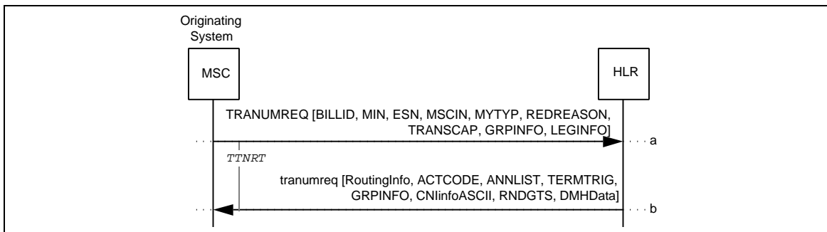
Figure 82 Successful TransferToNumberRequest
