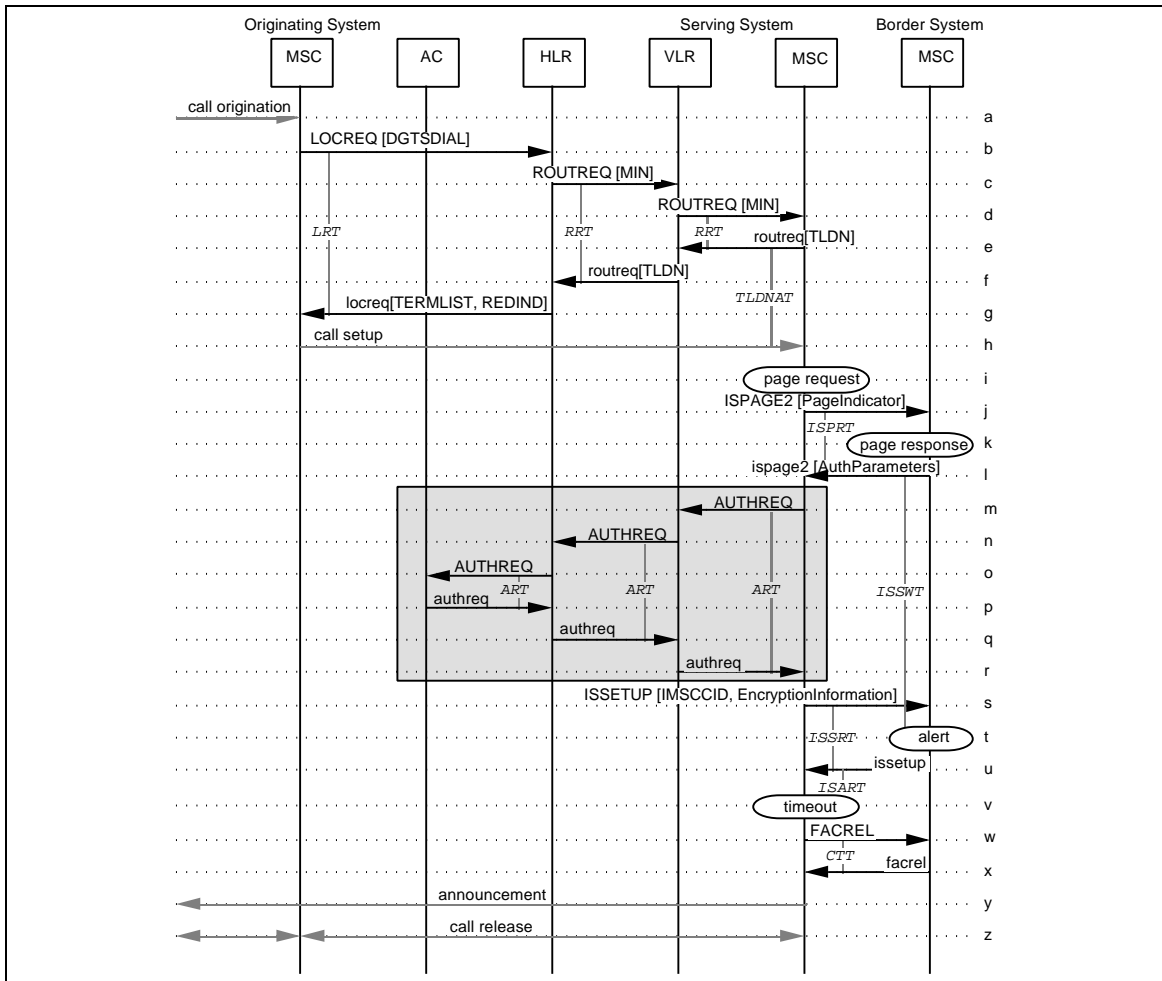
Figure 123 TLDN Call Arrival with No Answer After Paging, Call Release Initiated by Serving MSC
