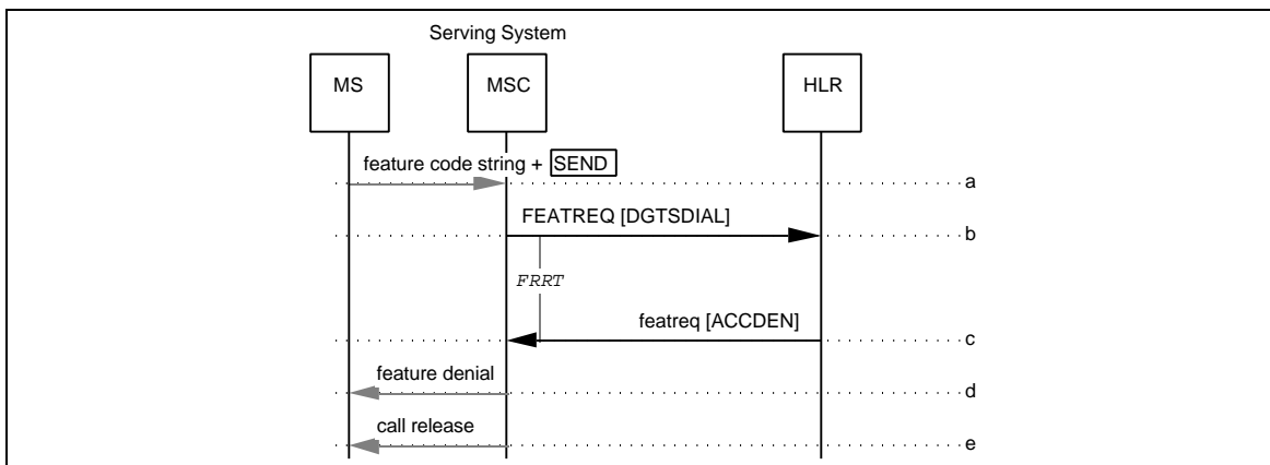
Figure 187 Feature Request with SPINA Active
