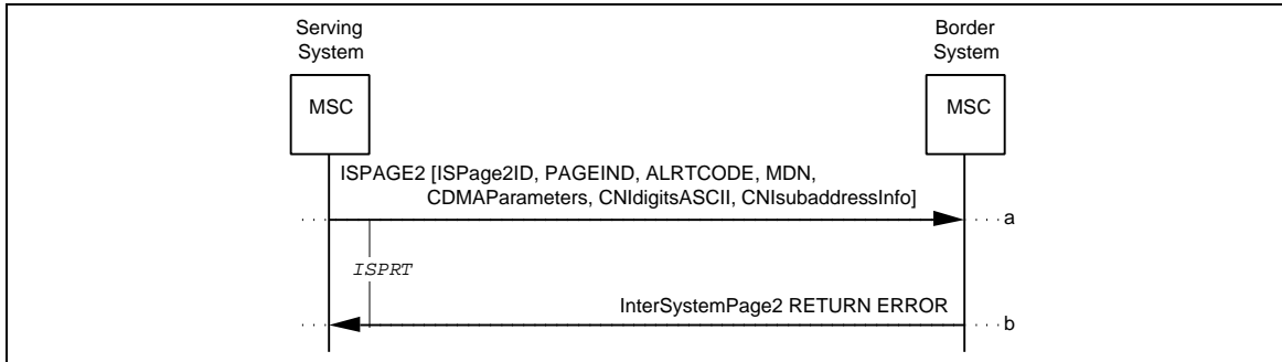
Figure 34 Unsuccessful InterSystemPage2: Resource Shortage
