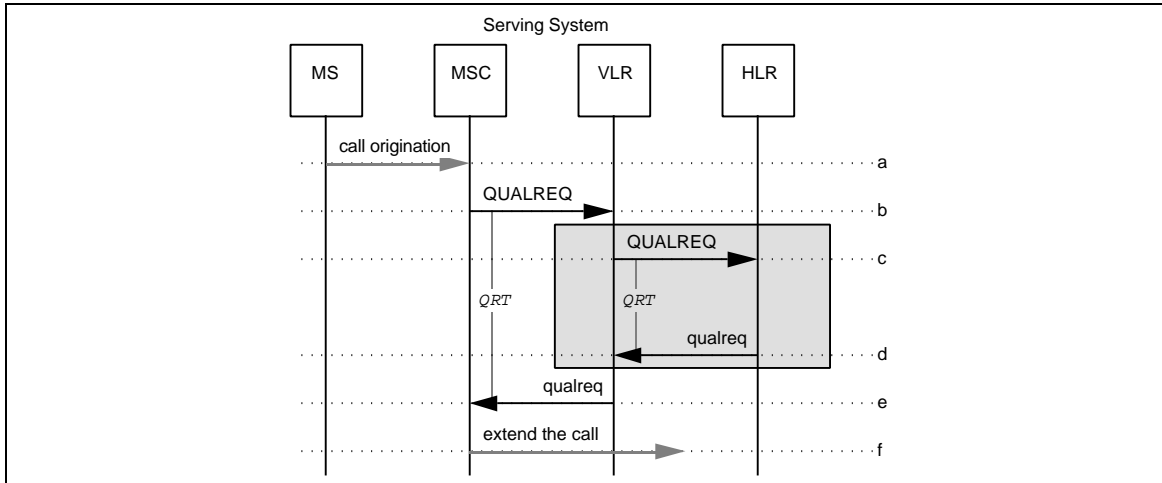
Figure 110 Call Origination without Profile
