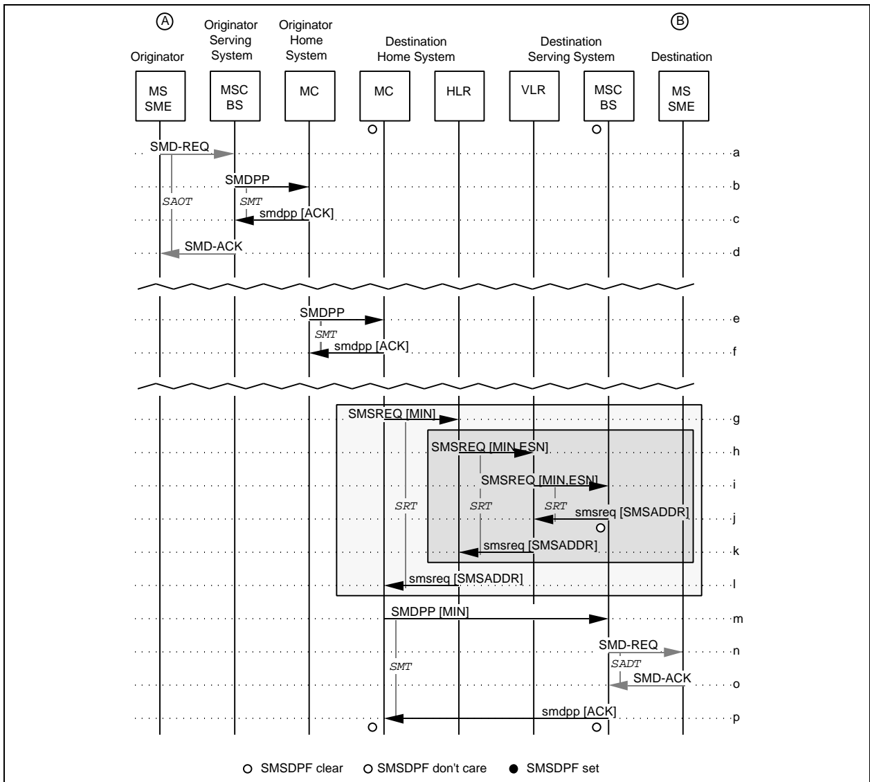
Figure 205 Short Message Between Two MS-Based SMEs with Originating SMS Supplementary Services
