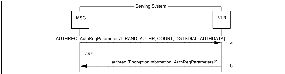
Figure 14 Successful Authentication on Call Origination (SSD shared)
