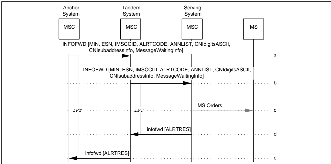
Figure 27 Successful InformationForward
