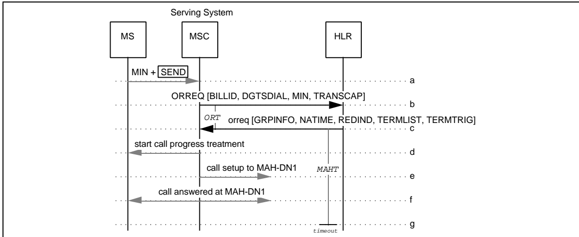
Figure 168 MAH Invocation on Revertive Call to MAH Pilot DN
