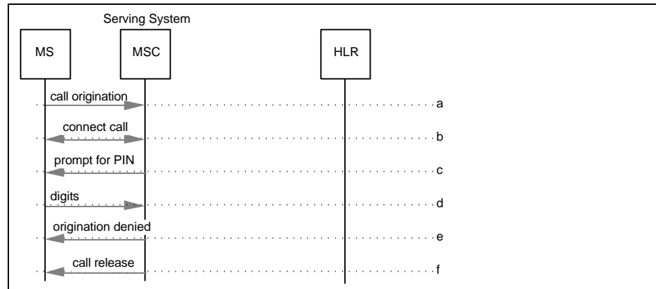
Figure 193 Unsuccessful Call Origination with Local SPINI Operation
