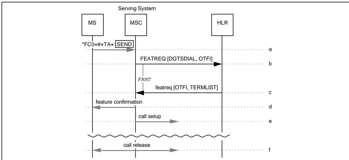
Figure 131 CW Demand Cancellation with Call
