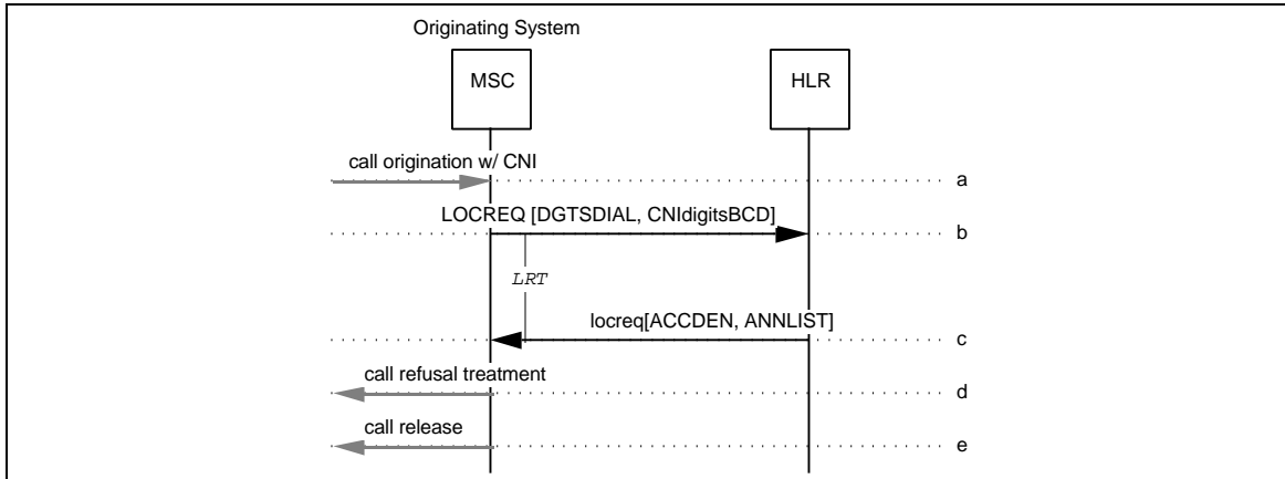
Figure 181 SCA Invocation with Call Refused to Tone or Announcement
