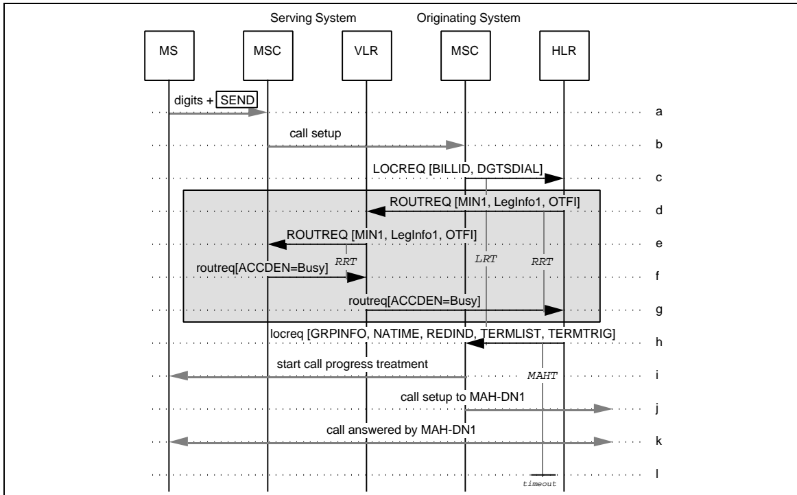
Figure 169 MAH Invocation on Call from MAH Group Member
