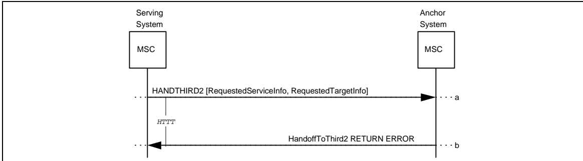
Figure 15 Unsuccessful HandoffToThird2
