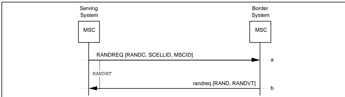
Figure 55 Successful RandomVariableRequest
