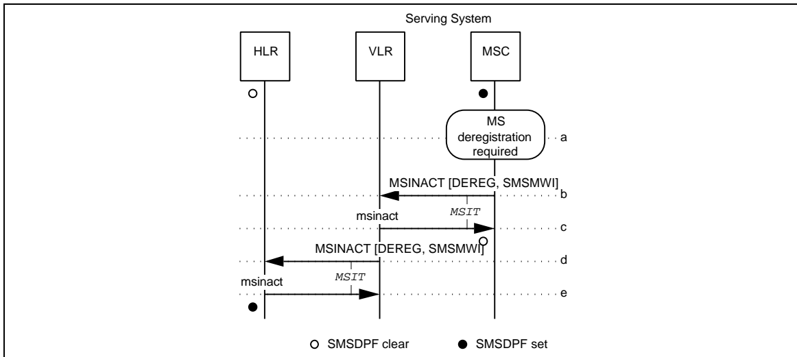
Figure 214 MSC Deregistration with Pending Postponed Delivery
