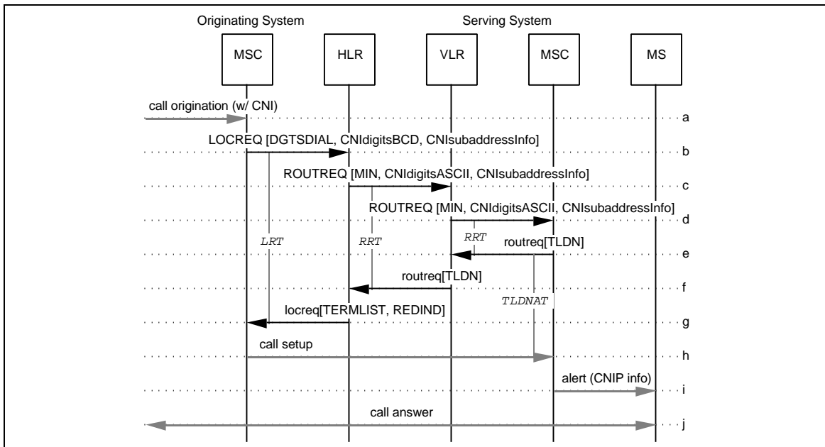
Figure 135 CNIP Invocation to an Idle Subscriber
