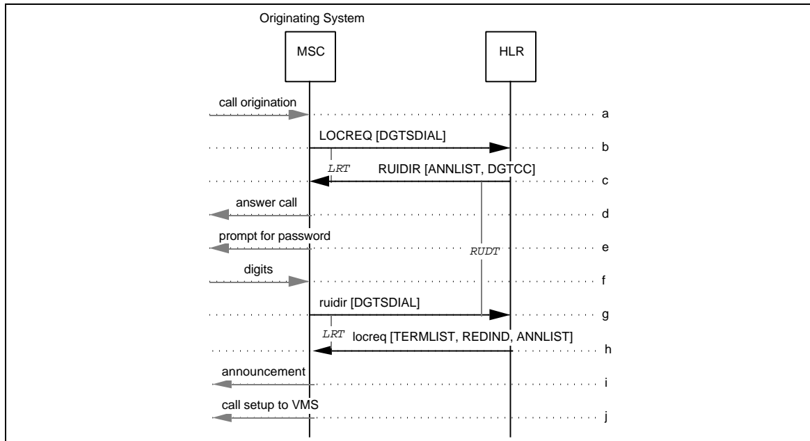
Figure 173 PCA Invocation with Call Refused to Voice Mail
