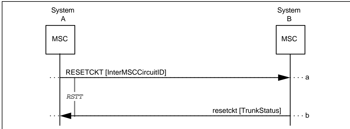
Figure 3 Normal Operation (ResetCircuit)
