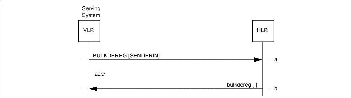
Figure 21 Successful BulkDeregistration
