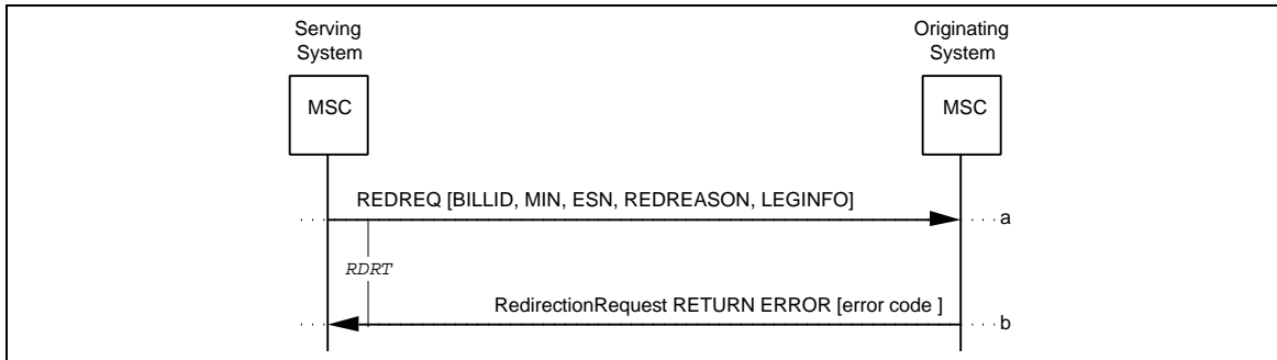
Figure 60 Unsuccessful RedirectionRequest
