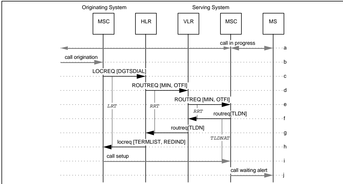
Figure 133 CW Invocation
