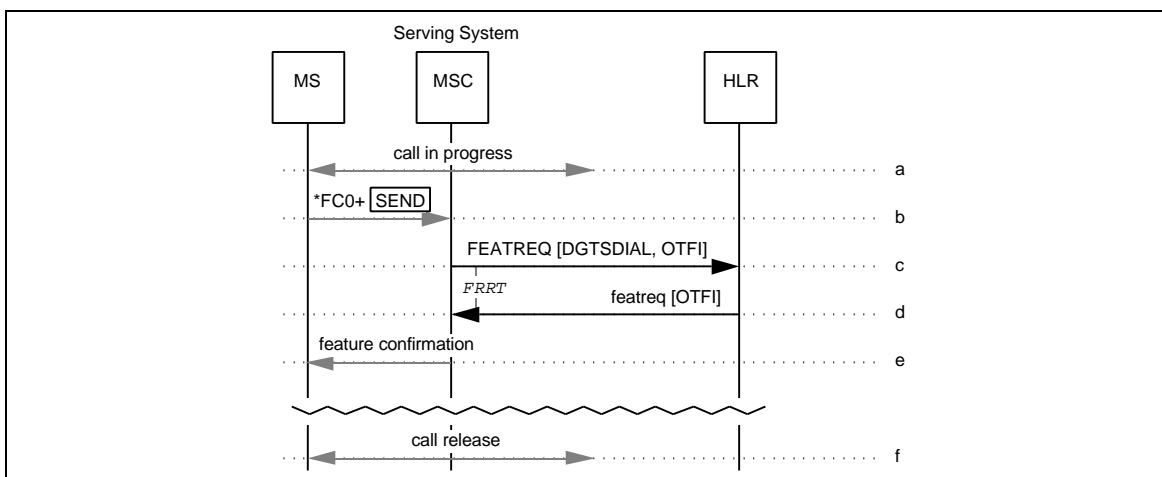
Figure 132 CW Demand Cancellation (during call)
