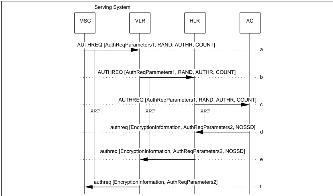
Figure 12 Successful Authentication on Call Termination (SSD not shared)
