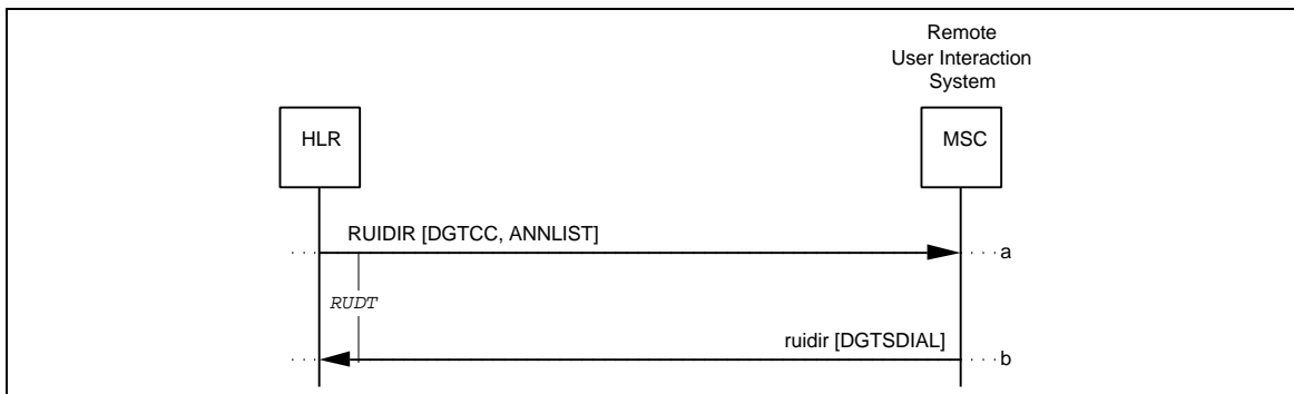
Figure 67 Successful RemoteUserInteractionDirective
