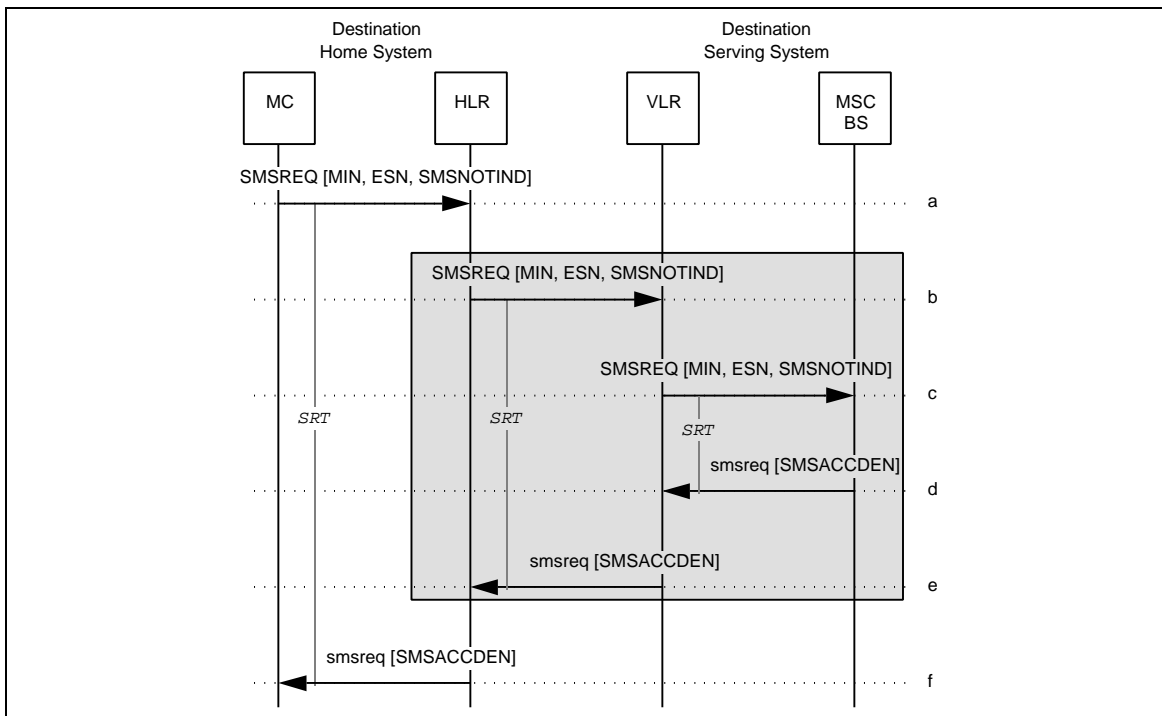
Figure 81 Unsuccessful SMSRequest: MS-Based SME Address Request
