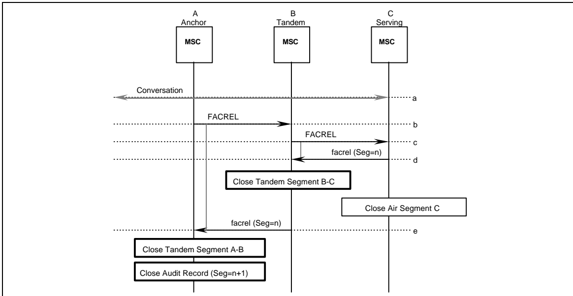
Figure A.7 Release by the other party (A-B-C)
