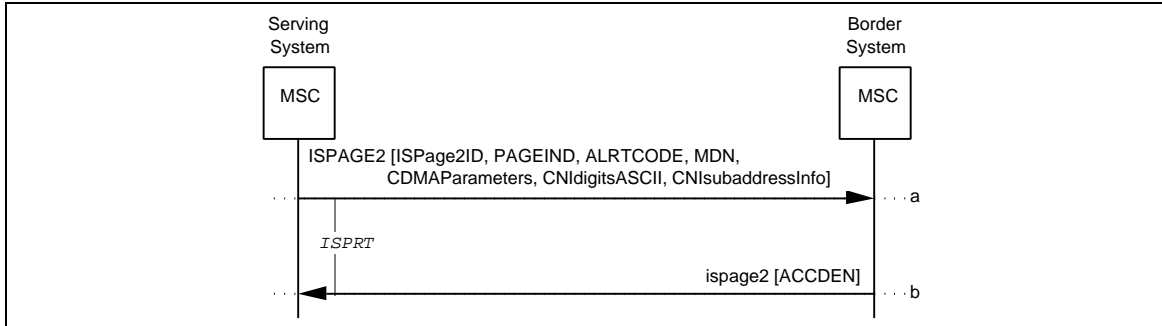
Figure 33 Unsuccessful InterSystemPage2: Access Denied
