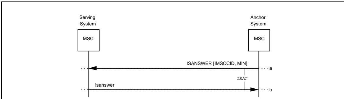
Figure 16 Successful InterSystemAnswer Following the Handoff of an Originating MS Awaiting Answer
