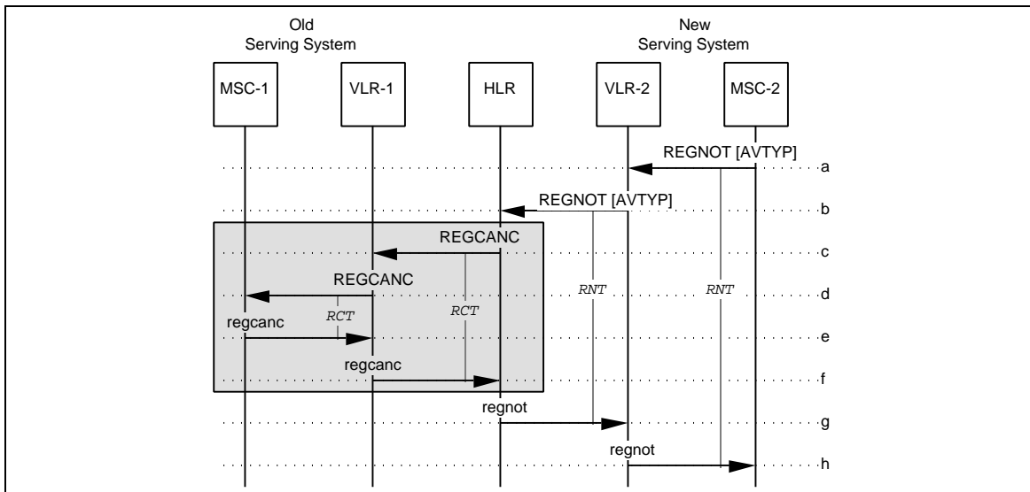
Figure 92 MS Declared Inactive by Serving MSC at Registration
