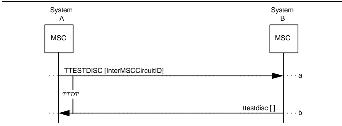
Figure 5 Normal Operation (TrunkTestDisconnect)
