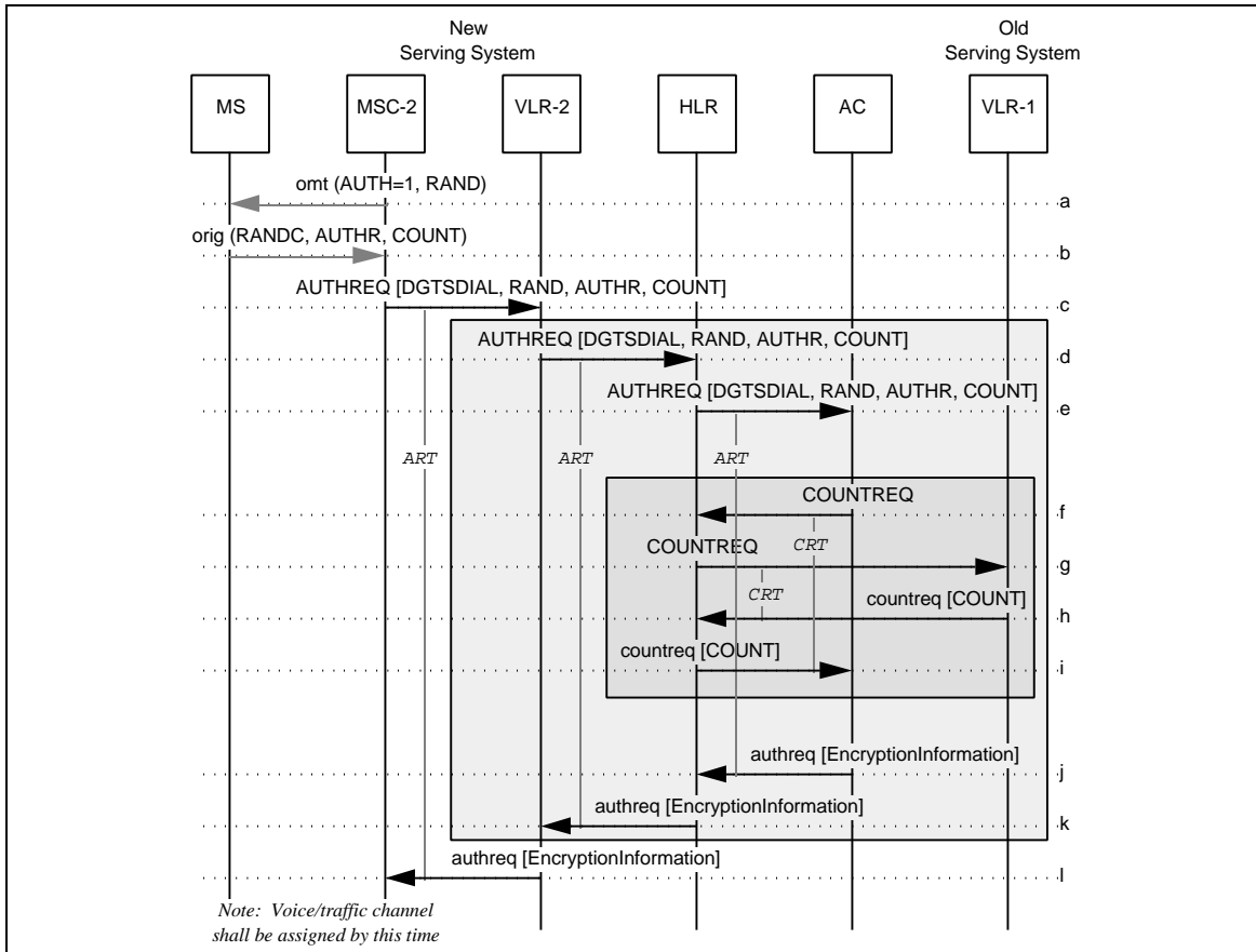
Figure 94 Origination with Authentication
