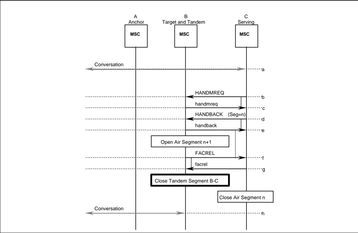
Figure A.4 Handoff-Back (C to B)
