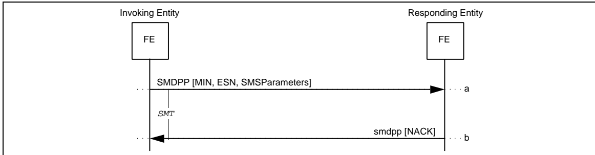
Figure 77 Unsuccessful SMSDeliveryPointToPoint
