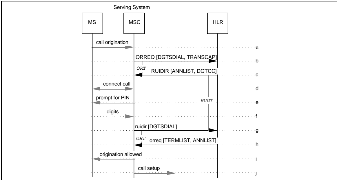
Figure 189 Call Origination with SPINI Active and Correct PIN Entered
