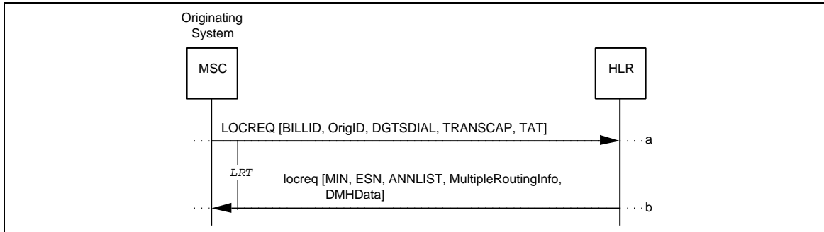
Figure 41 Successful LocationRequest: Route to Multiple Terminations
