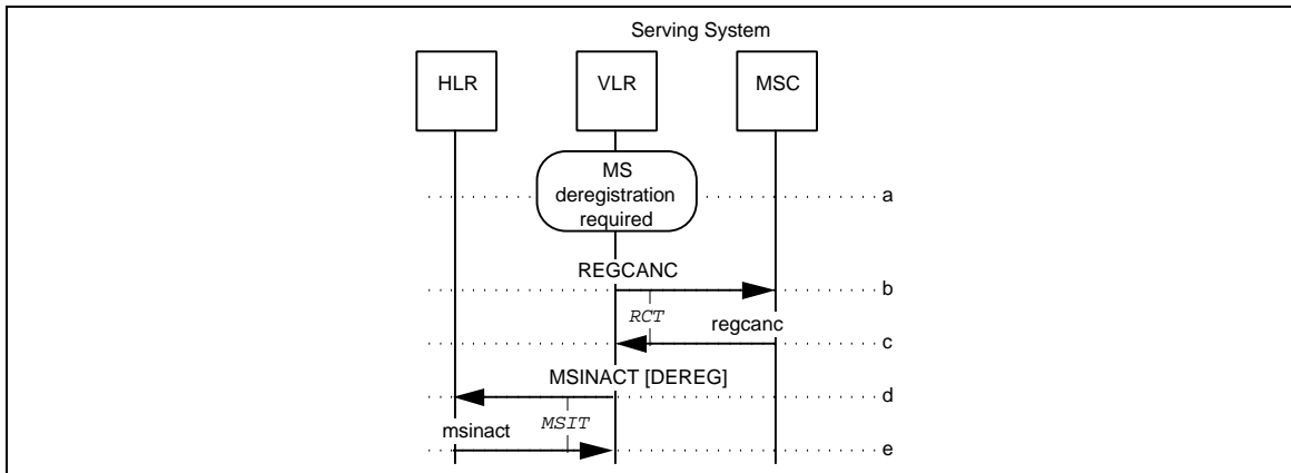
Figure 90 MS Deregistered by Serving VLR
