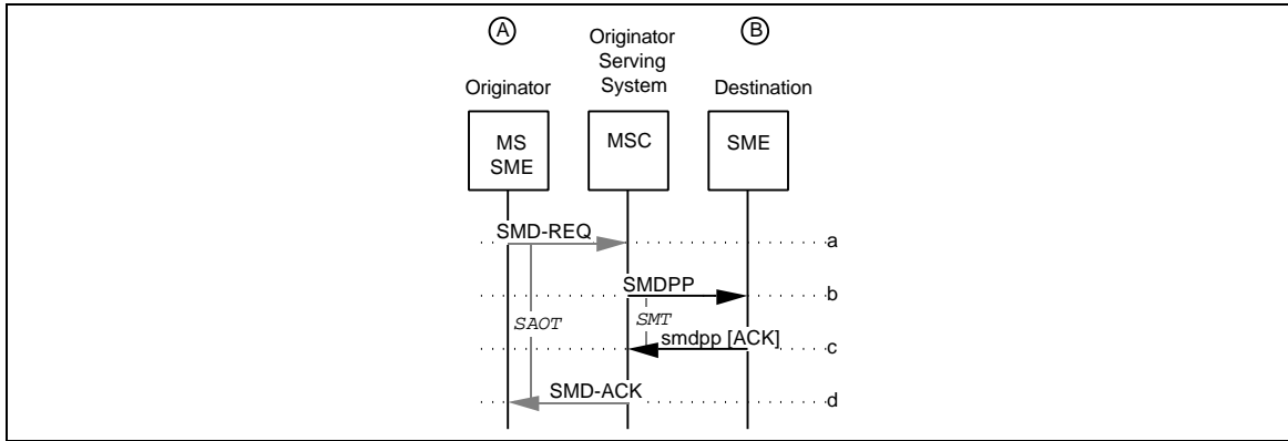
Figure 202 Short Message from an MS-Based SME to a Fixed SME
