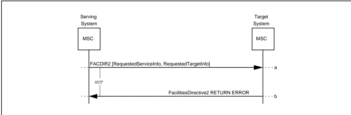
Figure 4 Unsuccessful FacilitiesDirective2
