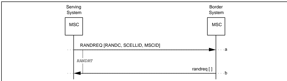
Figure 56 Unsuccessful RandomVariableRequest
