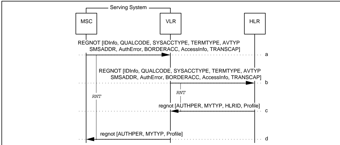
Figure 65 Successful RegistrationNotification: Confirmed at the HLR
