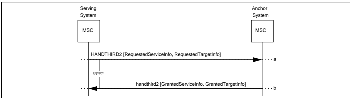
Figure 14 Successful HandoffToThird2
