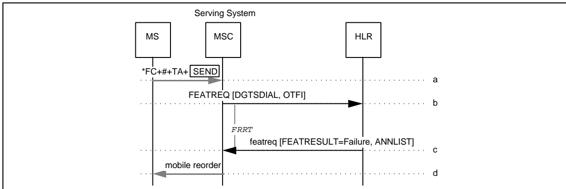
Figure 178 Unsuccessful PACA Activation with Call
