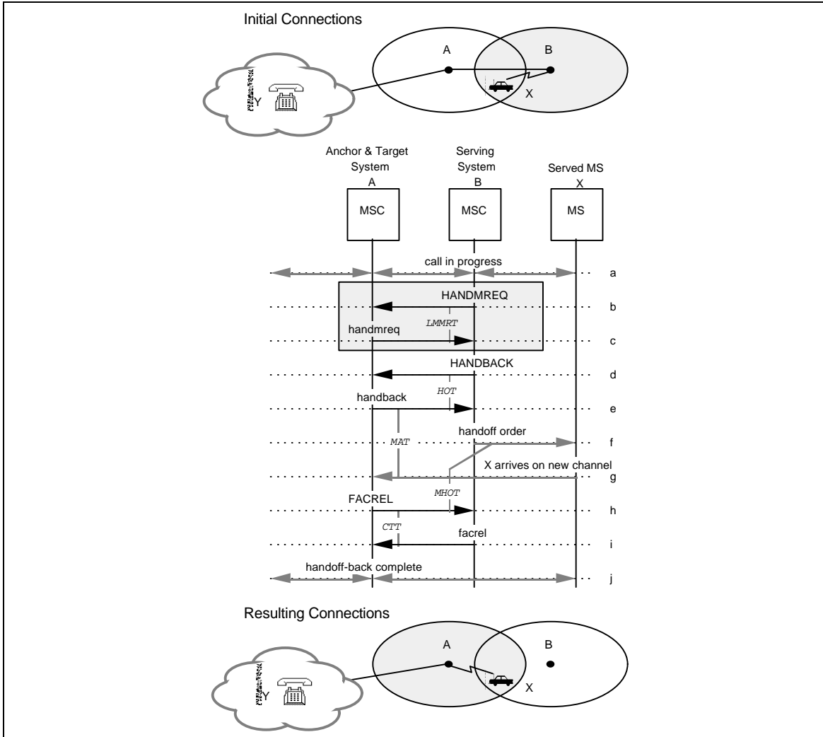
Figure 19 Successful Handoff-Back
