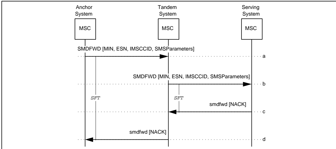
Figure 75 Unsuccessful SMSDeliveryForward
